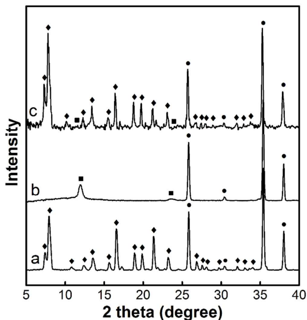
Fig. 3 XRD patterns of (a) ZIF-7 films prepared on bare \alpha -Al 2 O 3 substrates by in situ solvothermal growth; and (b) Co-Al HTlc buffer layers in situ grown on \alpha -Al 2 O 3 substrates; and (c) ZIF-7 films prepared on Co-Al HTlc buffer layer-modified \alpha -Al 2 O 3 substrates by in situ solvothermal growth. Peaks marked with rhombuses, squares and dots represent diffraction peaks from the ZIF-7 film, Co-Al HTlc buffer layer and \alpha -Al 2 O 3 substrate, respectively.
