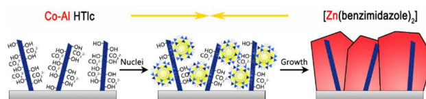
Fig. 1 Schematic illustration of in situ solvothermal synthesis of qualified ZIF-7 films on Co-Al HTlc buffer layer-modified \alpha -Al 2 O 3 substrates.
