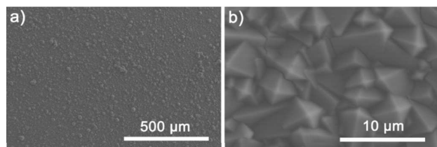
Fig. 6 (a, b) SEM images of the ZIF-7 film after ultrasonic treatment in methanol solvent for 30 min. Note: Cracks in figure (b) were spontaneously generated during the SEM observation.
