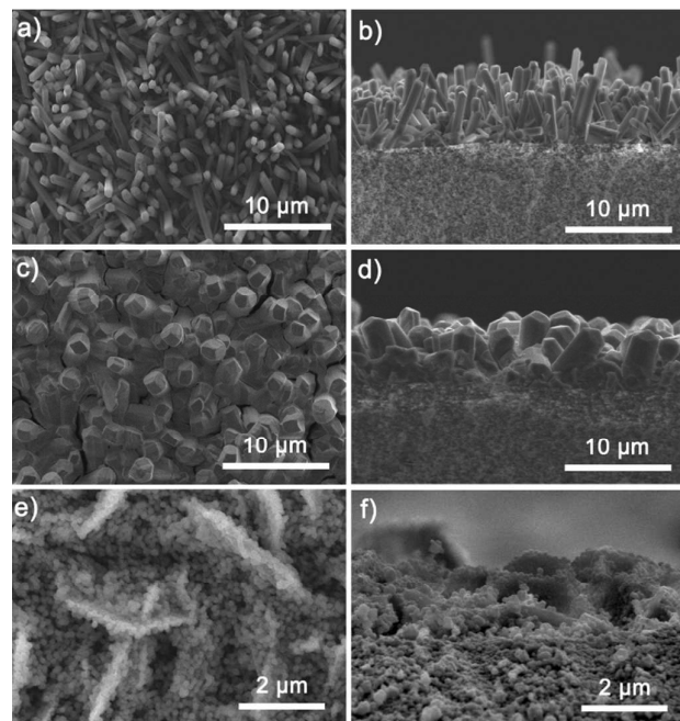
Fig. 4 SEM images of ZIF-7 films prepared on Co-Al HTlc buffer layer-modified \alpha\text{-Al}_2\text{O}_3 substrates by in situ solvothermal growth with (a, b) \text{ZnCl}_2 , (c, d) \text{ZnBr}_2 and (e, f) \text{ZnI}_2 as zinc sources, respectively.
