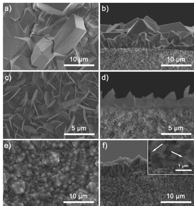
Fig. 2 SEM images of (a, b) ZIF-7 films prepared on bare \alpha -Al 2 O 3 substrates by in situ solvothermal growth; and (c, d) Co-Al HTlc buffer layers in situ grown on \alpha -Al 2 O 3 substrates; (e, f) ZIF-7 films prepared on Co-Al HTlc buffer layer-modified \alpha -Al 2 O 3 substrates by in situ solvothermal growth. Inset: Enlarged cross-sectional SEM image at the ZIF-7 film-substrate interface. White arrows: Co-Al HTlc crystals.
