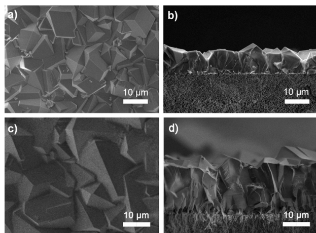
Fig. 7 SEM images of (a, b) ZIF-8 films prepared on Co-Al HTlc buffer layer-modified \alpha -Al 2 O 3 substrates by in situ solvothermal growth; (c, d) ZIF-8 films prepared on Mg-Al HTlc buffer layer-modified \alpha -Al 2 O 3 substrates by in situ solvothermal growth.
