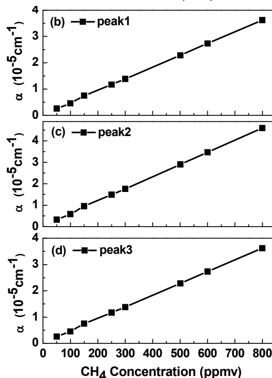
Fig. 8 (a) Measured absorption spectra of \text{CH}_4 with different concentration levels in the fitting range. Relationships between the maximum absorption coefficient of (b) peak1, (c) peak2, (d) peak3 and different \text{CH}_4 concentration levels, respectively.
