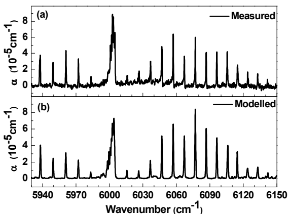
Fig. 7 (a) P, Q, R-branch of the 2\nu_3 overtone of \text{CH}_4 measured in ambient air at atmospheric pressure using the FT-IBCEAS. Measurement time: 20 min; Resolution: 0.5 \text{ cm}^{-1} . (b) Modelled least-square fit spectrum in the same region using the HITRAN database.
