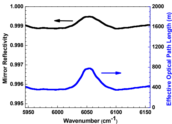
Fig. 6 Curves of the mirror reflectivity and the effective optical path length of the cavity versus wavenumber.
