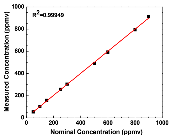
Fig. 9 Correlation plot of the \text{CH}_4 concentration measured by the sensor system and the nominal concentration generated by the standard gas mixing system.
