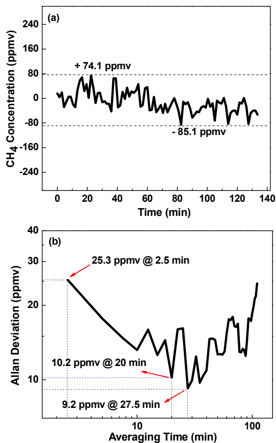
Fig. 10 (a) Time series of the measurement results of the \text{CH}_4 sample with zero concentration. (b) Allan variance analysis of the FT-IBBCEAS \text{CH}_4 sensor system.
