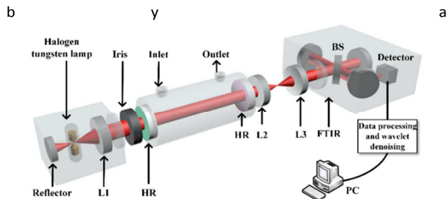
Fig. 4 Schematic of the experimental set-up. L1 is a plano-convex lens used to collimate the light from the tungsten-halogen lamp. HR is a highly-reflective mirror used to form an optical cavity and a gas cell. L2 and L3 are achromatic lenses used to focus and collimate the light leaking through the cavity. FTIR is a Fourier-transform infrared spectrometer. BS is a beam splitter. A PC is used for data processing and wavelet denoising.
