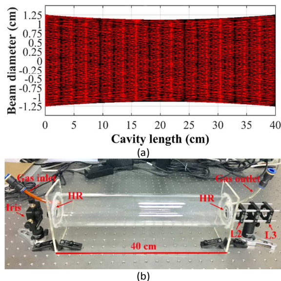
Fig. 3 (a) Simulated light beam propagation between two cavity mirrors with optimized parameters. (b) Photograph of the fabricated cavity with a length of 40 cm and a volume of 1 L.
