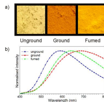
Fig. 11 a) Photographs showing the luminescence colour changes of complex 1 upon mechanical grinding and subsequent solvent treatment and b) the corresponding emission spectra.
