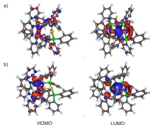
Fig. 8 Contour plots of the HOMO and LUMO superimposed on the a) singlet ground ( S_0 ) and b) triplet excited ( T_1 ) state geometry of [\text{Au}_2(\text{dpephos})_2]^{2+} .
