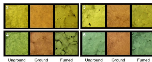
Fig. 9 Optical images taken under 365 \text{ nm} UV lamp illumination showing the reversible mechanochromic luminescence of complexes 2–5 upon grinding and exposure to solvent vapours.
