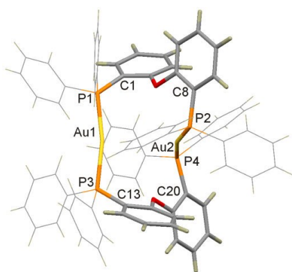
Fig. 1 Cationic [\text{Au}_2(\text{dpephos})_2]^{2+} skeleton in complexes 1–5. Colour scheme: gold, yellow; phosphorous, orange; carbon, grey; oxygen, red; hydrogen, dark brown. The phenyl groups are shown as a wireframe model.
