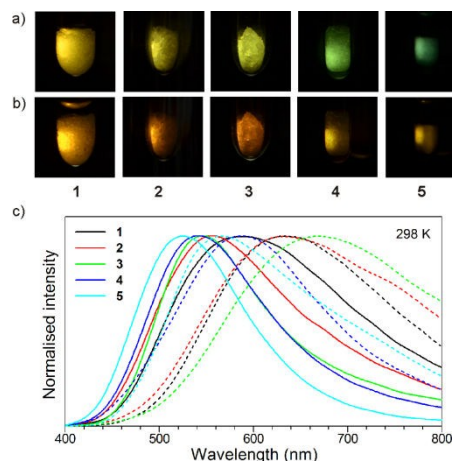
Fig. 4 Optical images of crystals of 1–5 taken under 365 nm (a) and 312 nm (b) UV lamp and (c) excitation wavelength-dependent emission spectra of crystals of 1–5 at 298 K ( \lambda_{\text{ex}} = 365 nm, solid lines; \lambda_{\text{ex}} = 312 nm, dashed lines).
