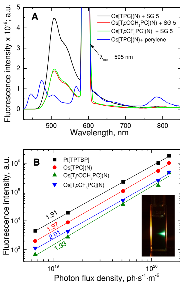
Figure 4. Panel A: Emission spectra of anoxic toluene solutions containing 1 \cdot 10^{-4} M of an \text{Os}^{\text{VI}}\text{N} corrole and 2.5 \cdot 10^{-4} M of annihilator ( \lambda_{exc} 595 nm). Panel B: Dependence of the intensity of upconverted fluorescence ( \lambda = 505 nm) on the power density of the excitation light with slopes of the curve indicated. The insert shows a photographic image of anoxic toluene solution containing 1 \cdot 10^{-4} M of \text{Os}^{\text{VI}}[\text{TPC}](\text{N}) and 2.5 \cdot 10^{-4} M of annihilator SG 5 under excitation with a 590-nm LED.
