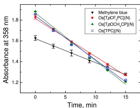
Figure 5. Degradation profiles of 9,10-dimethylanthracene (7 \mu M) in an air-saturated solution (9:1 EtOH/THF) in presence of a sensitizer ( \sim 15 \mu M) upon excitation with orange light (595 \pm 5 nm; photon flux \sim 175 \mu mol \cdot s -1 \cdot m -2 ). Absorption spectra for all the systems are provided in ESI (Fig. S4-S7).
