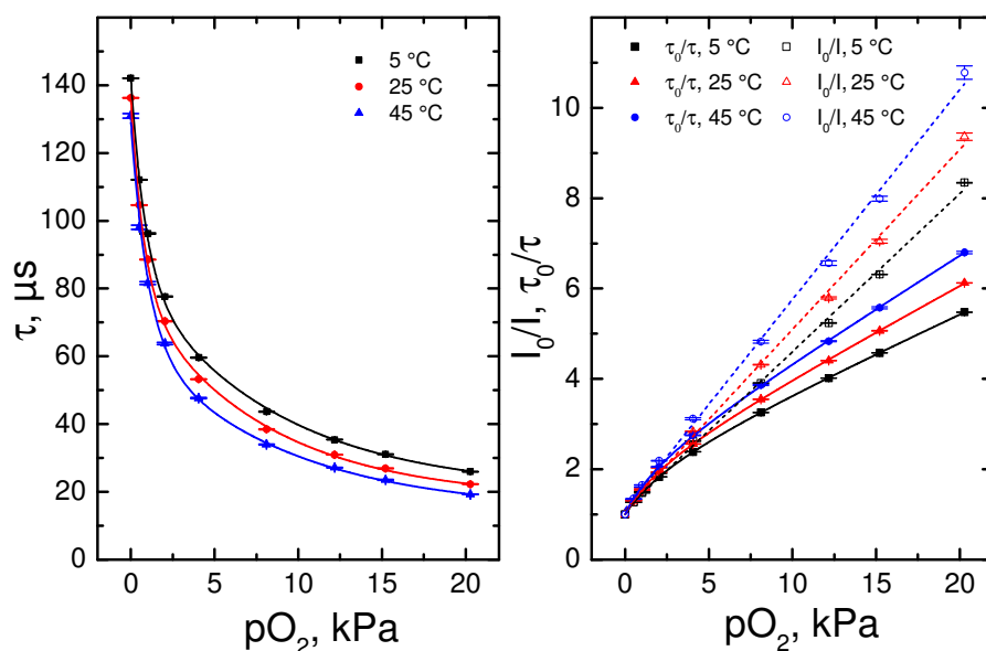
Figure 2. Decay time (left) and Stern-Volmer plots (right) for the oxygen sensor based on Os[TpOCH 3 PC](N) in polystyrene. Eq. 1 was used to fit the decay time Stern-Volmer plots, whereas a linear fit was used in case of the intensity plots.
