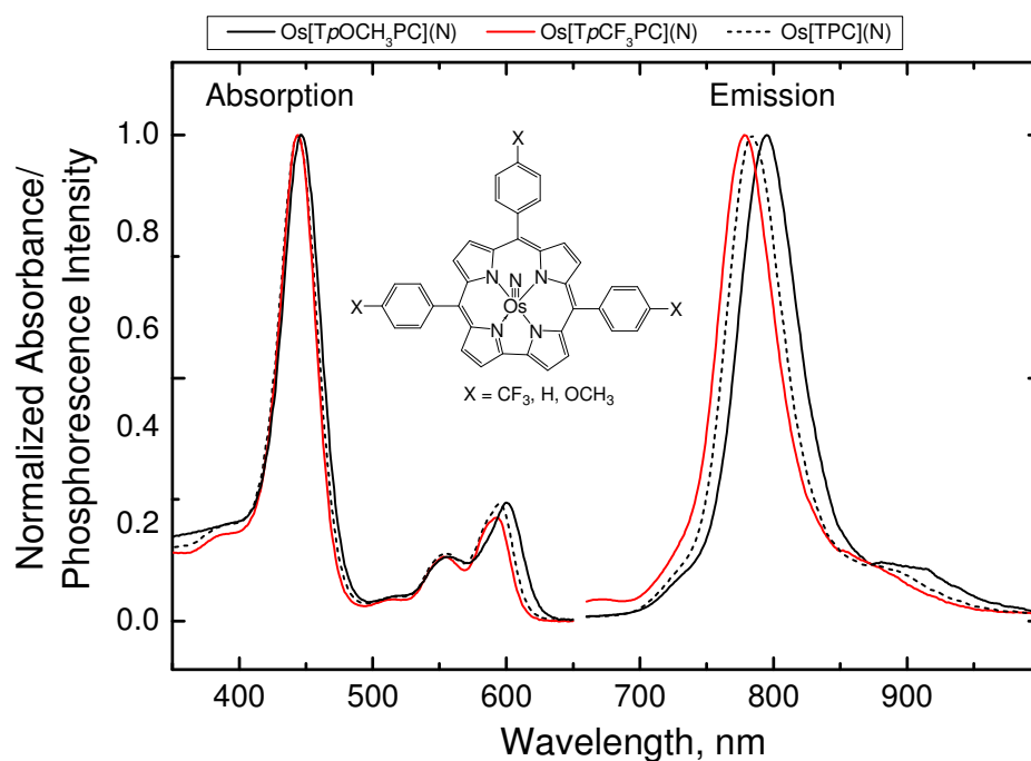
Figure 1. Absorption and emission spectra of Os VI N corroles in toluene (25 °C, \lambda_{\text{ex}} 595 nm).
