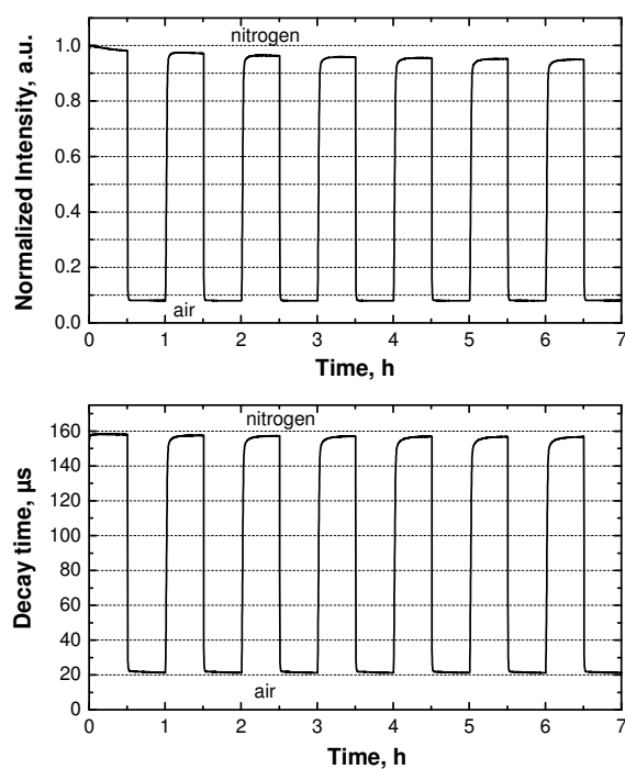
Figure 3. Intensity (above) and decay time (below) profiles for the oxygen sensor based on \text{Os}[\text{TpOCH}_3\text{PC}](\text{N}) in polystyrene upon continuous excitation with a 455-nm LED (25 °C).
