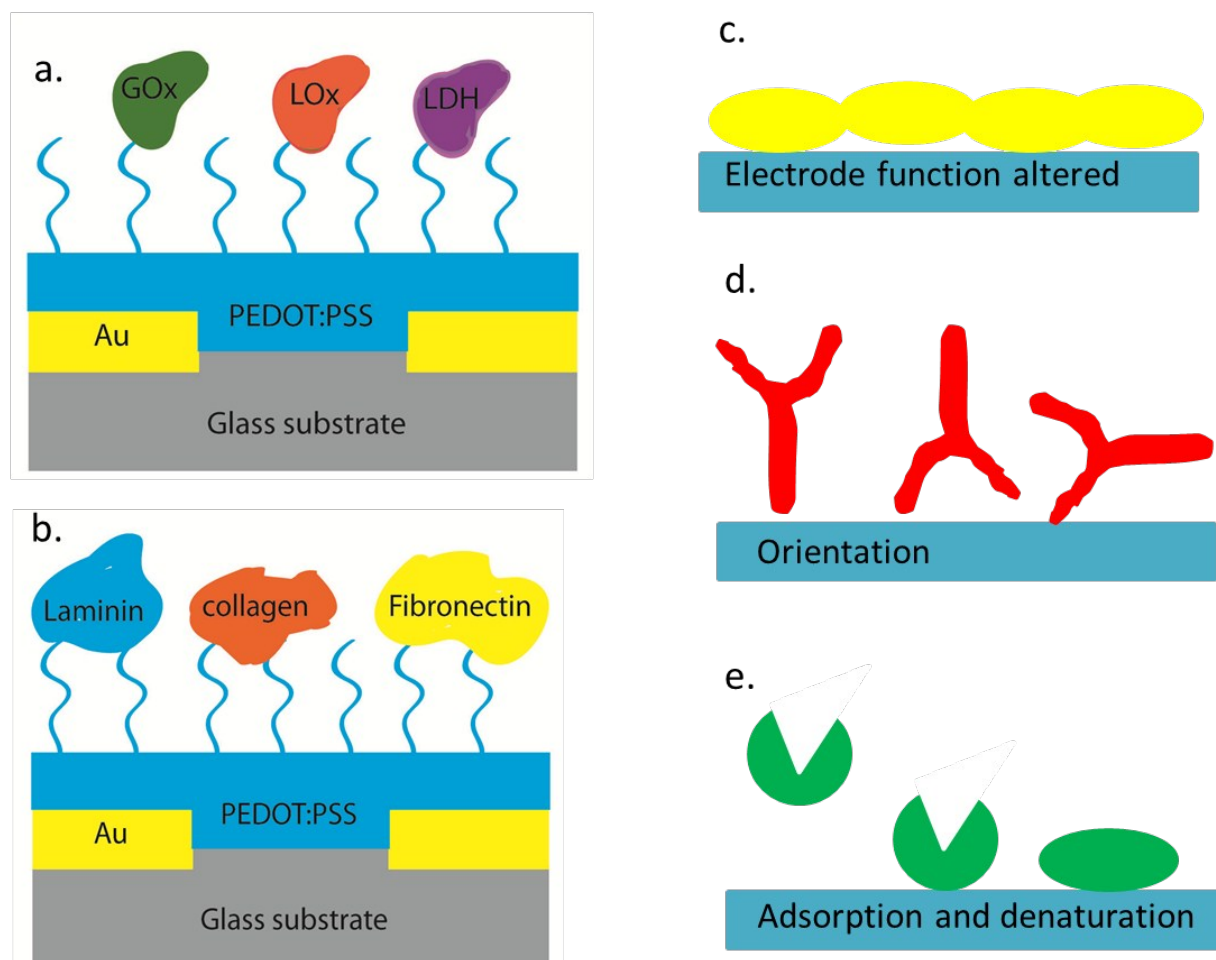
Figure 3. Biofunctionalisation strategies of polydioxythiophene electrodes for either (a) biosensing (GOx: glucose oxidase; LOx: Lactate oxidase; LDH: Lactate dehydrogenase) or (b) biocompatibility (c) Biomolecules adsorbed onto active surfaces can result in loss or change of function for example through impedance of ion flow. (d) Orientation of the protein molecules is important. For antibodies, the antigen binding region (designated by the arms of the Y) should be oriented away from the surface. Other orientations result in non-functional antibodies. (e) Adsorption of molecules such as enzymes can result in loss of conformation and inaccessibility of active site.
