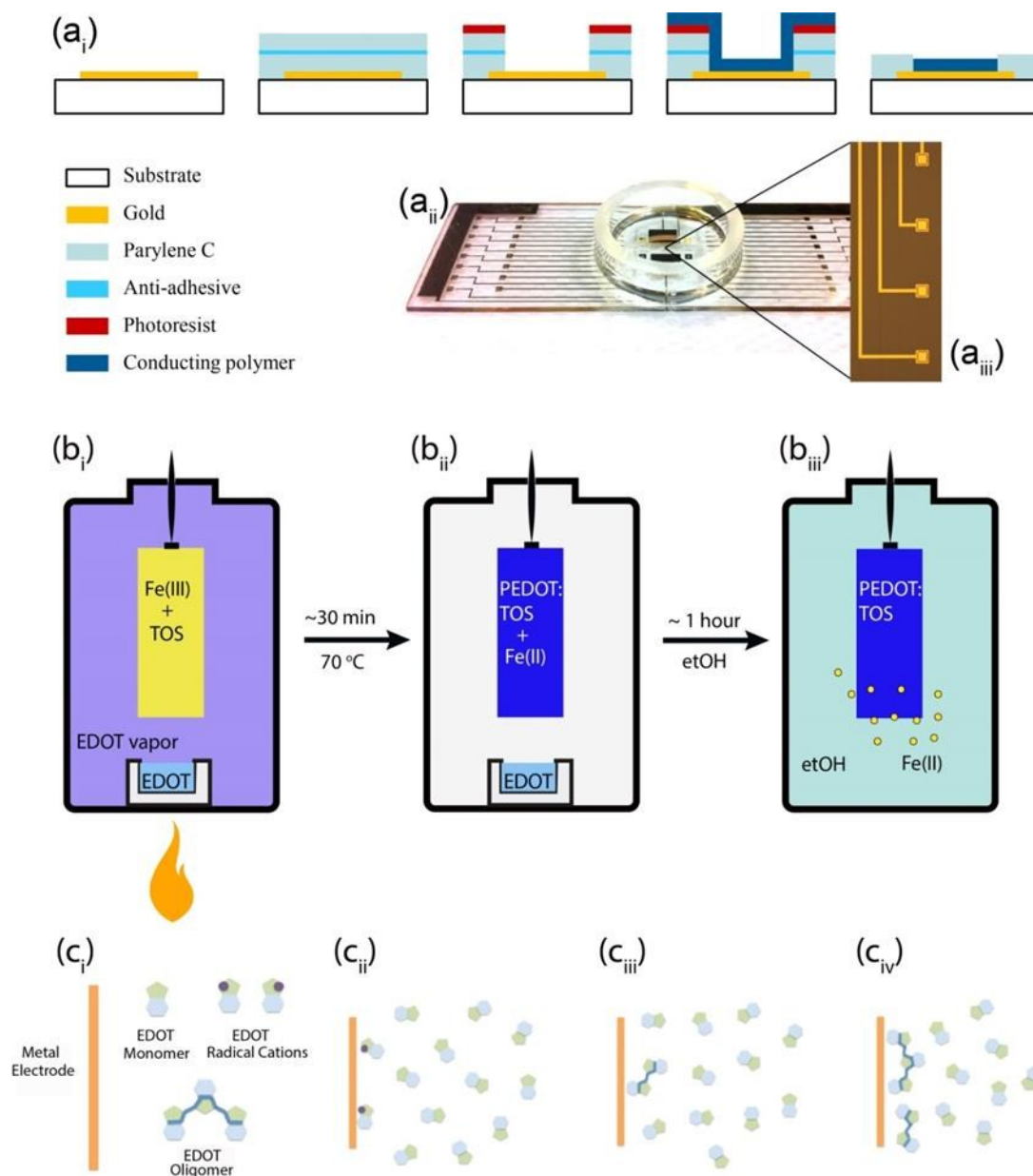
Figure 2: Polydioxythiophenes used in photolithography and polymerization processes: a) Chemically polymerised PEDOT:PSS is commercially available as a dispersion and is highly amenable to photolithographical processes. 7 b) vapor phase polymerization of PEDOT:TOS b i ) a thin film of Fe(III):TOS is inserted into a polymerization chamber. The chamber containing EDOT monomer is heated at 70 °C causing EDOT evaporation and creating a high pressure atmosphere. b ii ) The EDOT polymerizes on the substrate creating a PEDOT:TOS film. b iii ) A final rinsing step with ethanol removes the Fe(II):Fe(III) from the film. c) electrical
