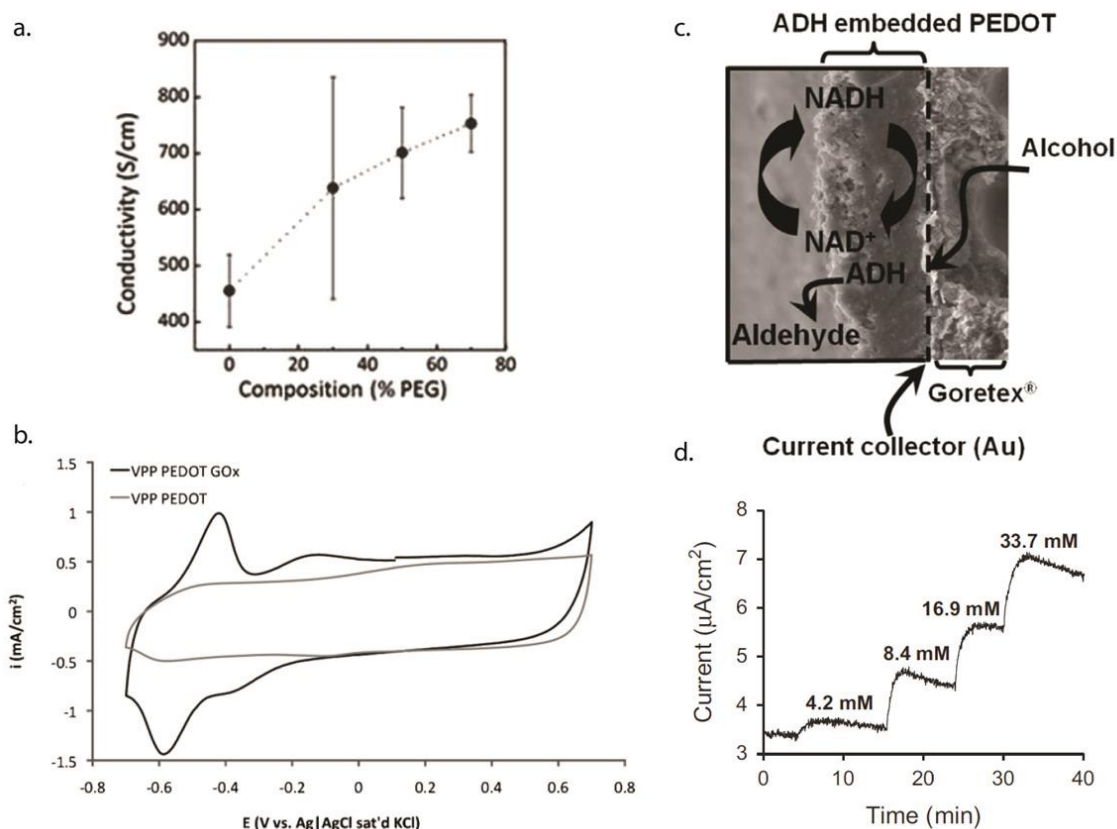
Figure 7: Biofunctionalization of PEDOT:TOS formed by VPP a) conductivity of PEDOT:TOS as a function of PEG content. From Jimison et al. 31 Reproduced by permission of The Royal Society of Chemistry. b) VPP-PEDOT/ GOx shows characteristic peaks of GOx. Post-growth CVs of VPP-PEDOT with and without GOx incorporation (3rd scan shown, taken at 10 mVs -1 ). VPP-PEDOT/GOx shows redox peaks characteristic of GOx at 0.58 to 0.43 V versus Ag/AgCl. From Thompson et al. 66 c) Schematic of the three phase-interface reaction between PEDOT/ADH, alcohol vapour and NAD + /NADH redox couple in the electrolyte. d) current ( I ) modulation as a function of ethanol content. From Winther-Jensen et al. 33
