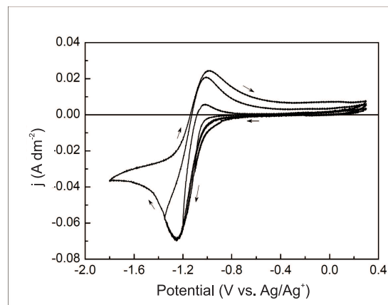
Fig. 1 Cyclic voltammograms of a DMSO solution containing 1 M TBAP and saturated with oxygen gas. Different cathodic vertex potentials were applied, using a glassy carbon disk ( \phi = 1 mm) as working electrode and a platinum coil as counter electrode. The scan rate was 50 \text{ mV s}^{-1} .
