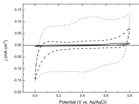
Fig. 11 Capacitance measured via cyclic voltammetry in 0.5 M \text{K}_2\text{SO}_4 aqueous electrolyte using a Pt counter electrode and \text{Ag}/\text{AgCl} reference electrode. A \text{Mn}_x\text{O}_y thin film of approx. 80 nm was deposited on a planar TiN working electrode (dashed) and on TiN coated Si pillars as 3D substrate (dotted). The capacitance of the pillars without \text{Mn}_x\text{O}_y (solid) is shown as reference.
