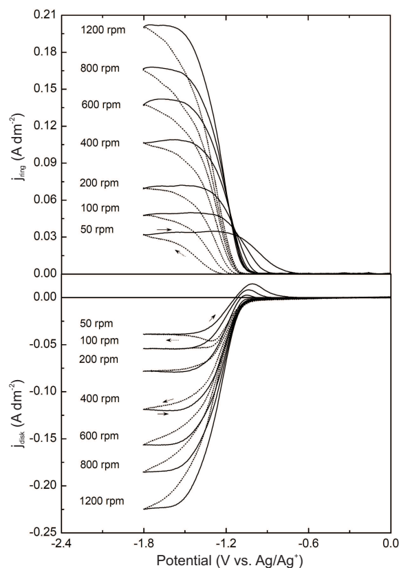
Fig. 2 Disk and ring currents recorded in an oxygen-saturated 1 M TBAP solution in DMSO with different rotation speed at room temperature. The disk current was generated from the cyclic voltammetry with a scan rate of 50 \text{ mV s}^{-1} , and the ring was kept at a potential of -0.2 \text{ V (vs. Ag/Ag}^+) .
