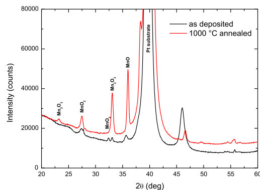
Fig. 8 XRD pattern of electro-precipitated \text{Mn}_x\text{O}_y thin film as deposited (black) and after annealing at 1000 °C (red).
