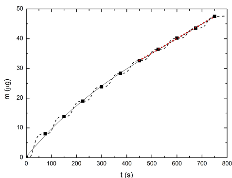
Fig. 5 Mass change was measured by EQCM (dashed line) while performing cyclic voltammetry in an oxygen-saturated DMSO solution with 0.1 \text{ M Mn(Tf}_2\text{N)}_2 . A platinum coated quartz crystal was used as working electrode ( \phi = 12.7 \text{ mm} ), a platinum coil was used as counter electrode and a silver wire was used as pseudo-reference electrode. For the cyclic voltammograms a scan rate of 50 \text{ mV s}^{-1} was applied, with -1.4 \text{ V} and +0.5 \text{ V} vs. Ag as vertex potentials.
