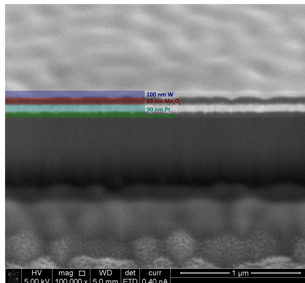
Fig. 6 Electro-precipitated \text{Mn}_x\text{O}_y , deposited via dissolved oxygen reduction in a 0.1 \text{ M Mn(Tf}_2\text{N)}_2 in DMSO solution. The deposition was made by applying cyclic voltammetry for 10 cycles with vertex potentials of -1.4 \text{ V} and +0.5 \text{ V} vs. Ag. As substrate and working electrode a platinum coated ( 90 \text{ nm} ) silicon wafer was used with a TiN buffer layer ( 50 \text{ nm} ). A focussed ion beam of gallium ions was used to etch the sample. To obtain a high-resolution image of the etch pattern, a tungsten layer ( 100 \text{ nm} ) was deposited on top of the 80 \text{ nm} thick \text{Mn}_x\text{O}_y layer.
