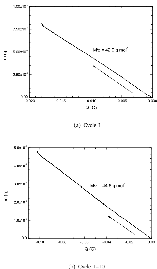
Fig. 7 m vs. Q plots based on the cyclic voltammograms in an oxygen-saturated DMSO solution containing 0.1 M \text{Mn}(\text{Tf}_2\text{N})_2 . M/z values are reported and determined via a linear fit.
