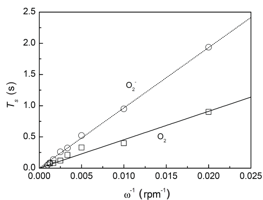
Fig. 3 The transient time change with the inverse of the rotation speed in an oxygen-saturated 1 M TBAP solution in DMSO.
