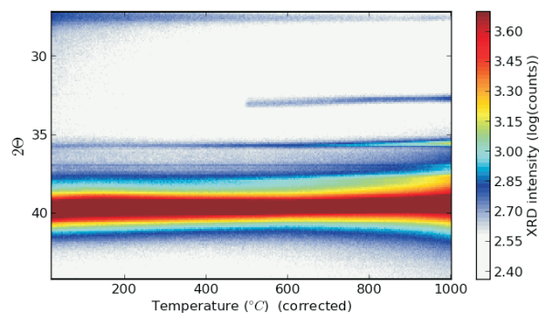
Fig. 9 In situ temperature XRD in air of electro-precipitated \text{Mn}_x\text{O}_y thin film.
