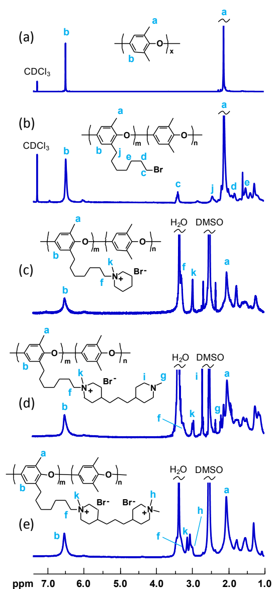
Figure 1. 1 H NMR spectra of native PPO (a), bromoalkylated PPO (PPO-7Br-19) (b), PPO with mono-QPi side chains (PPO-7QPi-1.7Br) (c), semi-quaternized intermediate (d), and PPO with bis-QPi side chains (PPO-7bisQPi-1.8Br) (e).
