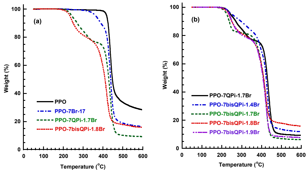
Figure 3. TGA traces of (a) native PPO, a bromoalkylated precursor PPO, a mono-QPi and a bis-QPi functionalized sample, and (b) mono- and bis-QPi functionalized samples with different IEC values. Samples were measured under N 2 at 10 °C min -1 .
