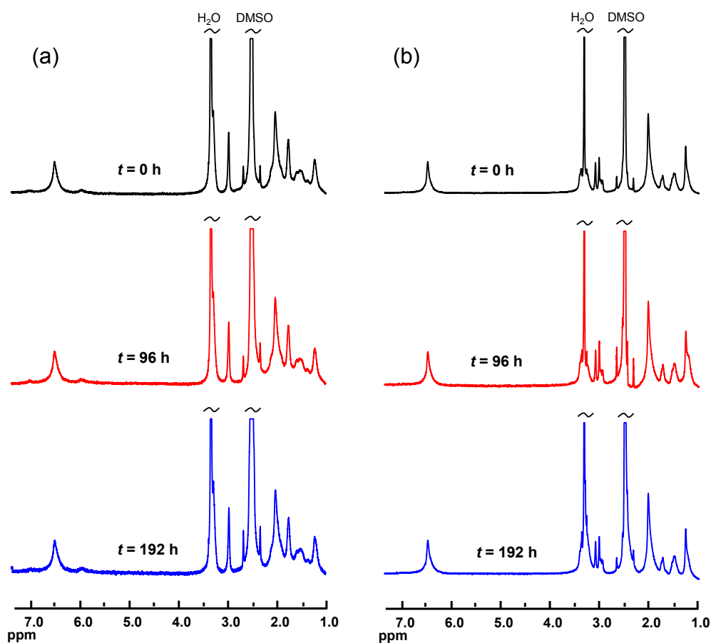
Figure 4. 1 H NMR spectra of PPOs functionalized with mono- and bis-QPi groups PPO-7QPi-1.7 and PPO-7bisQPi-1.7, respectively, after storage in 1 M aqueous NaOH solution at 90 °C during 0, 96, and 192 h, respectively.
