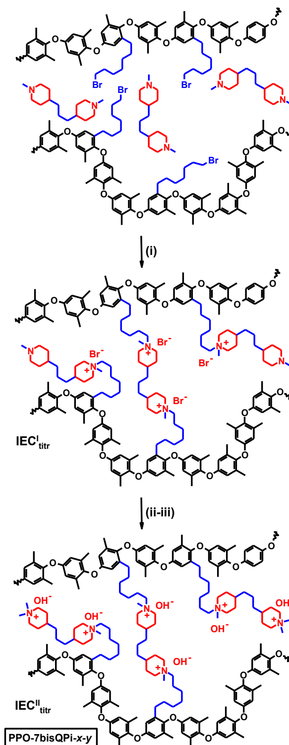
Scheme 2. Preparation of AEMs crosslinked by bis-QPi units via membrane casting/crosslinking (i), methylation (ii), and ion-exchange (iii) [Key: (i) NMP, 85\text{--}105^\circ\text{C} , (ii) MeI, NMP, 40^\circ\text{C} , (iii) aqueous NaOH, 20^\circ\text{C} ].
