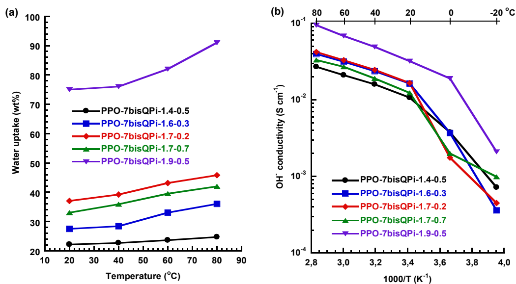
Figure 7. Water uptake (a) and OH - conductivity (b) of the bis-QPi crosslinked AEMs under fully hydrated (immersed) conditions.
