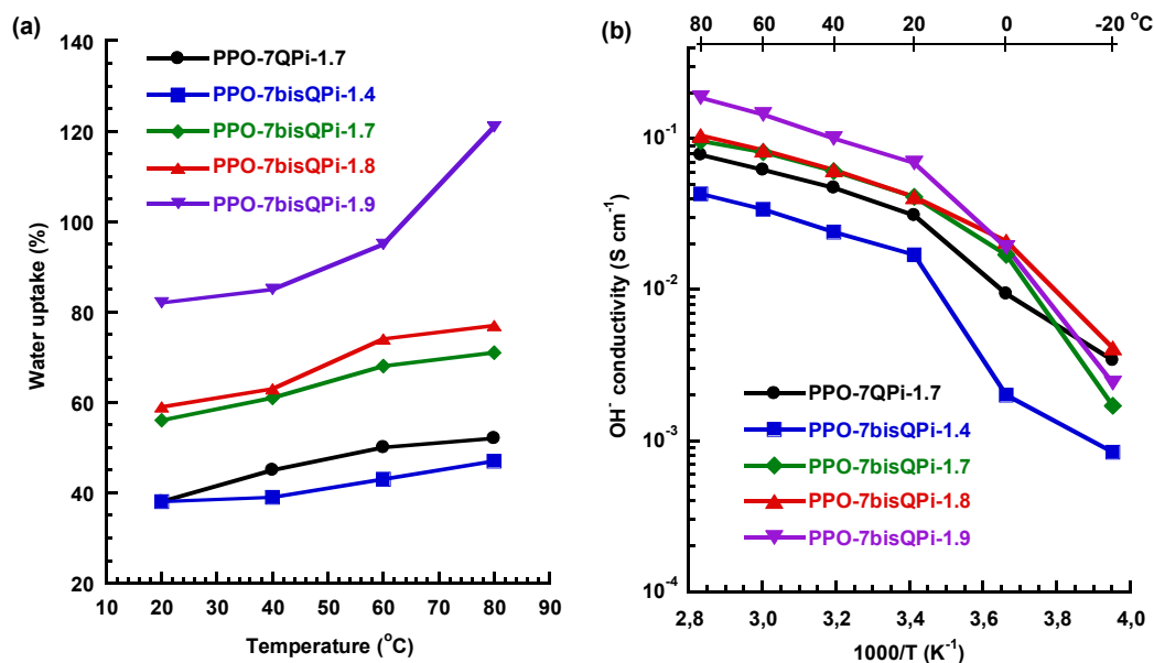
Figure 5. Water uptake of AEMs in the \text{OH}^- form (a) and Arrhenius plots of the \text{OH}^- conductivity (b) of mono- and bis-QPi functionalized PPO AEMs measured under fully hydrated (immersed) conditions.
