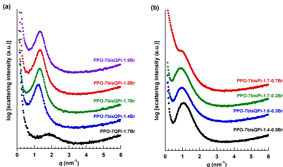
Figure 2. SAXS profiles of dry AEMs based on PPO functionalized with mono- and bis-QPi groups via alkyl spacer units (a), and of dry AEMs crosslinked by bis-QPi units (b). The data were measured with the AEMs in the Br - form and have been shifted vertically for clarity.
