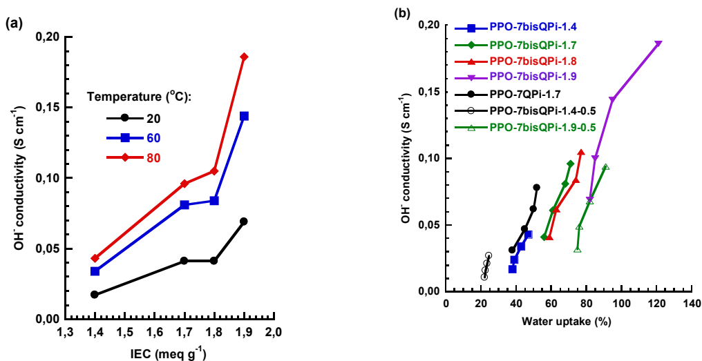
Figure 6. \text{OH}^- conductivity as a function of (a) IEC and (b) water uptake of the AEMs under fully hydrated (immersed) conditions. Data of crosslinked samples are denoted by open symbols.
