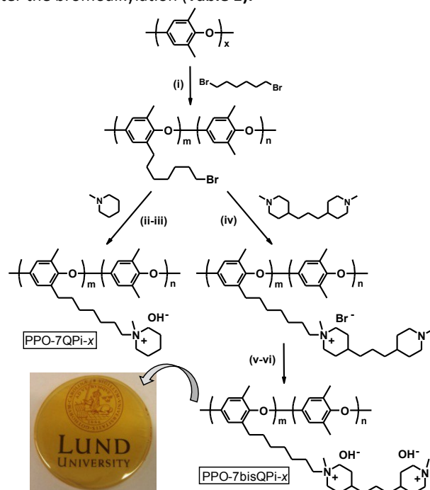
Scheme 1. Synthesis of PPO functionalized with mono- and bis-QPi groups via alkyl spacers. Photograph shows membrane PPO-7bisQPi-1.7 cast from NMP at 80 °C [Key: (i) n -BuLi, THF, -70 °C, (ii) NMP, 85 °C, (iii) aqueous NaOH, 20 °C, (iv) NMP, 85 °C, (v) MeI, NMP, 40 °C, (vi) aqueous NaOH, 20 °C].
