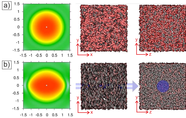
Fig. 9 Simulated scattering patterns and simulation snapshots of the ellipsoids at a packing fraction of \phi = 0.1 , where particles are colour coded according to their orientation given by \hat{L} with respect to the field or x -axis: grey for \hat{L} \perp \mathbf{B} and red for \hat{L} \parallel \mathbf{B} . a) Zero-field case, particles are randomly oriented and show relatively weak positional correlations only. b) Field B = 0.24 T, where the particles are fully aligned with their magnetic moment along the field axis given by the light blue arrow. The middle column shows snapshots in the plane parallel to the field direction ( x-y plane), whereas the right column shows the corresponding snapshots in a plane perpendicular to the field direction ( y-z plane).
