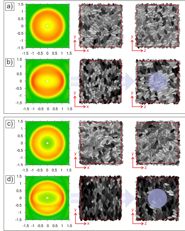
Fig. 7 Simulated scattering patterns and simulation snapshots. a) \phi=0.53 at zero-field. b) \phi=0.53 at B=0.04 T. c) \phi=0.59 at zero-field. d) \phi=0.59 at B=0.04 T. The middle column shows snapshots in the plane parallel to the field direction ( x-y plane), whereas the right column shows the corresponding snapshots in a plane perpendicular to the field direction ( y-z plane), and for systems with an applied field the field direction is also indicated by the light blue arrow. In the snapshots the particles are grey scale coded according to their orientation projected in the plane perpendicular to the field. Black indicates full alignment with respect to the average orientation in the snapshot.
