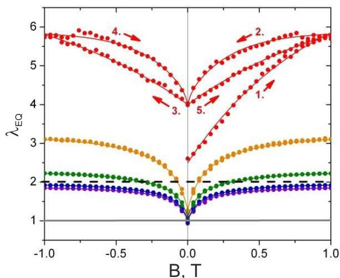
Fig. 6 Full hysteresis loops of the effective order parameter \lambda_{EQ} (Colour online). Shown is a sequence using a range of magnetic field strength -1 \leq B \leq +1 T for a five-branch loop of \lambda_{EQ} for different volume fractions ( \phi=0.59 plotted red, \phi=0.25 orange, \phi=0.19 olive, \phi=0.09 blue, \phi=0.04 violet). The grey line shows the limit of a fully disordered sample \lambda_{EQ} = 1 . The dashed line indicates \lambda_{EQ} = 2 chosen as the threshold value for the formation of a polarised fluid. Arrows indicate the directions of the hysteresis branches. The curves are visual guides only.
