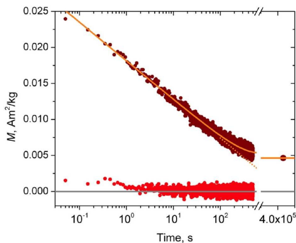
Fig. 11 Magnetic relaxation behaviour for \phi = 0.59 (red) and \phi = 0.77 (wine). The dotted and solid lines fits to a logarithmic time dependence without and with a constant term as given in equation 12. Note the long-time limit value for \phi = 0.77 recorded after 5 days of demagnetisation.
