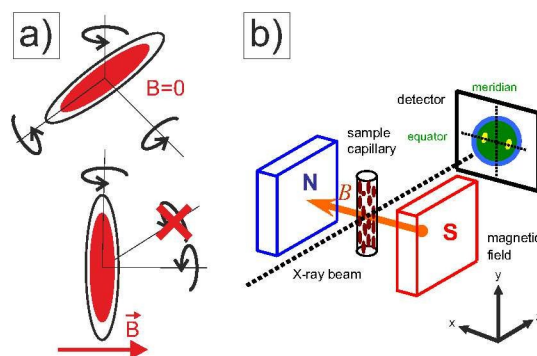
Fig. 2 a) Effect of an applied magnetic field of strength B on the orientation of the magnetic ellipsoids. The particles are aligned with their magnetic moment (parallel to the short particle axis) along the field, while the long axis of each particle is able to freely rotate around the B axis. b) Geometry of the SAXS experiment and definition of the lab frame system. The direction of the uniform magnetic field is in the x -axis, which is always normal to the incident X-ray beam along the z -axis. The scattered X-rays are then recorded on the detector in the x - y - plane.
