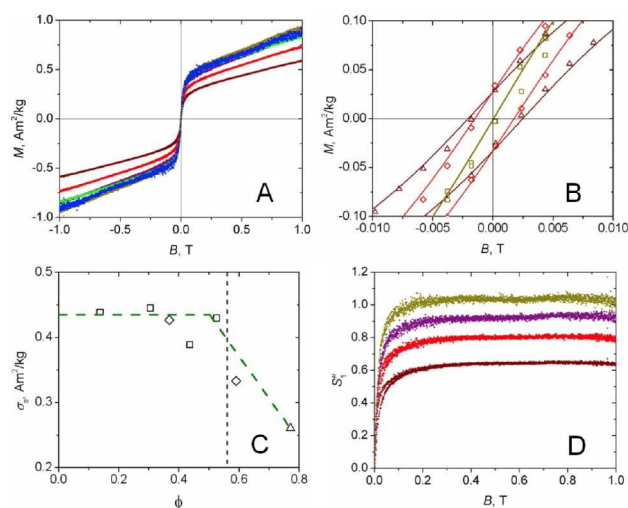
Fig. 10 Bulk magnetic properties of the particle suspensions. A: Net magnetisation is nearly independent on packing fraction for \phi \leq 0.53 ( \phi=0.14 : blue; \phi=0.30 : dark yellow; \phi=0.37 : green; \phi=0.44 : purple; \phi=0.53 : pink), but shows a progressive decay for \phi=0.59 (plotted red) and \phi=0.77 (plotted wine.) B: Same data magnified to highlight regime around B = 0 , the data reveal ferromagnetic-type hysteresis loops for \phi \geq 0.59 yet no hysteresis for \phi=0.30 . C: Saturation magnetisation decreases with packing fraction. D: The Langevin-type behaviour of the first-rank orientational order parameter S_1^\mu reveals the saturation plateau decreasing with packing fraction. Plotted are \phi=0.77 (wine), \phi=0.59 (red), \phi=0.44 (purple), \phi=0.30 (dark yellow.)
