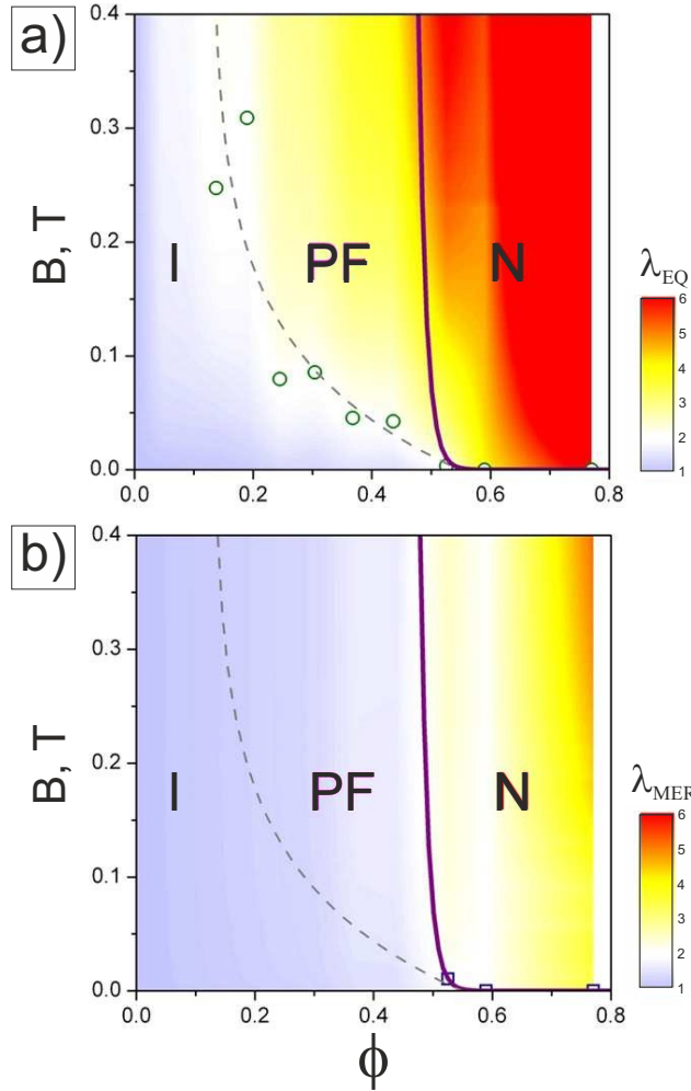
Fig. 8 Phase diagram of the ellipsoids, where we distinguish between an isotropic fluid ( I ), a polarised fluid ( PF ) and a nematic ( N ) phase. a) Effective equatorial order parameter \lambda_{EQ} maps a family of contour lines where the field-induced alignment of the dipole axes results in a particular positional correlation along the x -axis. The values of \phi and B where we experimentally observed the criterion \lambda_{EQ} = 2 are shown as open circles. The dashed line in both figures is a representative contour line \lambda_{EQ} = 2 . The corresponding colour code for \lambda_{EQ} is given on the right hand side of the graph. b) The effective meridian order parameter \lambda_{MER} allows mapping the nematic transition ( \lambda_{MER} = 2 ) as shown by the solid line in both figures. The values of \phi and B where we experimentally observed the criterion \lambda_{MER} = 2 are shown as open squares. The corresponding colour code for \lambda_{MER} is given on the right hand side of the graph.
