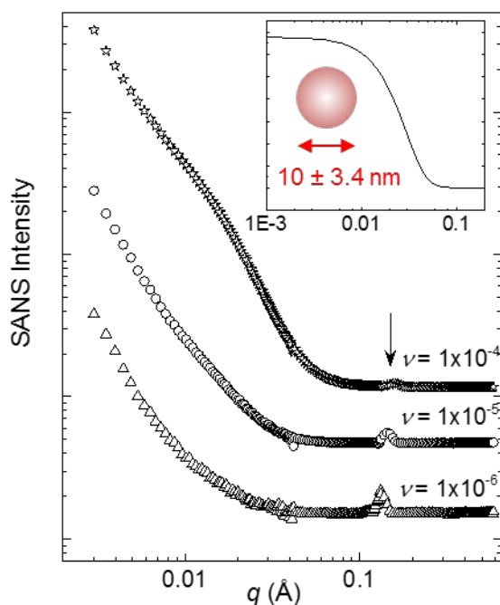
Figure 6 Contrast matched SANS curves on a log-log scale of silica NPs in 30% hydrated MO at \nu of 1 \times 10^{-4} , 1 \times 10^{-5} and 1 \times 10^{-6} , measured at 15 °C. The solvent was a mixture of \text{H}_2\text{O}:\text{D}_2\text{O} at a volume ratio of 89:11, to match the scattering length density of MO. The SANS curves showed little temperature dependence, with the curves at all the temperatures shown in Figure S4. The inset shows a model SANS curve for 10 \pm 3.4 nm spherical nanoparticles (modelled using SansView), with the polydispersity modelled as a Gaussian distribution. The SLD of the contrast matched solvent was 2.1 \times 10^{-5} \text{ \AA}^{-2} , and that for the silica sphere was 3.475 \times 10^{-6} \text{ \AA}^{-2} . The vertical scale of the curves has been displaced for clarity.
