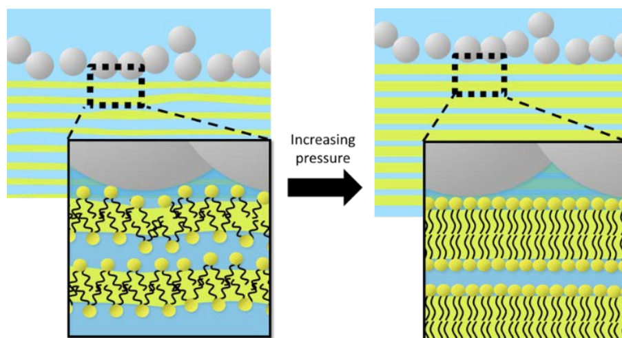
Figure 7 At higher NP \nu , the NPs may form chain of pearl-like aggregates. These aggregates reside at the domain interface. Upon increasing the pressure, the L_{\alpha} phase to the Q_{II}^G phase transition is suppressed. To seek smaller volumes, the lipids would adopt denser packing. As a result, the L_D phase would rearrange, eventually forming the L_{\alpha} and then the L_C domains, with the NPs retaining the chain of pearls structure at the domain boundaries.
