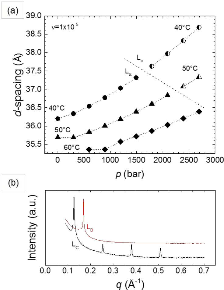
Figure 5 (a) Comparison of the d -spacing values for L_D and L_c phases at 40, 50 and 60 °C at v of 1 \times 10^{-5} . The d -spacing for both L_\alpha and L_D followed the same increasing trend with pressure (dotted lines as a guide for the eye). (b) 1D SAXS curves showing the appearance of higher order Bragg peaks after the L_D - L_c transition, suggest an enhanced order in the lamellar structure rather than a complete mesophase transition. The vertical scale of the curves has been displaced for clarity.
