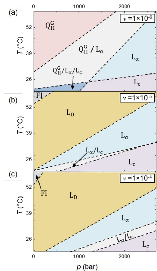
Figure 4 p - T diagrams of MO mesophases containing silica NPs at v of (a) 1 \times 10^{-6} , (b) 1 \times 10^{-5} , and (c) 1 \times 10^{-4} between 20 – 60 °C and 1 – 2700 bar. At lower v , the NPs stabilised the Q_{II}^G phase so that its phase region persisted to higher pressures and lower temperatures. However, at higher NP v , the Q_{II}^G phase was suppressed and the lamellar phases were retained until the fluid isotropic (FI) phase formed.
