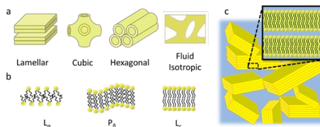
Figure 1 a) Lipids may self-assemble to form the lamellar, cubic, hexagonal and fluid isotropic phases, with different curvatures in the constituent monolayers. b) The fluid ( L_{\alpha} ), ripple ( P_{\beta} ) and crystalline ( L_c ) of the lamellar phases. c) Schematic of domains of L_c stacks at low hydration.
