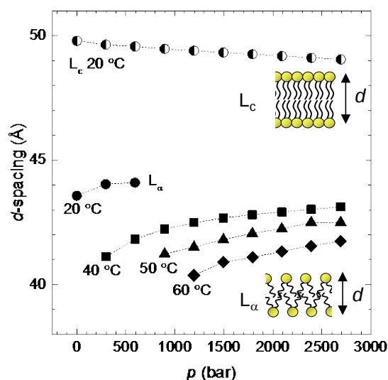
Figure 3 d -spacing vs p for the MO L_\alpha (filled symbols) and L_c (partially filled circles) mesophases. The d -spacing for the L_\alpha phase increased slightly with pressure, whereas that for the L_c phase remained largely constant. The uncertainty in the d -spacing is estimated as \sigma_d = 0.02 Å. The stability of the pressure within the sample cell was \pm 5 bar 58 .
