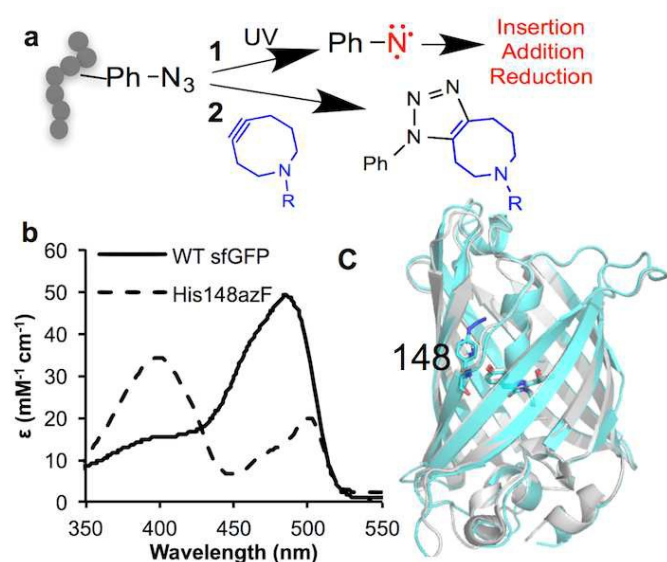
Figure 1. Incorporation of phenyl azide chemistry into sfGFP. (A) Routes for modulating protein activity via nnPTM; 1 – photochemistry, 2 – SPAAC addition (B) Switch in sfGFP (black line) absorbance on mutating H148 to azF (dashed line). (C) Crystal structure of dark state sfGFP 148azF (cyan) overlaid with sfGFP (PDB 2B3P 26 ).
