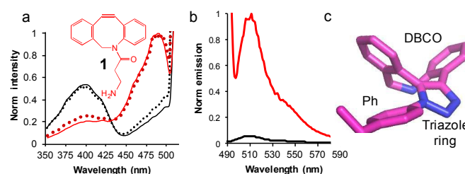
Figure 3. The use of SPAAC to switch sfGFP 148azF function (A) Change in fluorescence excitation spectra in vitro (solid line) and in vivo (dotted line) in the absence (black) and presence (red) of DBCO-amine ( 1 , inset). In vivo experiments represent fluorescence from intact cells after incubation of 1 with cell cultures for up to 8 hr. (B) Emission spectra on excitation of 400 nm (black line) and 485 nm (red line) of isolated sfGFP H148azF modified with 1 . The unmodified sfGFP 148azF emission spectra is shown in Figure S1; the major emission peak corresponds to excitation at 400 nm. (C) Determined structure of the DBCO moiety linked to azF148. The amino acid side chain (Ph), triazole link and DBCO are shown.
