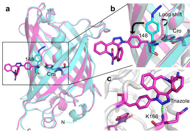
Figure 4. Structure of SPAAC modified sfGFP 148azF . (A) Overlay of sfGFP 148azF pre (cyan) and post (magenta) modification with 1 . (B) Close-up of the region around residue 148. Original sfGFP is coloured grey. (C) Putative H-bond (green dashed line) formed between the triazole link and K166.
