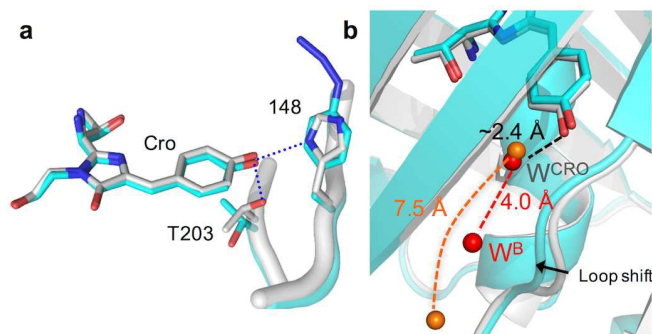
Figure 2. Structural changes on mutating H148 to azF. Original sfGFP and sfGFP 148azF are coloured grey and cyan respectively. (A) The chromophore (Cro) with T203 and 148 highlighted (H-bonds in sfGFP are shown as blue dots and absent in sfGFP 148azF ). The terminal N 2 group of azF148 represents a modelled structural representation. (B) Positions of water molecules (W) in sfGFP 148azF (orange balls) and original sfGFP (red balls).
