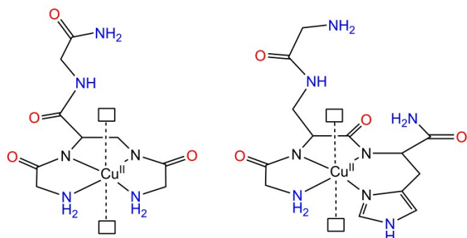
Scheme 1 Structural representation 27 and short name of the Cu(II) complexes subject to the present study. Open rectangles represent sites of water coordination. Ligands are H-Gly-Dap(H-Gly)-Gly-NH 2 (3G) and H-Gly-Dap(H-Gly)-His-NH 2 (2GH). Potential H-bonding sites are marked with red and blue.
