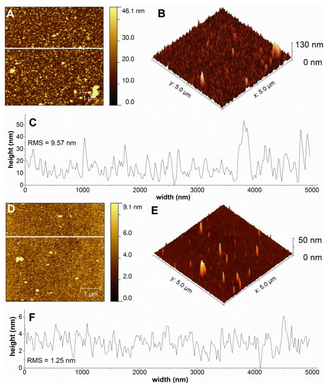
Figure 2 (A) Representative AFM image ( 5 \times 5 \mu\text{m} ) of the Cu-3G/PLL /phosphate composite layers; (B) 3D view of the same area; (C) profilometric section of the AFM image; (D)-(F) the same images for the Cu-2GH/PAH /phosphate LbL formations. 8 deposition cycles were conducted in both cases according to method (A) at pH = 10. The places of profilometric cross-sections are indicated by white lines in (A) and (D).
