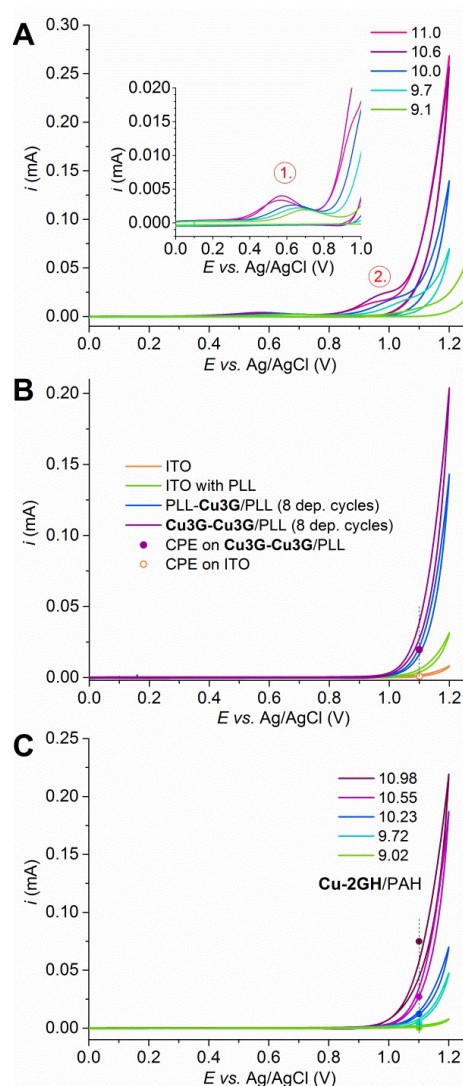
Figure 3 (A) First cycle of CVs of LbL-ITO electrodes treated with 8 deposition cycles of Cu-3G/PLL (pH = 10) in 0.1 M phosphate solution at different pH values as indicated, inset: blown up picture of the current peak attributed to the Cu(II)/Cu(III) transition of the surface adsorbed Cu-3G ; (B) third cycle of CVs of ITO electrodes with or without Cu-3G/PLL (deposited at pH = 10) in 0.1 M phosphate solution at pH = 10.64 (see legend and text for details); (C) third cycle of CVs of LbL-ITO treated with 8 deposition cycles of Cu-2GH/PAH (pH = 10) in 0.1 M phosphate solution at pH = 10.55 (for colour codes see the legend, open circles stand for CPE current after 5 min). Scan rates were 25 mV/s uniformly.
