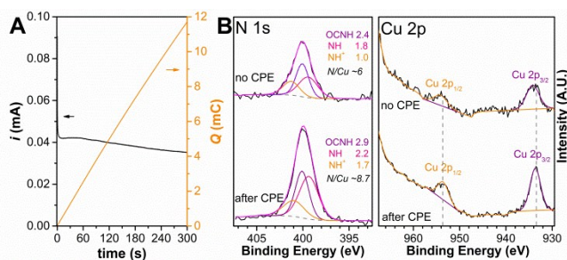
Figure 5 (A) CPE current ( i at 1.1 V) and charge on an LbL-ITO treated with 8 Cu-3G /PLL/phosphate deposition cycles (surface area ~1.4 cm 2 ); (B) XPS analysis of N and Cu on the electrode after CPE and the same analysis on another LbL-ITO prepared analogously, but unused (numbers indicate relative contributions).
