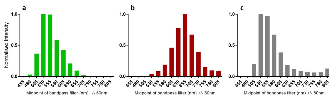
Figure 5. Emission spectra of luciferin and analogues with wild-type Photinus pyralis luciferase. a. 0.17 \mu M Fluc was mixed with 150 \mu M D-luciferin ( 1 ) and 2 mM ATP and emission spectra were obtained using the PIO. b. infra-luciferin ( 5 ) in same conditions as (a). c. 3 \mu M WT Fluc was used to acquire spectra with ( 6 ).
