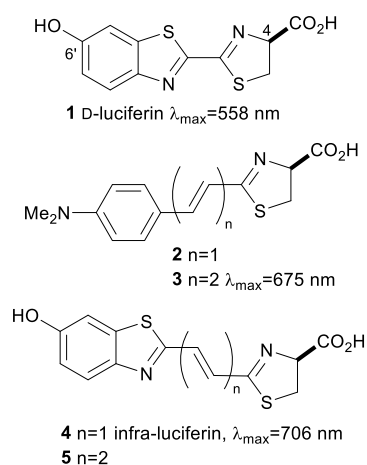
Figure 1: Firefly D-luciferin and synthetic extended conjugation analogues.
