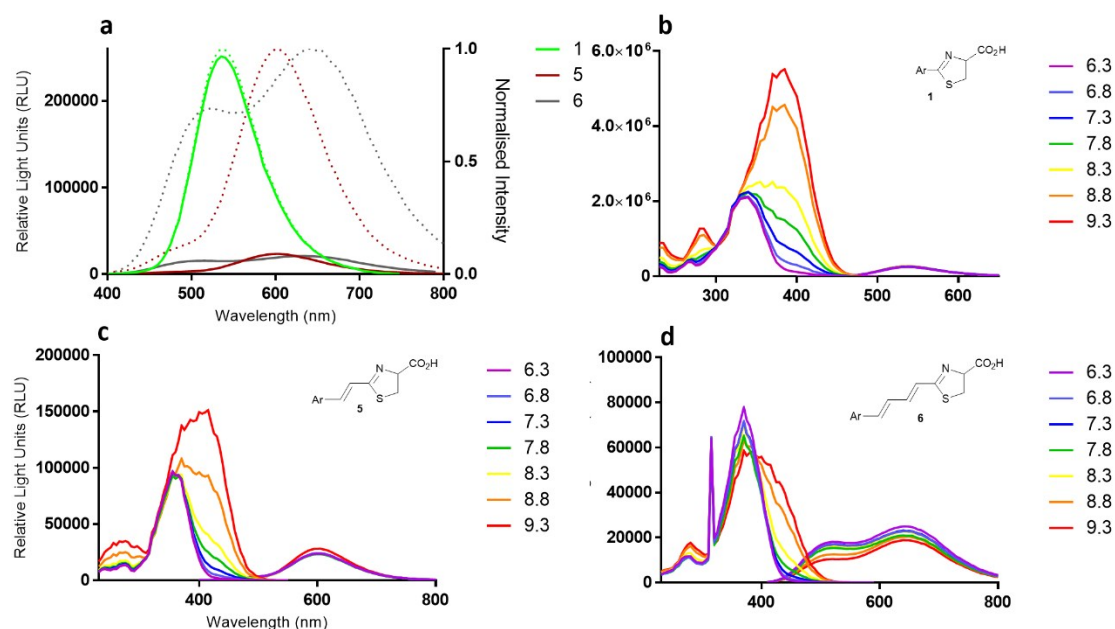
Figure 3. a. Normalised fluorescence emission spectra of D-luciferin ( 1 ) (green line), infra-luciferin ( 5 ) (red line) and 6 (black line). Dotted lines are normalized spectra, b. pH dependence of fluorescence spectra of D-luciferin ( 1 ) (330 nm excitation), c.
