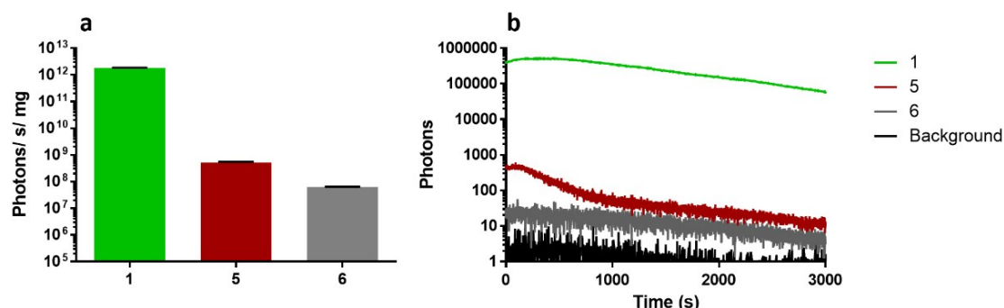
Figure 4. Quantification of light emission of luciferin and analogues with wild-type Photinus pyralis luciferase. 2 mM ATP was added to 0.5 \mu M pure Flucs mixed with 150 \mu M substrates and these were assayed in the PIO with and open filter to measure a. specific activity, and b. kinetics over 50 min.
