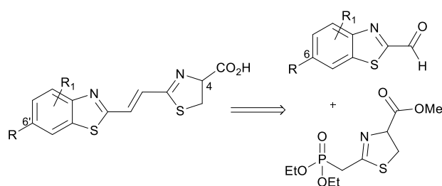
Figure 2: Proposed disconnection for the rapid synthesis of conjugated luciferin analogues.
