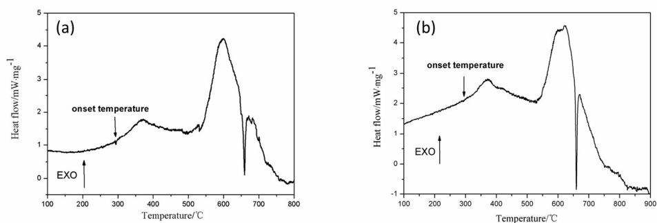
Fig. 5. DSC curve of Al/NiFe 2 O 4 membrane with an aluminizing duration of (a) 30 min and (b) 45 min
