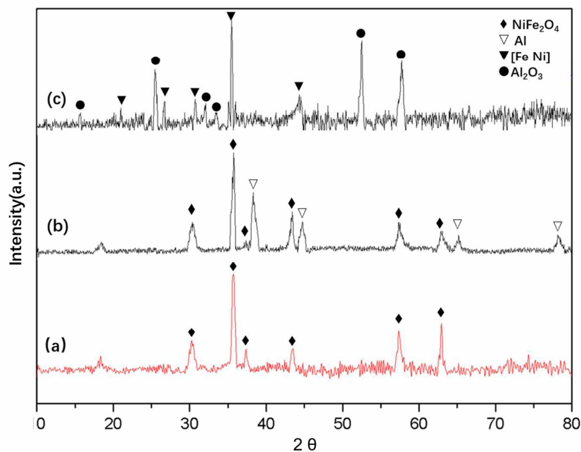
Fig. 1. XRD patterns of (a) NiFe 2 O 4 membrane after calcination, (b) Al/NiFe 2 O 4 membrane, (c) Al/NiFe 2 O 4 membrane after a DSC test
