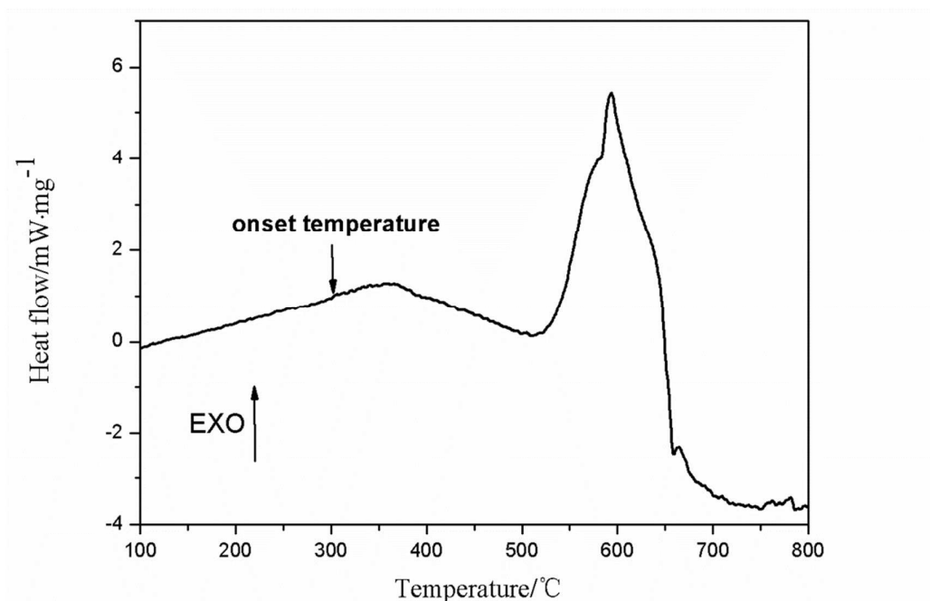
Fig. 4. DSC curve of Al/NiFe 2 O 4 membrane with an aluminizing duration of 15 min obtained in a temperature range from 100 to 800 °C with a heating rate of 20 °C min -1 under a 30.0 mL min -1 N 2 flow.
