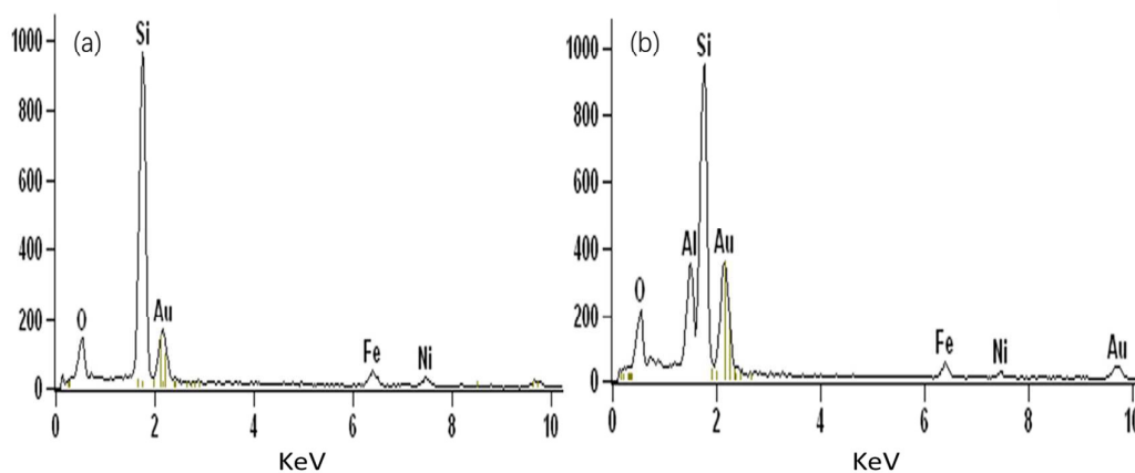
Fig. 2. EDS patterns of (a) NiFe 2 O 4 membrane and (b) Al/NiFe 2 O 4 membrane
