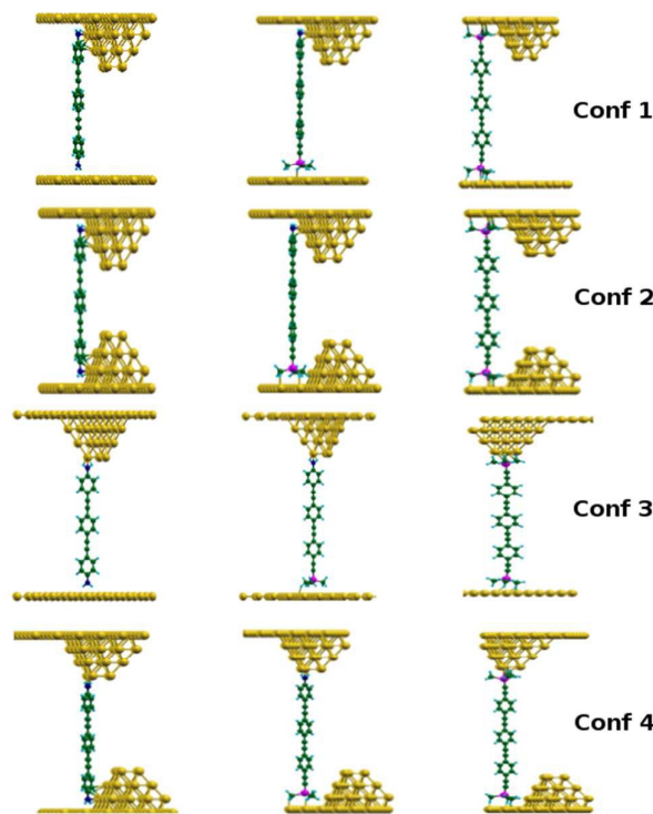
Figure 1. The four configurations (Conf. X, X=1, 2, 3 and 4) used to start the ab-initio molecular dynamics (MD) simulations of each junction for compounds 1 , 2 and 3 (left, middle and right columns, respectively).
