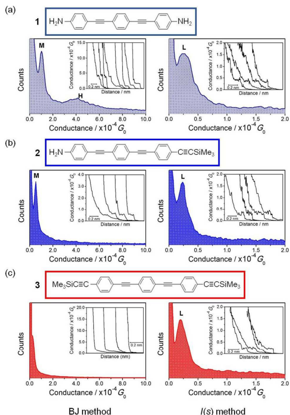
Figure 2. Conductance histograms built from summation of conductance traces (ca. 450) that showed discernible plateaus (with a current plateau which exceeds 0.1 nm in length) such as those displayed in the inset of the figures using either the STM-BJ technique (left side) or the I(s) method (right side). (a) compound 1 , (b) compound 2 and (c) compound 3 . Conductance data are referenced to the conductance quantum G_0 = 2e^2/h = 77.5 \mu S . U_{tip} = 0.6 V .
