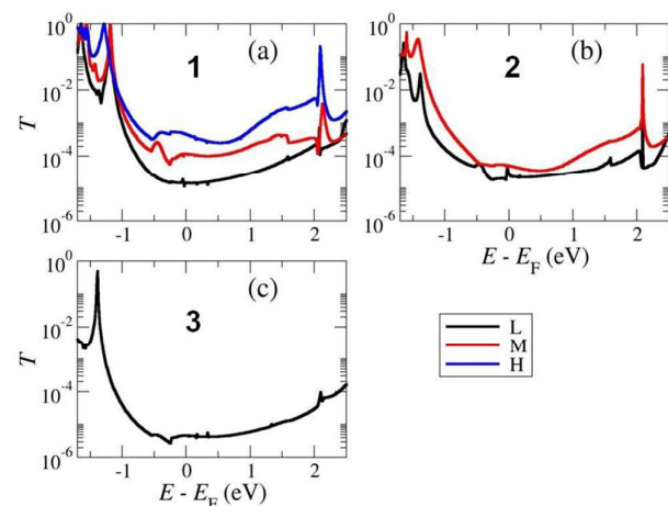
Figure 6. Transmission as a function of energy for a junction comprising (a) compound 1 , (b) compound 2 and (c) compound 3 on a gold surface with pyramids.
