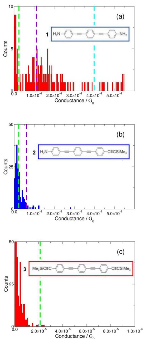
5. Conductance histograms of (a) compound 1 (b) compound 2 and (c) compound 3 . Vertical dashed lines correspond to the experimental values of the conductance groups (e.g. three conductance groups for 1 , two conductance groups for 2 and one conductance group for 3 ).
