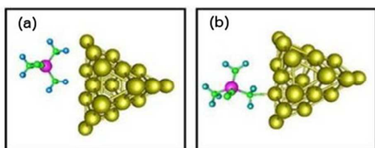
Figure 4. A top view of the relative -C\equiv CSiMe_3 group-pyramid arrangements. Blue, green, magenta and yellow atoms represent hydrogen, carbon, silicon and gold atoms, respectively. Only the gold atoms of the pyramid are shown but not the underlying gold terrace.
