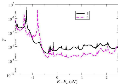
Figure 7. Transmission as a function of energy for a junction comprising 3 and 4 (solid black and magenta dashed solid lines, respectively) on a flat gold surface (without pyramids), calculated at the equilibrium distances (3.8 Å and 5.0 Å from the Si atom to the surface for 3 and 4 , respectively).
