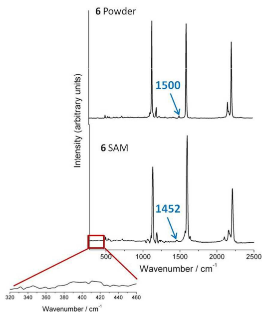
Figure 3. Raman spectra of 6 in the solid state and as a self-assembled monolayer on a silver mirror.
