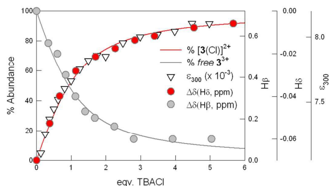
Figure 5: 1 H-NMR and UV-vis profiles for the titration of 3^{3+} with TBACl in acetonitrile/DMSO mixture. The distribution diagram was obtained, by considering a 1:1 binding constant of 4.04 Log units (see Table 5). For details see the text; further material is available in SI (see Fig. S15 for the family of 1 H NMR spectra).
