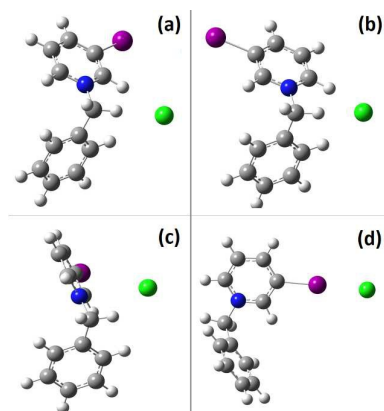
Figure 2. Geometries of four possible conformers for the binding of Cl - by 1a .
