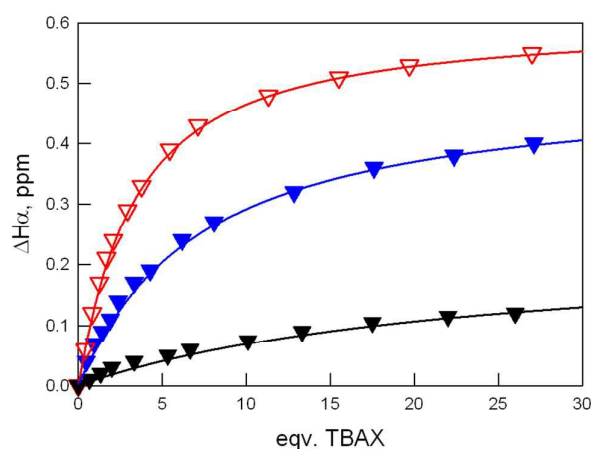
Figure 1. 1 H-NMR titrations of 1a + with halides in CD 3 CN. Variation of the chemical shift of H α upon anion (as TBA salt) addition (symbols: red, chloride; blue, bromide; black, iodide). The experimental profiles are superimposed to the formation curves of the 1:1 adducts with the anions, calculated according to the constants reported in Table 1.
