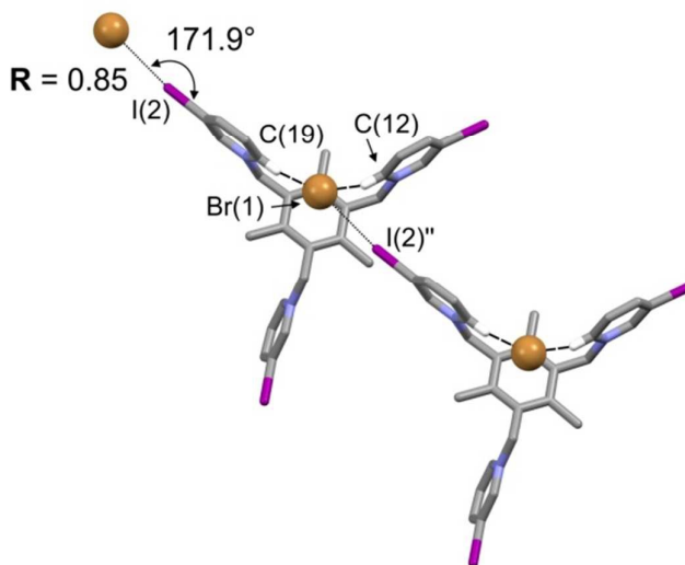
Figure 7. A simplified sketch of the crystal structure of 2(\text{Br})(\text{PF}_6)_2 ( \text{PF}_6^- counter ions are not shown for simplicity). Names are shown only for atoms involved in C-I...Y halogen bonds (drawn with dotted lines) and C-H...A hydrogen bonds (drawn with dashed lines). The normalized R values = d_{\text{I...Y}}/(r_{\text{I}}+r_{\text{Y}}) and the C-I...Y bond angles are reported. Symmetry code: (') x, -1+y, z ; (") -1+x, y, z .
