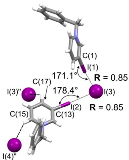
Figure 3. A simplified sketch of the crystal structure of 1a (I). Atom names are shown only for atoms involved in C–I...Y halogen bonds (drawn with dotted lines) and weak C–H...A hydrogen bonds (drawn with dashed lines). The normalized R values = d_{i...y}/(r_i+r_y) and the C–I...Y bond angles are reported. Symmetry code: (') = -1+x, 1/2-y, -1/2+z; (") = 1+x, y, z.
