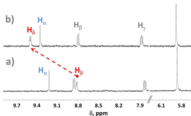
Figure 4: 1 H-NMR spectra of 3^{3+} in CD_3CN/d^6 -DMSO mixture (10% d^6 -DMSO), taken before (a) and after addition of excess TBACl (b). The family of spectra is shown in the SI.
