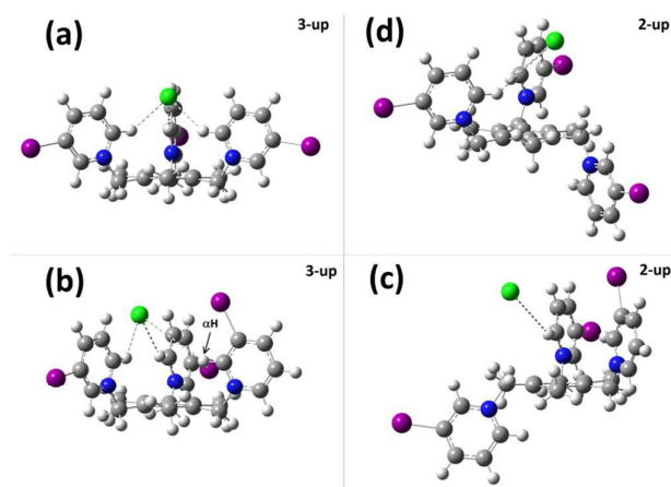
Figure 6. Lowest conformers for 2^{3+}/\text{Cl}^- . Note that top and bottom conformers differ due to the rotation of an iodo-pyridinium group in the up position around the \text{CH}_2\text{-N} bond. Such rotation substitutes \text{H}\alpha to \text{H}\delta in the contact with the anion.
