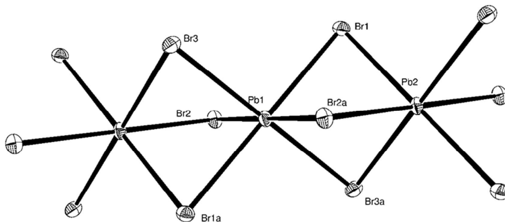
Figure 1 The structure of a portion of the chain polymer anion present in [\text{PPh}_4][\text{PbBr}_3] showing the atom labelling scheme. Ellipsoids are drawn at the 50% probability level. Symmetry operation: a = -x, -y, -z . Selected bond lengths (Å) and angles (°): Pb1–Br1 = 3.0416(8), Pb1–Br2 = 3.0332(8), Pb1–Br3 = 2.9823(6), Pb2–Br1 = 3.0179(7), Pb2–Br2a = 3.0176(6), Pb2–Br3a = 3.0296(7), Br1–Pb1–Br2 = 92.89(2), Br1–Pb1–Br3 = 96.094(16), Br2–Pb1–Br3 = 88.18(2), Br1–Pb1–Br2a = 87.11(2), Br1–Pb1–Br3a = 83.906(16), Br2–Pb1–Br3a = 91.82(2), Br1–Pb2–Br2a = 87.82(2), Br1–Pb2–Br3a = 83.51(2), Br2a–Pb2–Br3a = 87.60(2).
