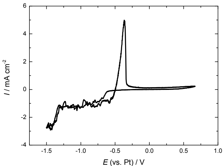
Figure 5 Cyclic voltammetry of 2 mM [\text{PPh}_4][\text{PbCl}_3] + 50 mM [\text{N}^n\text{Bu}_4]\text{Cl} at a Pt disk electrode (surface area 1.963 \times 10^{-3} \text{ cm}^2 ) in \text{scCH}_2\text{F}_2 (17.5 MPa, 360 K). The potential scan rate was 50 \text{ mV s}^{-1} .
