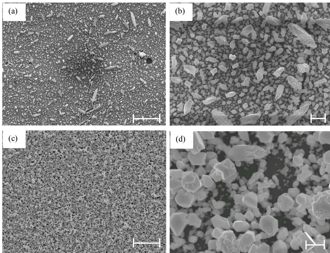
Figure 6 SEM micrographs of Pb electrodeposited on planar electrodes in \text{CH}_2\text{Cl}_2 . The substrates and magnifications used are (a) Au, x2000 (scale bar = 10 \mu\text{m} ), (b) Au, x10000 (scale bar = 1 \mu\text{m} ), (c) TiN, x2000 (scale bar = 10 \mu\text{m} ), (d) TiN, x13000 (scale bar = 1 \mu\text{m} ).
