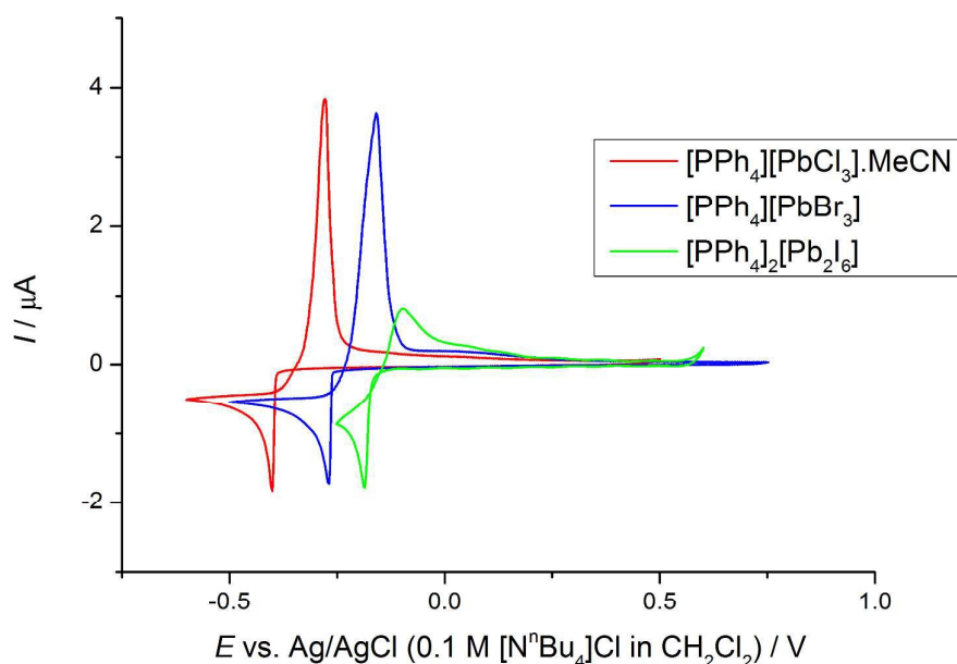
Figure 4 Cyclic voltammograms of [\text{PPh}_4][\text{PbX}_3] ( X = \text{Cl}, \text{Br}, \text{I} ) in \text{CH}_2\text{Cl}_2 recorded at a 0.5 mm diameter Pt disk. The composition of each electrolyte system was 0.5 mM (based on Pb content) of (i) [\text{PPh}_4][\text{PbCl}_3] , (ii) [\text{PPh}_4][\text{PbBr}_3] and (iii) [\text{PPh}_4]_2[\text{Pb}_2\text{I}_6] with 100 mM [\text{PPh}_4]\text{X} . The potential scan rate was 50 \text{ mV s}^{-1} .
