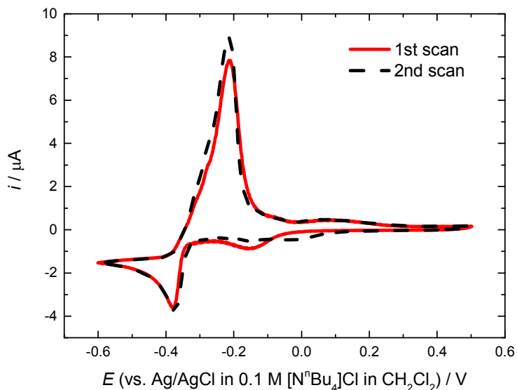
Figure 3 Cyclic voltammograms of 0.5 mM [\text{PPh}_4][\text{PbCl}_3]\cdot\text{CH}_3\text{CN} in \text{CH}_2\text{Cl}_2 recorded at a 1.0 mm diameter Au disk. The supporting electrolyte used was 100 mM [\text{PPh}_4]\text{Cl} and the potential scan rate was 50 \text{ mV s}^{-1} .
