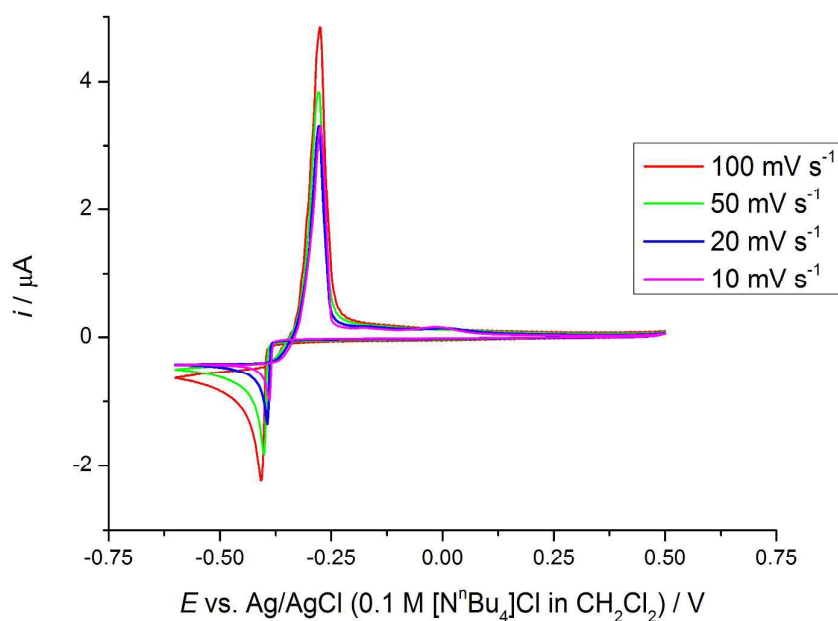
Figure 2 Cyclic voltammograms of 0.5 mM [\text{PPh}_4][\text{PbCl}_3] in \text{CH}_2\text{Cl}_2 as a function of scan rate, recorded at a 0.5 mm diameter Pt disk. The supporting electrolyte used was 100 mM [\text{PPh}_4]\text{Cl} .
