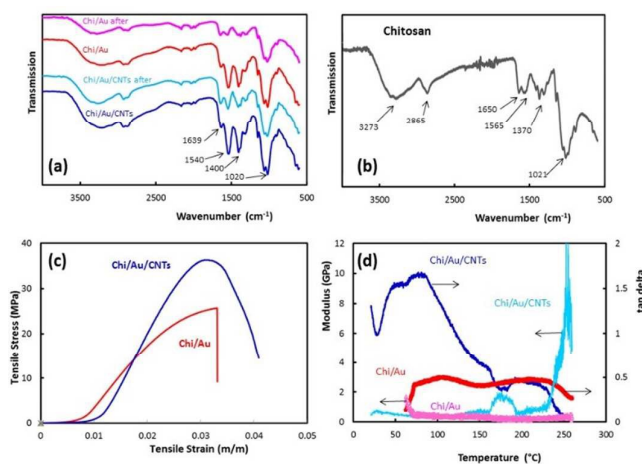
Fig. 4. FT-IR spectra of (a) Gold-Nanocomposites, (b) chitosan. Representative tensile stress-strain curves (c), Storage modulus and \tan \delta versus temperature for Chi/Au and Chi/Au/CNTs (d).
