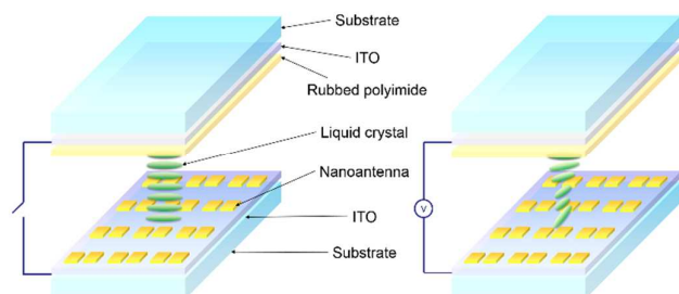
Figure 2. Schematic of the LC cell with a nanoantenna-patterned surface on the bottom substrate. An applied electric field across the cell reorients the nematic molecules and, in turn, changes the wavelength of resonance.
