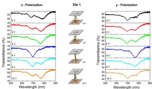
Figure 4. Transmission spectra of the LC cell with the die-1 nanoantenna array on the bottom substrate at various applied voltages under the x- and y-polarizations.
