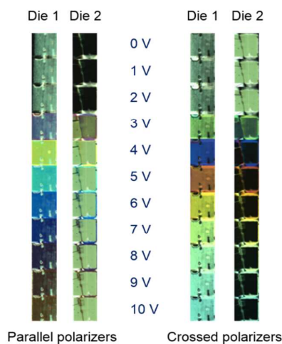
Figure 6. Polarizing micrographs of the LC cell covering regions of die 1 and die 2.
