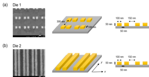
Figure 1. Scanning electron micrographs of gold nanoantenna arrays in (a) die 1 and (b) die 2.
