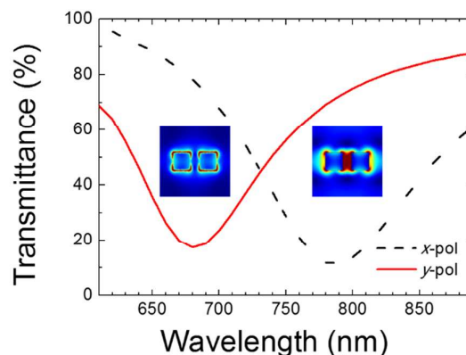
Figure 3. Simulated far-field spectra of the die-1 nanoantenna array for linearly polarized EM waves with the x- and y-polarizations. The resonance wavelength shifts from 780 to 680 nm when the polarization changes from the x- to the y-polarization. The insets depict the localized EM field distributions.
