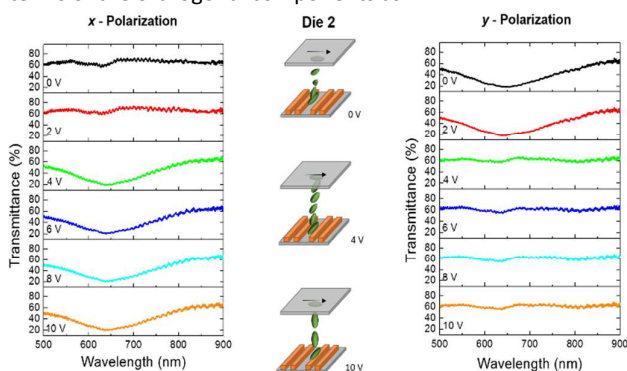
Figure 5. Transmission spectra of the LC cell with the die-2 nanoantenna array on the bottom substrate at various applied voltages under the x - and y -polarization conditions.
