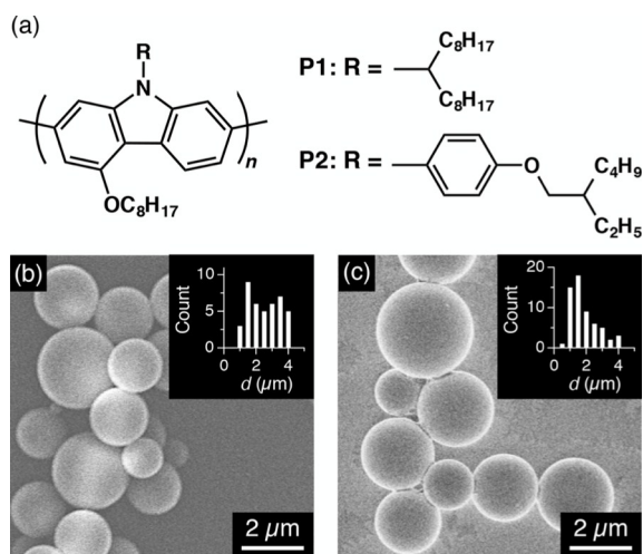
Fig. 1. (a) Molecular structures of poly(2,7-carbazole) P1 and P2 . (b, c) SEM micrographs of self-assembled microspheres of P1 (b) and P2 (c). Insets show histograms of d of the microspheres.
