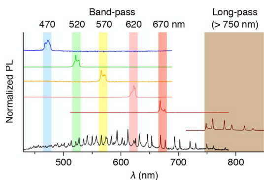
Fig. 4. PL spectra of a single microsphere of P1 , upon focused laser excitation ( \lambda_{\text{ex}} = 405 \text{ nm} ), without an optical filter (black), with band-pass filters centered at 470 (blue), 520 (green), 570 (orange), 620 (pale-red) and 670 nm (deep red) and with a long-pass filter ( > 750 \text{ nm} , brown).
