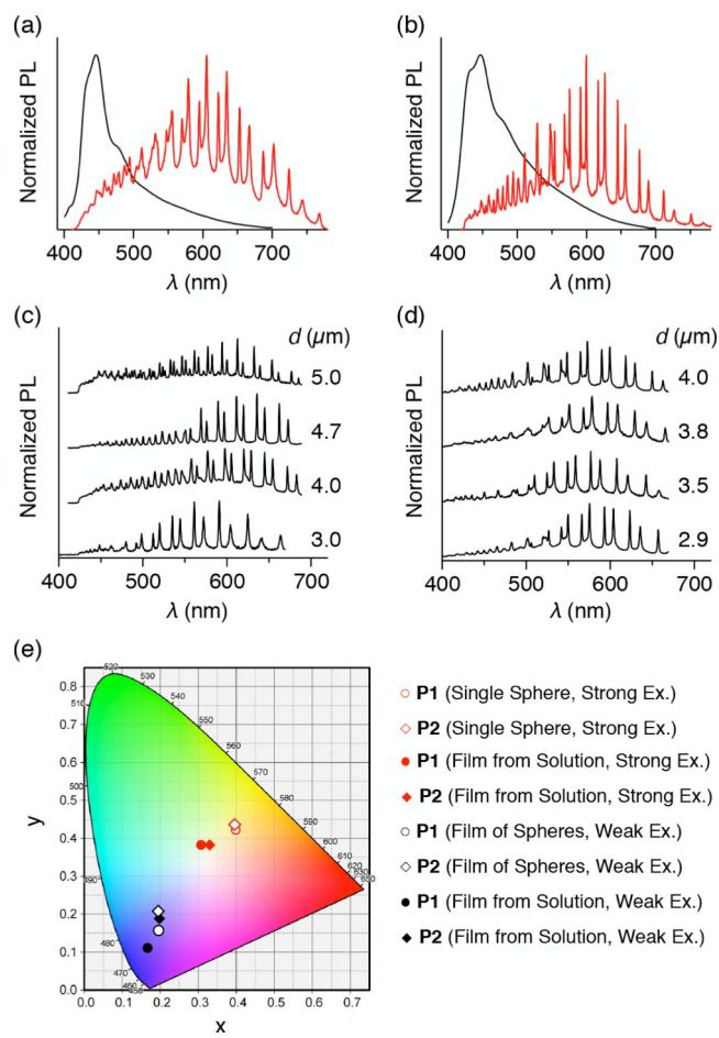
Fig. 2. (a, b) PL spectra of microspheres of P1 (a) and P2 (b). Black spectra show PL of a thin film of the microspheres upon excitation with stationary light ( \lambda_{\text{ex}} = 380 \text{ nm} ), while red spectra shows PL from a single microsphere upon focused laser excitation ( \lambda_{\text{ex}} = 405 \text{ nm} ). (c, d) PL spectra of a single microsphere of P1 (c) and P2 (d) with different d . (e) CIE coordinates of P1 (circles) and P2 (squares) upon excitation with stationary light (black) and focused laser (red) to microspheres (open symbols) and cast films from solution (closed symbols).
