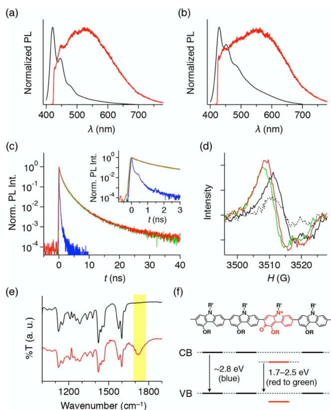
Fig. 3. (a, b) PL spectra of thin films of P1 (a) and P2 (b), prepared by drop-cast from \text{CHCl}_3 solutions, upon excitation with stationary light (black, \lambda_{\text{ex}} = 380 nm) and focused laser excitation (red, \lambda_{\text{ex}} = 405 nm). (c) Fluorescence decay profiles of a cast film of microspheres of P1 at 450 (blue), 550 (green), and 650 nm (red). Inset shows decay profiles with the shorter time range ( < 3 ns). (d) ESR spectra of P1 in dark (black, dotted), upon laser irradiation in \text{N}_2 (black, solid) and in air (red), and after laser irradiation (green). \lambda_{\text{ex}} = 355 nm. (e) FT-IR spectra of a cast film of P1 before (black) and after (red) laser irradiation ( \lambda_{\text{ex}} = 355 nm) in air. (f) Schematic representation of the possible structure of the partly oxidized PCz (top) and its electronic state (bottom). CB; conduction band, VB; valence band.
