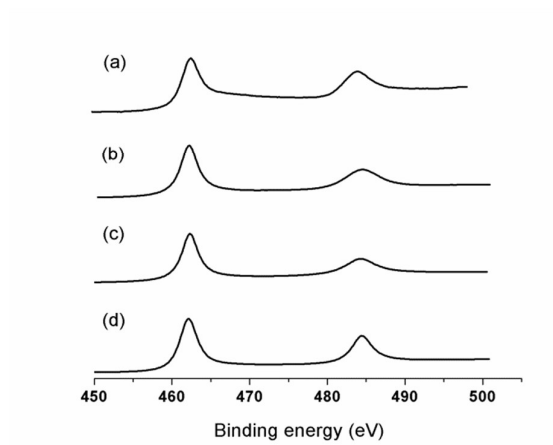
Fig. 3 XPS spectra of Ru 3p of the fresh and recycled Ru/AC. (a) fresh; (b) used once; (c) used twice; (d) used thrice .
