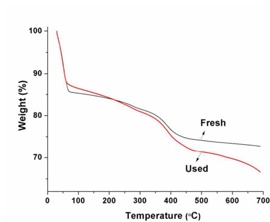
Fig. 6 TG curves of the fresh and used Ru/AC for the conversion of cellulose into EG under a N 2 atmosphere.
