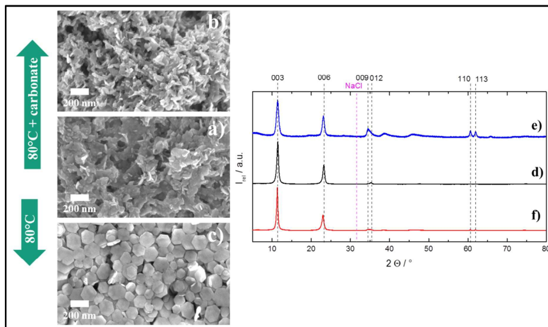
Figure 10. LDH nanoparticles, precipitated at low salt and NaOH concentrations (a) turn into slightly more defined platelets upon recrystallization in presence of carbonate (b). Remarkably, however, they turn into perfect hexagonal platelets when recrystallized without carbonate (c). Respective XRDs: d) corresponds to a), e) to b) and f) to c).
