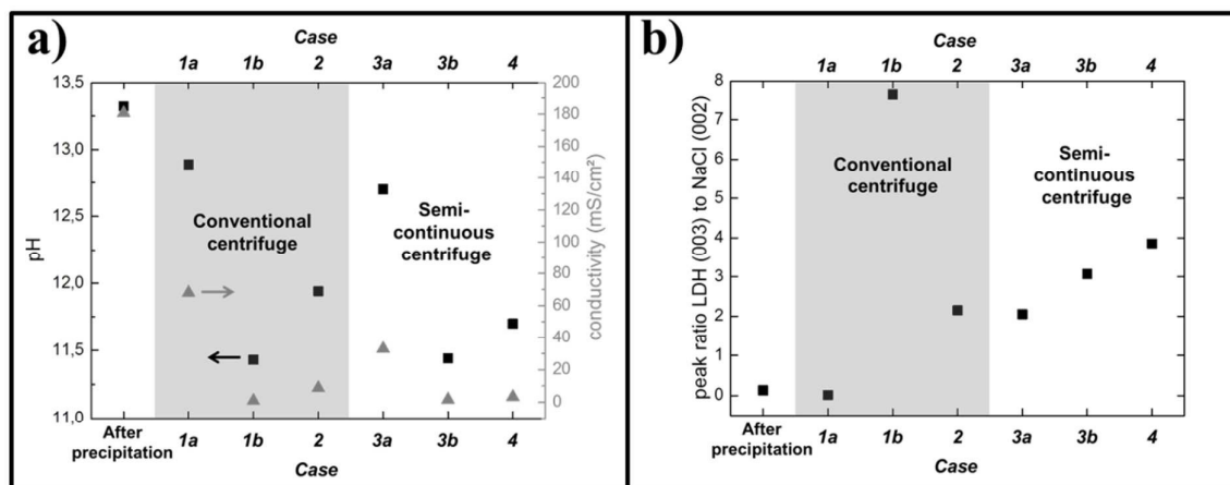
Figure 4a. Resulting pH and conductivity values for the cases 1-4 . Figure 4b. Resulting intensity ratios of LDH (003) to NaCl (002) XRD peaks.
