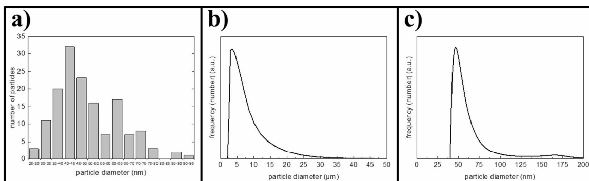
Figure 6. Size distribution of nano LDH determined from SEM images (Figure 6a) compared to size distribution of as-precipitated particle agglomerates in dispersion obtained via Fraunhofer diffraction (Figure 6b) and redispersed from the gel which was harvested from the centrifuge, obtained via DLS (Figure 6c).
