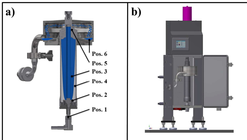
Figure 3. (a) Working principle and (b) sketch of the tubular centrifuge used for down-stream processing.
