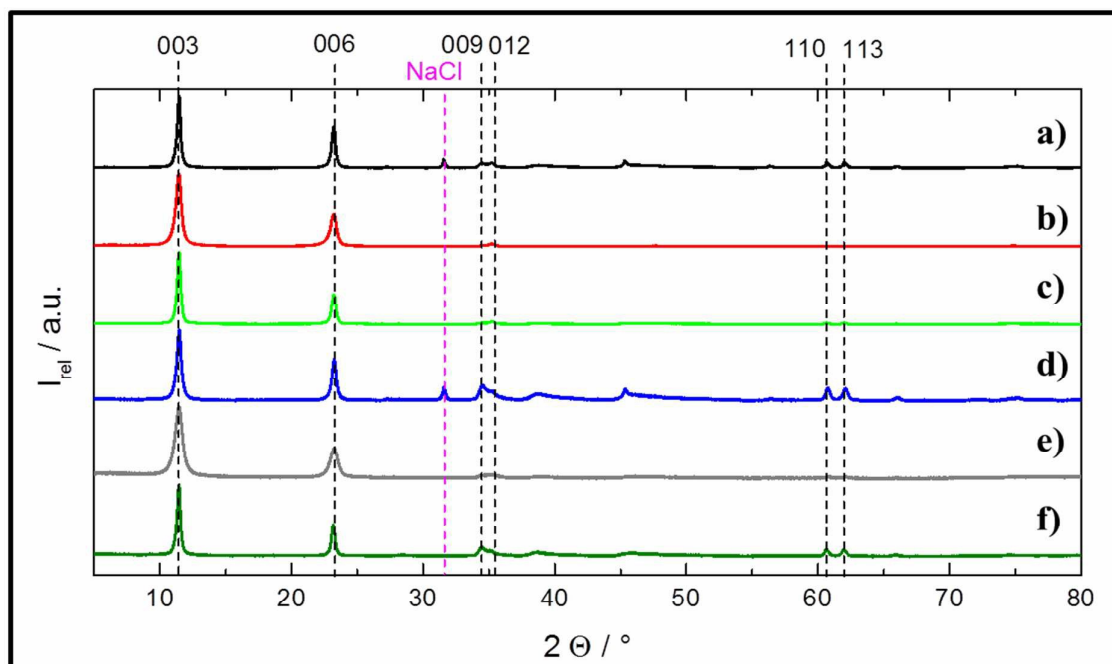
Figure 8. X-ray diffractograms of the samples, depicted in SEM in Figure 7. The numbering a)-f) corresponds to the equivalent samples as they are depicted in Figure 7. All XRDs are normalized in intensity with respect to the (003) peak.
