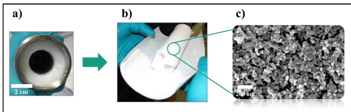
Figure 5. 144 g of nano-LDH, harvested from the cylinder (Figure 5a) of the semi-continuous centrifuge keeping the cylinder body shape as a rigid gel (Figure 5b). Figure 5c. SEM image of the LDH nanoparticles.
