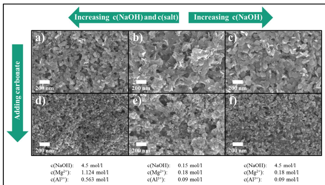
Figure 7. SEM images of the obtained LDH particle morphology for different concentrations of reactants during continuous precipitation without (a-c) and with (d-f) deliberately added carbonate during precipitation.
