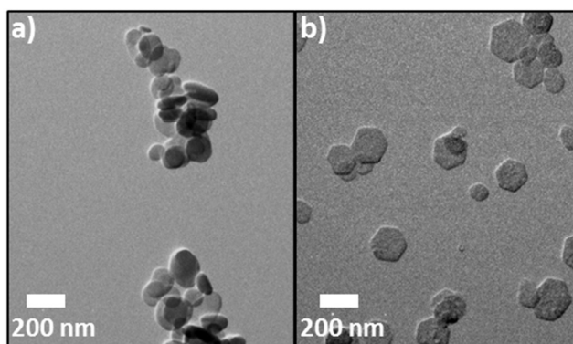
Figure 11. Two distinct morphologies of nano-LDH can be obtained with the process reported herein: a) rather round shaped particles and b) well-defined hexagonal platelets with sharp edges.
