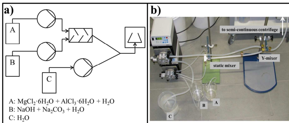
Figure 2. (a) Schematic process flowsheet of the continuous LDH synthesis with (b) the corresponding photograph of the setup.
