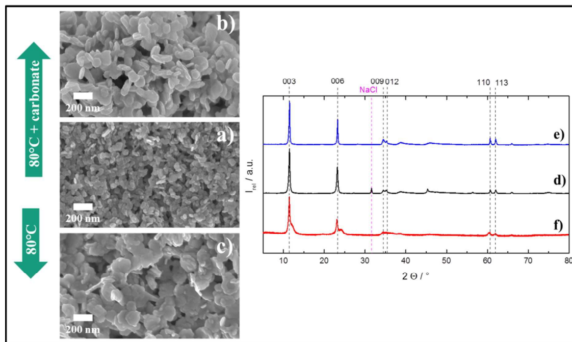
Figure 9. Initially rather spherically shaped LDH nanoparticles (a) transform to particles with slightly more platelet-like morphologies when recrystallized. Apparently, carbonate presence has no significant influence (b) with, c) without carbonate). The respective XRDs are rather similar for all cases (d) corresponds to a), e) to b) and f) to c).
