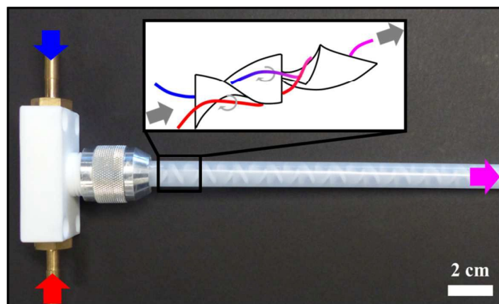
Figure 1. Photograph of the static mixer used in this work along with a schematic depiction of the spiral mixing elements.
