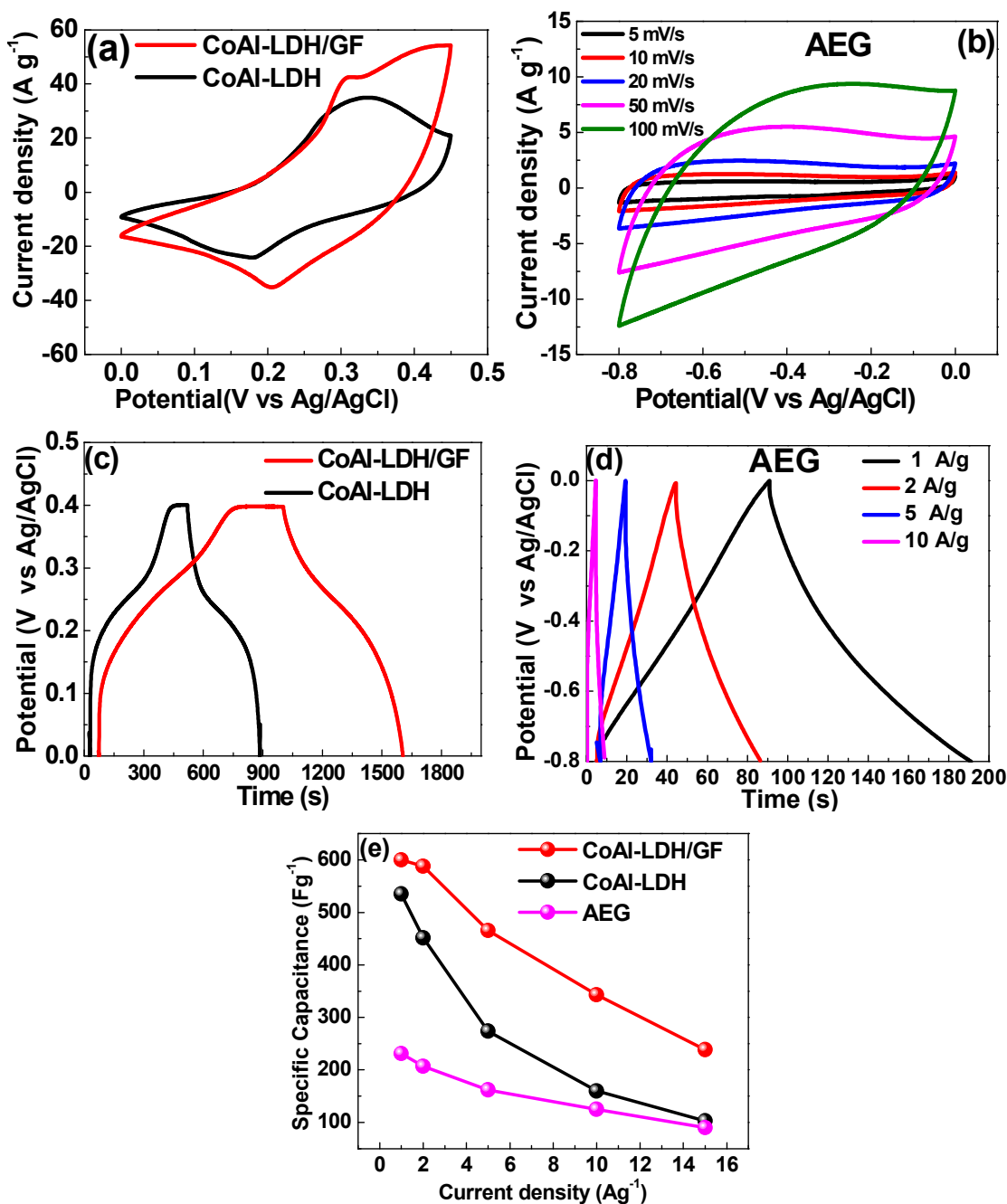
Figure 5: (a) Cyclic voltammety comparison at scan rate of 50 mVs -1 and (b) Cyclic voltammety at scan rates of 5-100 mV s -1 ; (c) Galvanostatic charge–discharge comparison at current density of 1 A g -1 , (d) Galvanostatic charge–discharge at current densities of 1 - 10 A g -1 and (e) specific capacitance versus current densities of the of CoAl-LDH ,CoAl-LDH/GF composite and AEG respectively.
