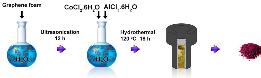
Scheme 1. Preparation of CoAl-LDH/GF
