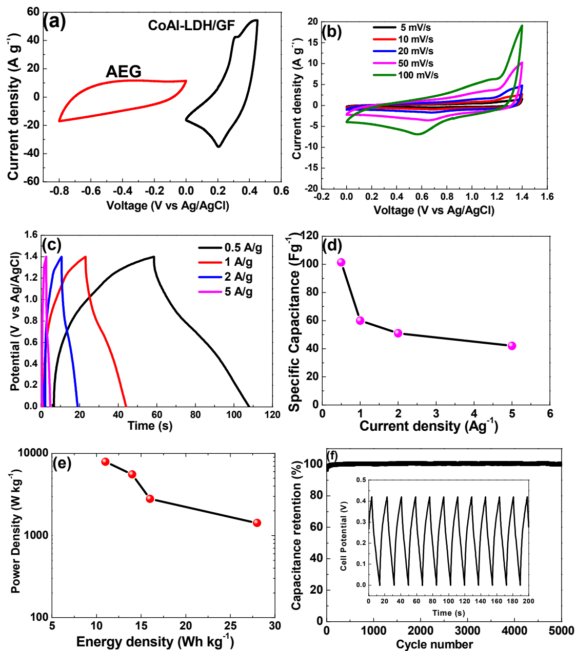
Figure 6: (a) Cyclic voltammetry of CoAl-LDH/GF and AEG electrodes at scan rates of 50 mV s -1 for three-electrode setup; asymmetric CoAl-LDH/GF//AEG device (b) Cyclic voltammetry at scan rates of 5 – 100 mV s -1 , (c) Galvanostatic charge–discharge at current densities of 0.5- 5 A g -1 and (d) the specific capacitance as function of the current density, (e) Ragone plot and (f) cycle stability at a constant current density of 0.5 A g -1 (inset shows charge – discharge curves after 200 circles) respectively.
