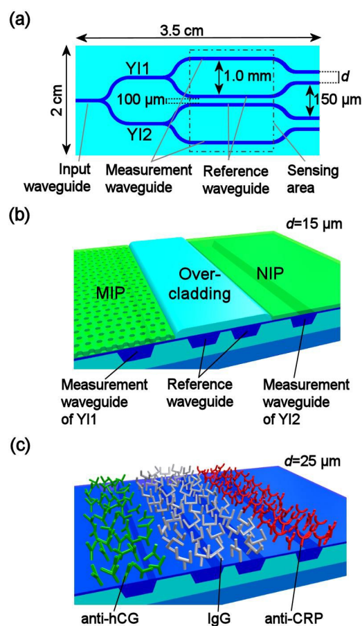
Fig. 1 (a) Top view illustration of the sensor chip with names of the parts and dimensions. (b) Illustration of the cross-cut structure of the MIP functionalised sensor chip within the sensing area showing the MIP and NIP coatings on the respective measurement waveguides, and the passivating overcladding layer on the reference waveguides. (c) Antibody functionalized chip having analyte specific anti-hCG and anti-CRP antibody coatings on the respective measurement waveguides and reference IgG coating on the reference waveguides. The separations of the measurement and the reference waveguides at the outcoupling end of the chip, d , are shown next to the sensor illustrations in (b) and (c).
