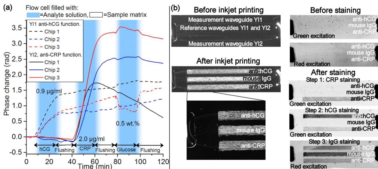
Fig. 8 (a) Phase change curves showing the specific responses of Y11 (dashed lines) and Y12 (solid lines) to hCG and human CRP samples, respectively. Responses to glucose solution demonstrate the sensor sensitivity to ambient RI changes. (b) Left: Microscope images of the YI chip before and after the antibody functionalization by inkjet printing showing the printed areas on top of the waveguides. Printed areas are visible due to the salts in the bio-inks that dry onto the chip surface. Right: Verification of specific binding of analytes onto the inkjet printed areas by fluorescent staining and imaging. The fluorescence images (the darker the colour the higher the fluorescence intensity) taken before staining show no fluorescence from the printed areas. After each staining step, the corresponding inkjet printed area became fluorescent verifying the localized presence of the analytes and the reference IgG coating.
