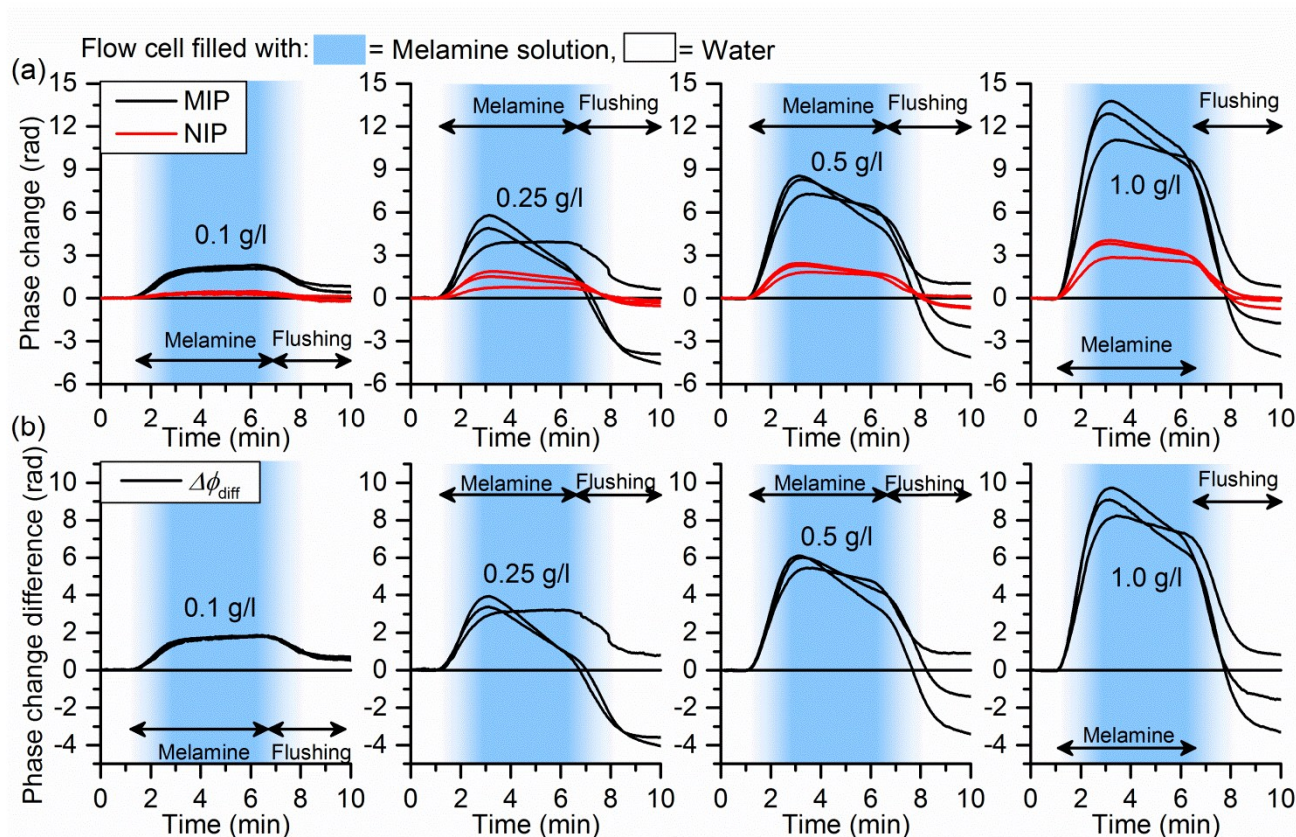
Fig. 5 (a) Phase change curves of MIP functionalized Y11 and NIP coated Y12 measured at various melamine concentrations. Each concentration (value shown next to the curves) was measured three times. (b), \Delta\phi_{\text{diff}} curves showing the net difference of the phase change values between the MIP functionalized Y11 and NIP functionalized Y12 at different melamine concentrations. Timing of the solutions in the flow cell is indicated by the arrows and the background colour.
