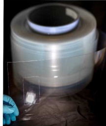
Roll of sensor waveguides
