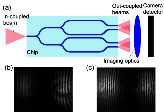
Fig. 2 (a) Schematic illustration of the experimental arrangement. Captured interferogram of (b) MIP functionalized, and (c) antibody functionalized sensor chip.
