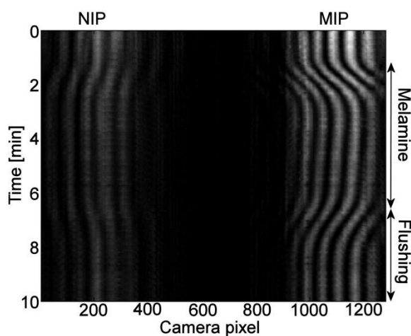
Fig. 6 Shift of the interferogram fringes during a chemical sensing experiment conducted with the melamine concentration of 1.0 g/l. Figure is constructed by first selecting the same narrow section (height 5 pixels) across each of the time laps images captured during the experiment, and then combining these sections.
