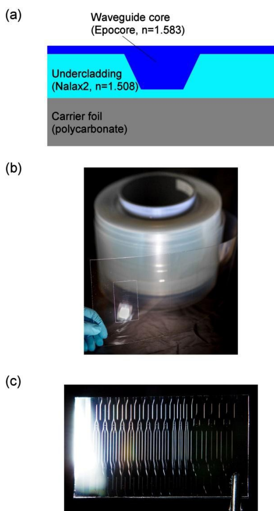
Fig. 3 (a) Schematic of the cross-section of the inverted ridge waveguide structure showing the materials and the refractive indices 14 , n , of the core and undercladding layers at the wavelength of 975 nm, i.e. at the wavelength used in the sensing experiments. (b) Roll of sensor waveguides. (c) Sensor platform cut from the roll.
