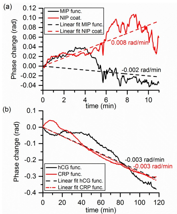
Fig. 4 Phase change curves measured while the sample matrix flowed in the flow cell, and lines fitted to the data points for a) MIP functionalized chip (image interval 2 s), and b) for antibody functionalized chip (image interval 30 s). The slope of the fitted lines is also shown indicating the trend of the system drift.
