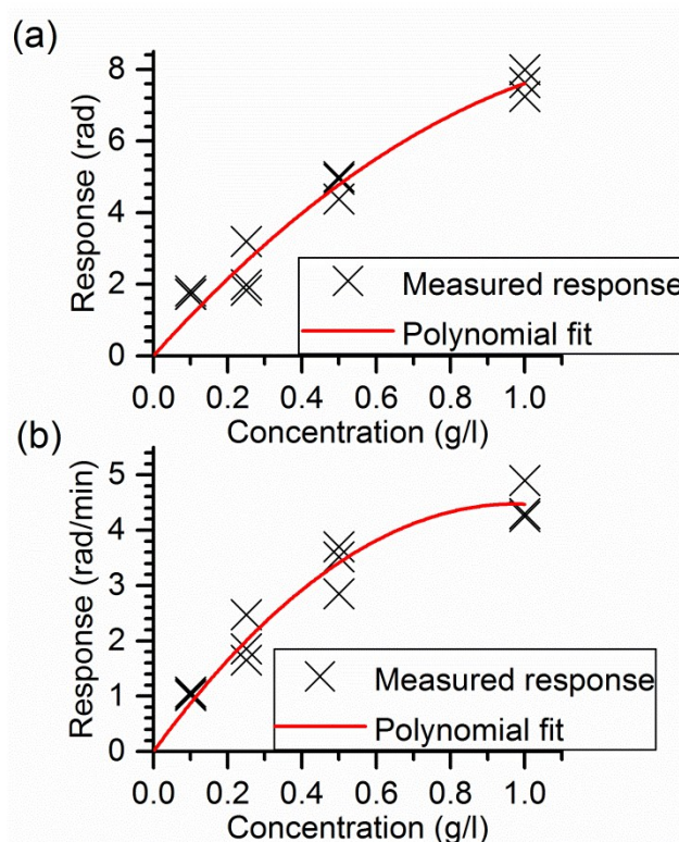
Fig. 7 Calculated responses and lines fitted to the data points based on (a) the phase change step height, and (b) the slope of the rising edge of \Delta\Phi_{diff} curves.
