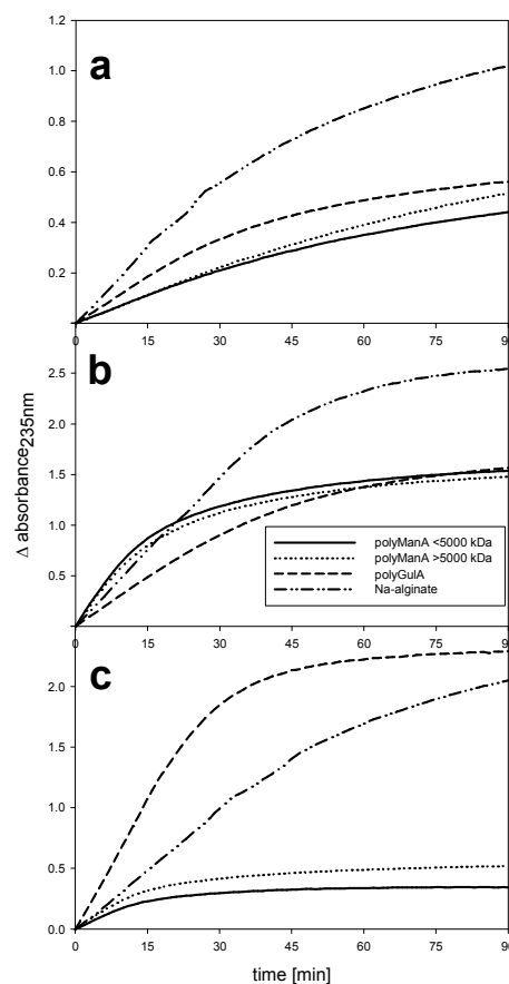
Figure 3: Substrate specificity of alginate lyases: SALy (a), FALy (b), and SigMAlY (c) on poly-mannuronic acid < 5000 kDa, poly-mannuronic acid > 5000 kDa, poly-guluronic acid and sodium alginate at S/V 0.2 %, pH 7 and 40 °C recorded as \Delta\text{absorbance}_{\epsilon=235\text{ nm}} over the first 90 min of reaction. Enzyme dosages E/S were 0.1 % for SALy and SigMAlY, and 0.03 % for FALy.
