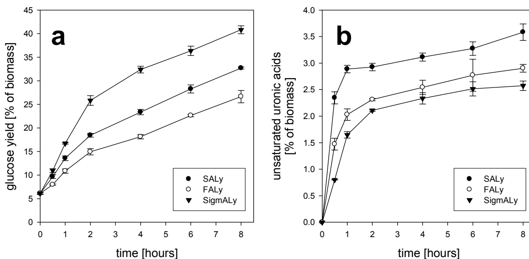
Figure 4: (a) Glucose yields in % of dry biomass in response to enzymatic treatment; (b) alginate degradation products of unsaturated uronic acid residues in % of dry biomass of refiner milled wet Laminaria digitata . Enzymatic saccharification with Cellic CTec2 concentration of 10 % v/w and alginate lyase (SALy, FALy and purchased lyase SigmALy) of 1 % w/w over time with measurements at timepoints 0, 0.5, 1, 2, 4, 6 and 8 hours. Each data point represents the average value of independent duplicates; vertical bars indicate the standard deviation.
