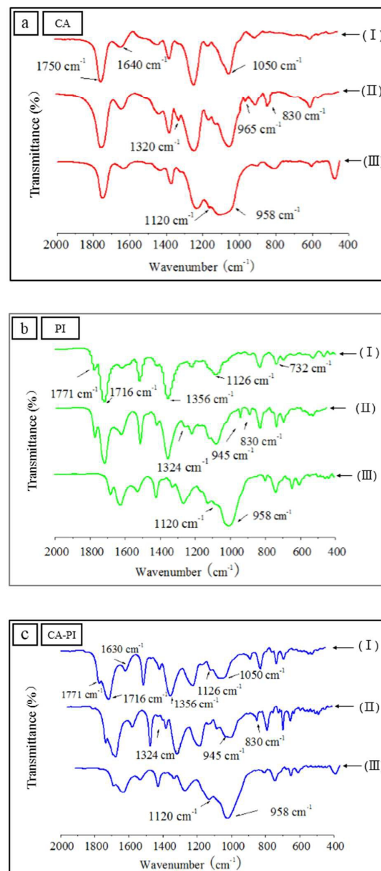
Fig. 4 FT-IR spectrograph of (a) CA, (b) PI and (c) CA-PI membranes. (I), (II) and (III) correspond to respectively pristine fibrous
