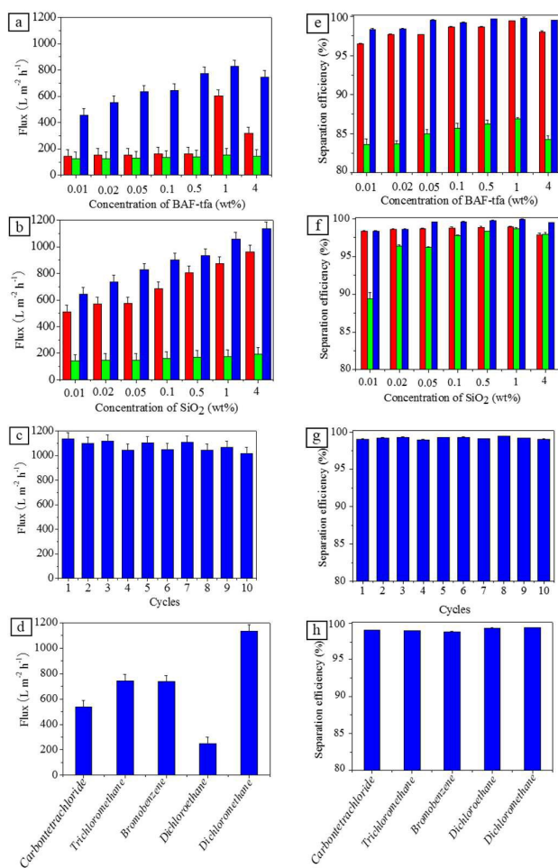
Fig. 9 (a-c) Flux of dichloromethane (DCM) through electrospun CA-PI (□), PI- (□) and core-sheath structured CA-PI (□) nanofibrous membranes. (d) Flux of various oil-water mixtures through F-PBZ-1/SNP-4/CA-PI membranes. (e-g) Separation efficiency of the membranes for dichloromethane-water mixtures. (h) Separation
