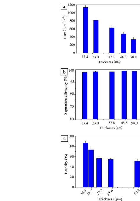
Fig. 10 (a) Flux of DCM through F-PBZ-1/SNP-4/CA-PI nanofibrous membranes with different thickness. (b) Separation efficiency of these membranes for dichloromethane-water mixtures and their porosity (c).
