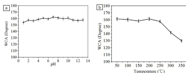
Fig. 11 WCAs of F-PBZ-1/SNP-4/CA-PI membranes. (a) in function of the pH of the water in the oil-water mixtures and (b) after calcination at different temperatures in air (for 10 min).
