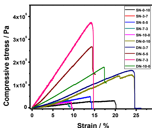
Fig. 5. a) Compressive stress-strain curves of the SN and DN hydrogels. b) Elastic modulus, the maximum of compressive stress and strain obtained from compressive stress-strain curves. Elastic
