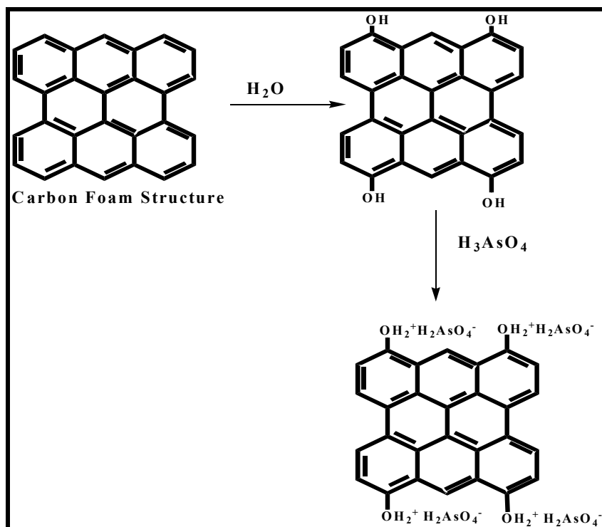
Figure 3: schematic diagram of chemical interaction between carbon foam and As (V)
