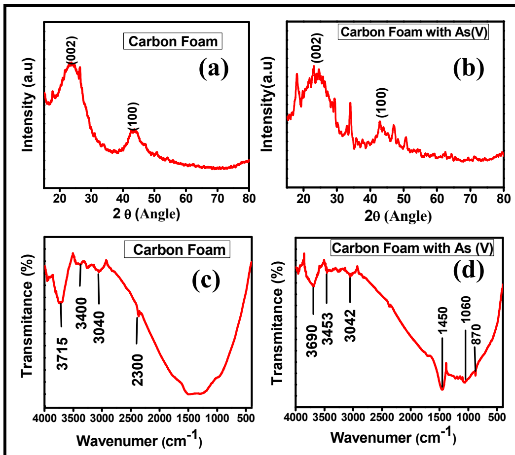
Figure 5: (a), (b) XRD spectra and (c), (d) FTIR spectra of carbon foam before and after As (V) adsorption respectively
