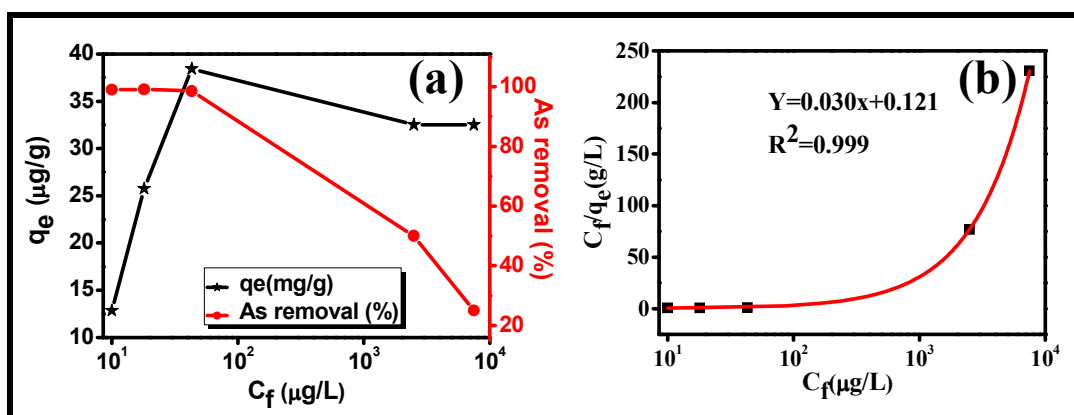
Figure 8: (a) Effect of remaining concentration of As (V) on adsorption capacity of carbon foam, and (b) Langmuir adsorption isotherm
