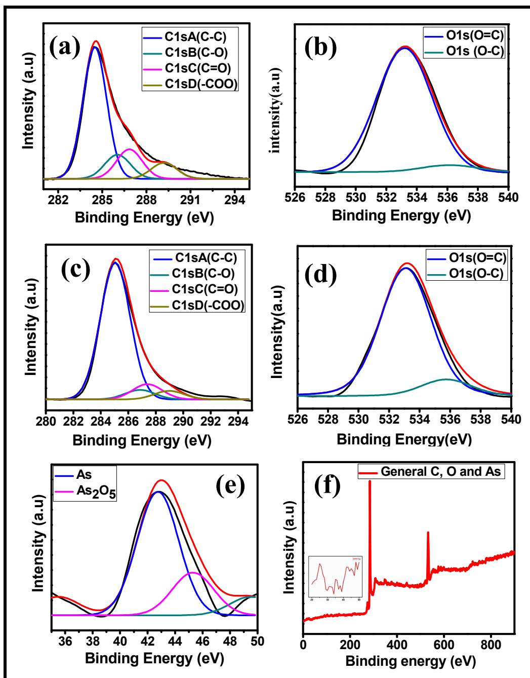
Figure 4: XPS spectra of carbon foam before As (V) adsorption (a-b) and (c-f) after As (V) adsorption
