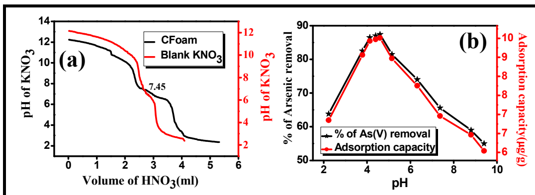
Figure 2: (a) pHPzc and (b) Effect of pH on arsenic (V) adsorption capacity
