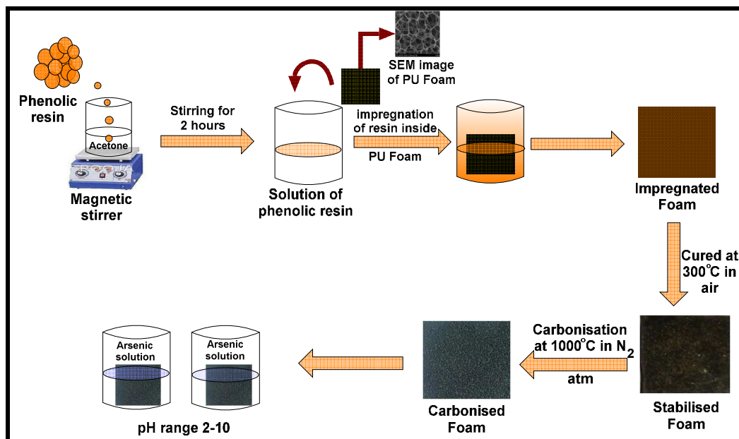
Figure 1: Schematic diagram shows the fabrication process of carbon foam for the removal of As (V)
