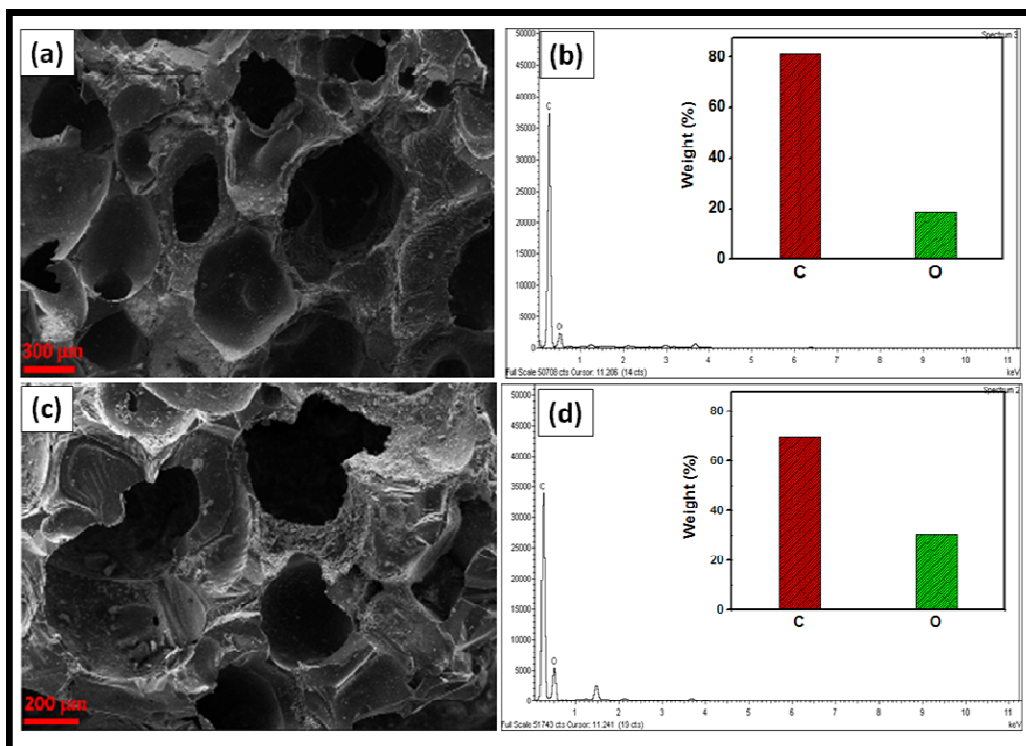
Figure 10: SEM and EDX of used carbon foam (a) & (b) after treated with EDTA, (c) & (d) after treated with HNO 3
