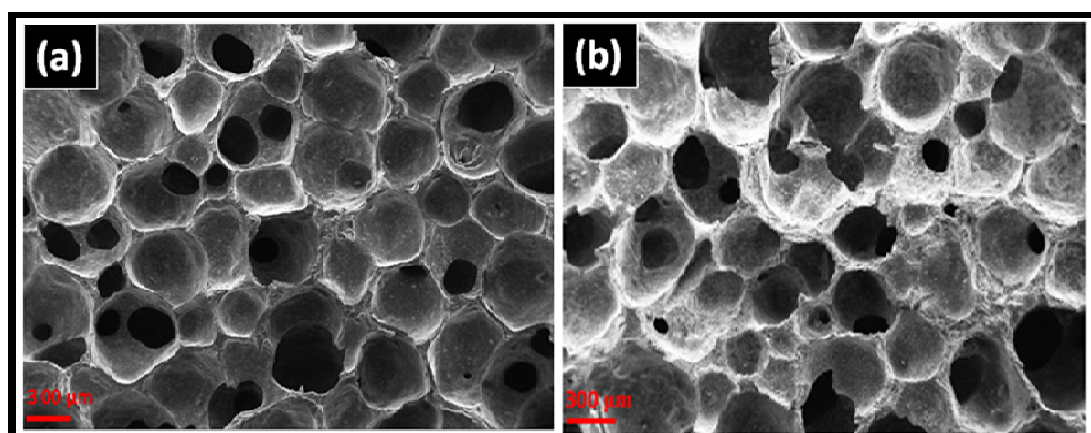
Figure 6: SEM images of (a) pristine carbon foam, (b) after As (V) adsorption
