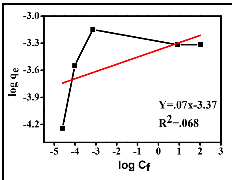
Figure 9: Freundlich adsorption isotherm
