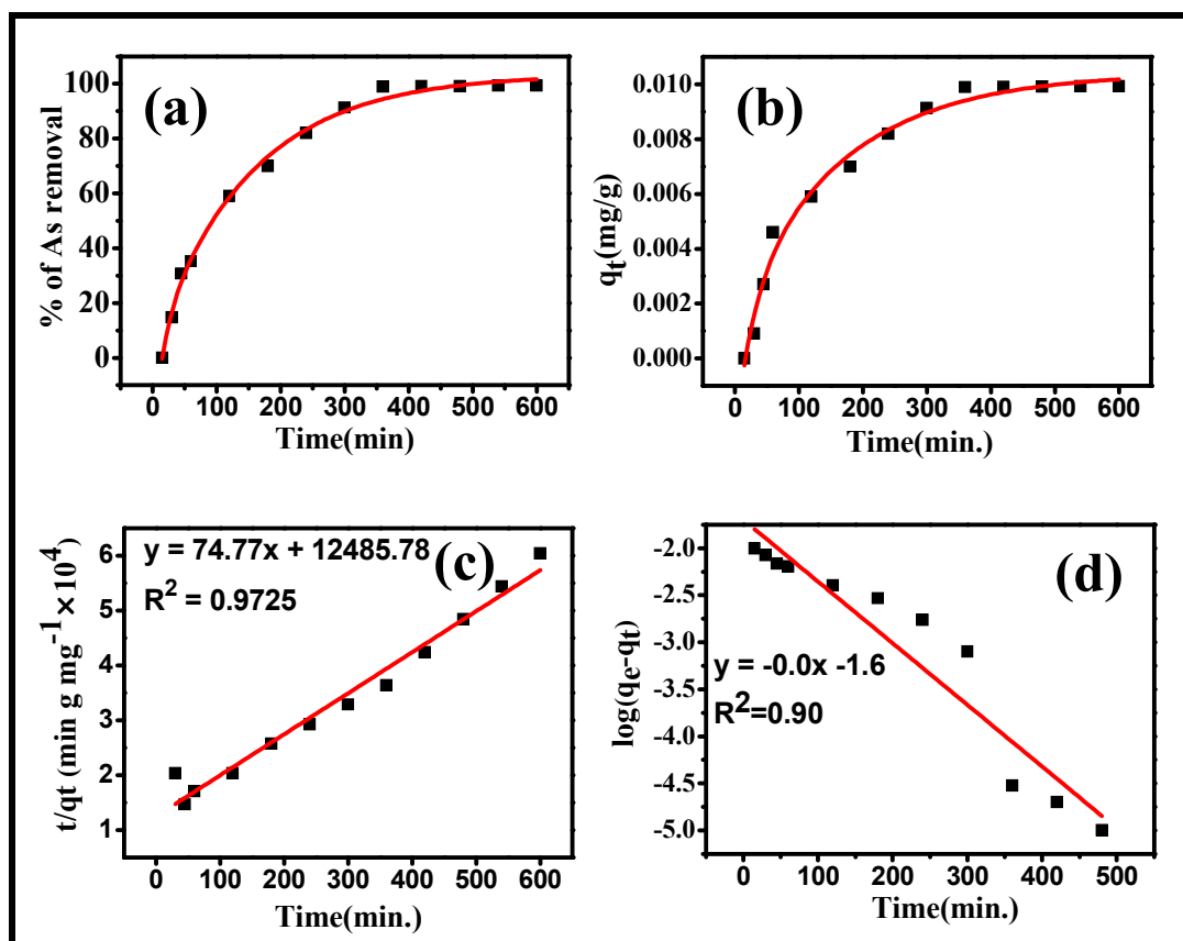
Figure 7: Effect of time on (a) As (V) removal, (b) adsorption capacity ( q_t ) of As (V), (c) pseudo second order kinetics and (d) pseudo first order kinetics
