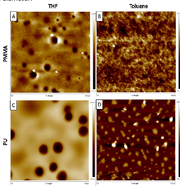
Fig. 2 AFM height images of PMMA- or PU-only surfaces cast from toluene or THF. A) Surface A; B) surface C; C) surface B; D) surface D, as described in Table 1. Images are 5 \times 5 \mu\text{m} .
