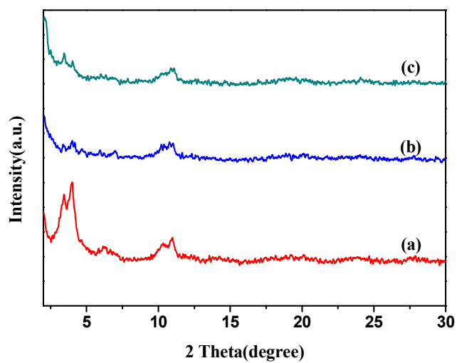
Fig.1. XRD patterns of (a) MIL-100(Fe), (b) MIL-100(Fe)@DAILs, and (c) recovered MIL-100(Fe)@DAILs.
