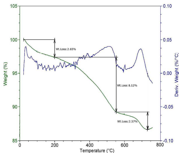
Fig. 5. TGA-DTA analysis of \text{Fe}_3\text{O}_4@\text{nSiO}_2@\text{mSiO}_2@\text{Pr-Imi-NH}_2
