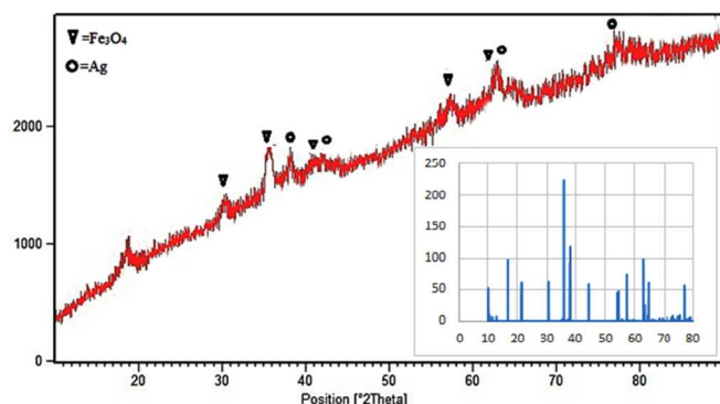
Fig. 2 The X-ray diffraction pattern for \text{Fe}_3\text{O}_4@ \text{nSiO}_2@ \text{mSiO}_2@ \text{Pr-Imi-NH}_2 .Ag
