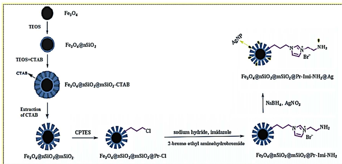
Scheme 1. Schematic illustration of the steps in the synthesis of \text{Fe}_3\text{O}_4@ \text{nSiO}_2@ \text{mSiO}_2/\text{Pr-Im-NH}_2\text{-Ag}
