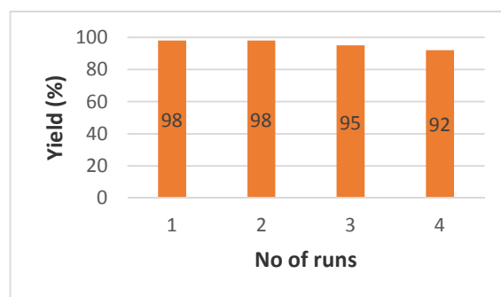
Fig. 7. Recyclability of \text{Fe}_3\text{O}_4@ \text{nSiO}_2@ \text{mSiO}_2@ \text{Pr-Imi-NH}_2\text{.Ag} in the nitrobenzene reduction in water after 40 min
