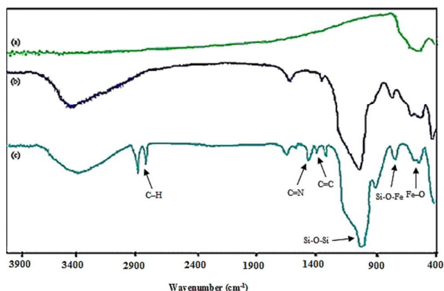
Fig. 1 The FT-IR spectra of (a) \text{Fe}_3\text{O}_4 , (b) \text{Fe}_3\text{O}_4@ \text{nSiO}_2@ \text{mSiO}_2 , (c) \text{Fe}_3\text{O}_4@ \text{nSiO}_2@ \text{mSiO}_2@ \text{Pr-Imi-NH}_2
