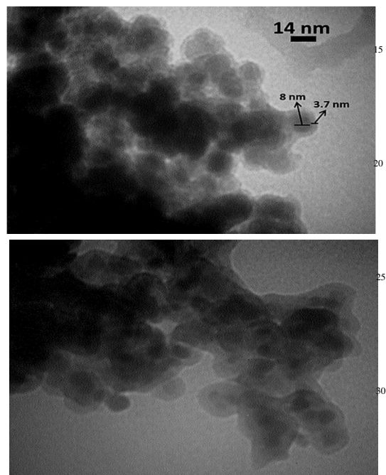
Fig. 4. TEM images of \text{Fe}_3\text{O}_4@\text{nSiO}_2@\text{mSiO}_2@\text{Pr-Imi-NH}_2 Ag Core-Shell nanostructures.
