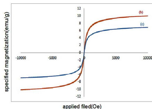
Fig. 3. VSM magnetization curves of the \text{Fe}_3\text{O}_4 (a), \text{Fe}_3\text{O}_4@ \text{nSiO}_2@ \text{mSiO}_2/ \text{Pr-Imi-NH}_2 (b) and \text{Fe}_3\text{O}_4@ \text{nSiO}_2@ \text{mSiO}_2/ \text{Pr-Imi-NH}_2 .Ag (c) nanoparticles
