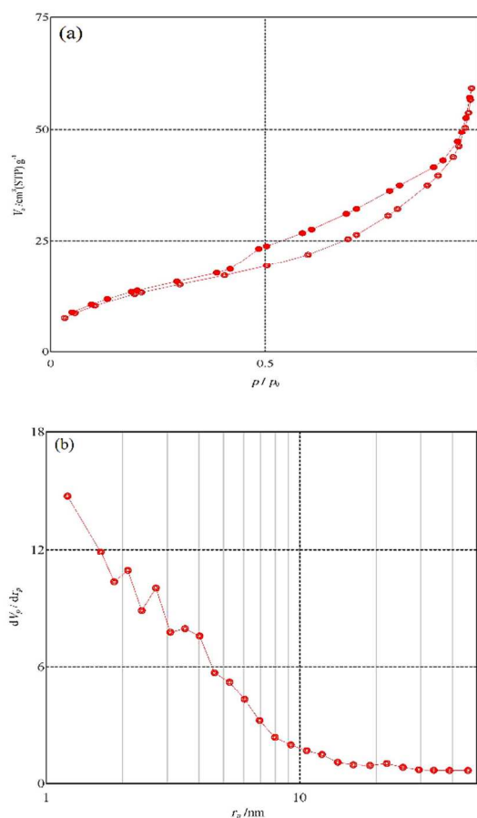
Fig. 6. Nitrogen adsorption-desorption (a) and Pore size distributions (b) isotherms of \text{Fe}_3\text{O}_4@\text{nSiO}_2@\text{mSiO}_2@\text{Pr-Imi-NH}_2
