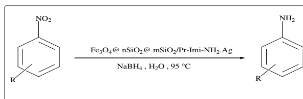
Scheme 2. Reduction of the nitroarenes
