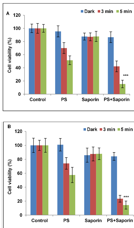
Figure 6. Light-induced cytotoxic response for 19 (A) and 26 (B) in MC28 cells, showing PDT (without saporin) and PCI (with saporin) effects. Cells were incubated with photosensitiser (50 nM) with or without saporin (20 nM) for 18 h. Irradiation was carried out for 3 and 5 min with a blue lamp. MTT assay was carried 72 h after irradiation. The experiments were repeated 3 times, and representative data are shown. Error bars = SD. Statistically significant difference between PCI conjugate 19-saporin versus PDT conjugate 19 ( p < 0.0001 ) is indicated by ***. Likewise, statistically significant difference between PCI conjugate 26-saporin versus PDT conjugate 26 ( p < 0.0001 ) is indicated by ***.
