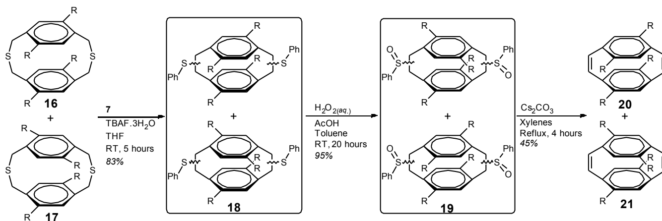
Scheme 4. Synthesis of [2.2]paracyclophane-1,9-dienes 20 and 21 , R = n -octyl.
