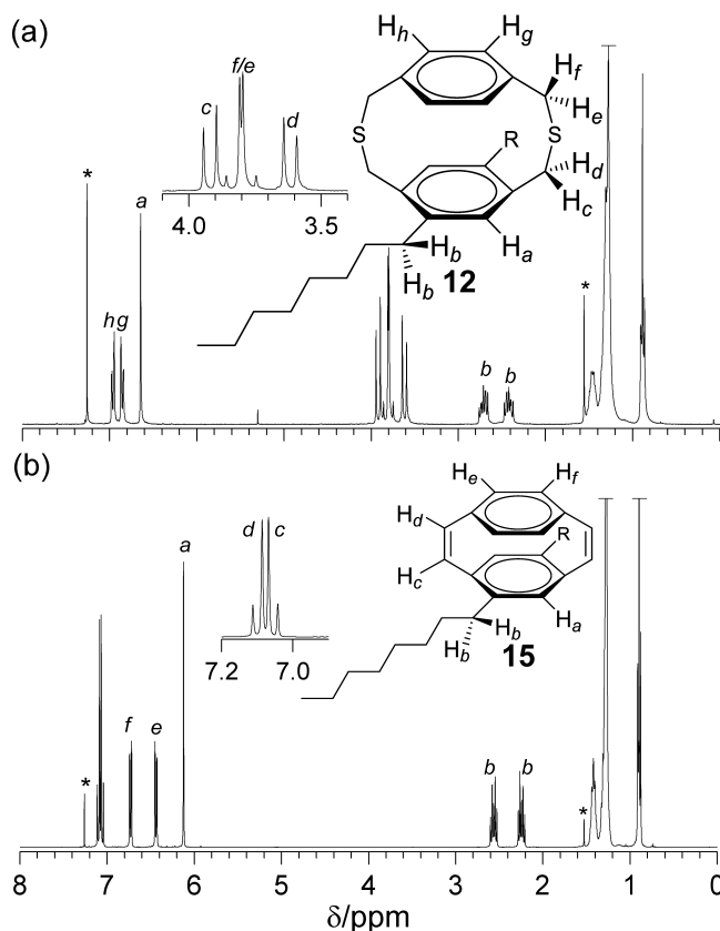
Figure 1. 1 H NMR spectra (CDCl 3 ) of (a) dithia[3.3]paracyclophane 12 and (b) [2.2]paracyclophane-1,9-diene 15 .
