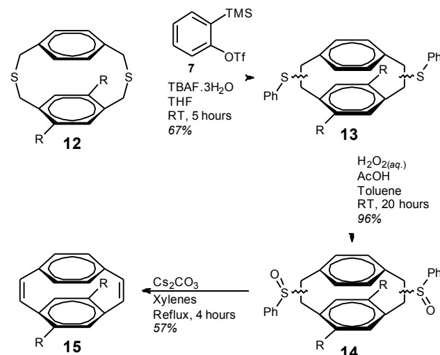
Scheme 3. Synthesis of [2.2]paracyclophane-1,9-diene 15 , R = n -octyl.
