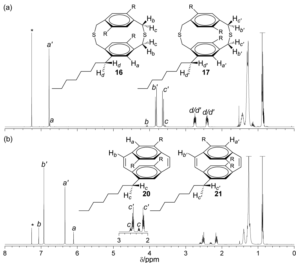
Figure 2. ^1\text{H} NMR spectra ( \text{CDCl}_3 ) of (a) dithia[3.3]paracyclophanes 16 and 17 , and (b) [2.2]paracyclophane-1,9-dienes 20 and 21 , R = n\text{-octyl} .
