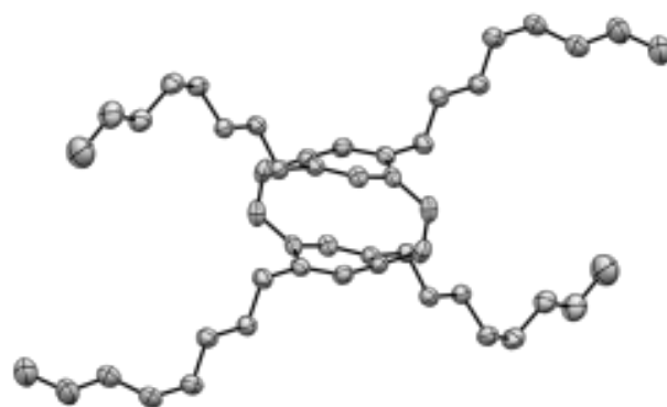
Figure 3. Solid-state structure of 20 as ORTEP plot. Hydrogen atoms are omitted for clarity.
