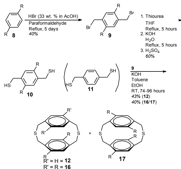
Scheme 2. Synthesis of dithia[3.3]paracyclophanes; 12 , 16 and 17 , R = n -octyl.
