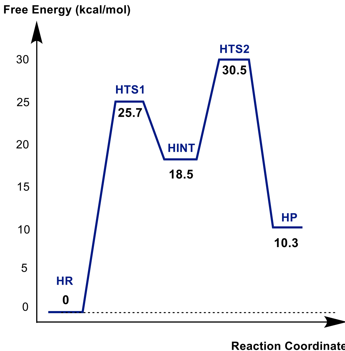
Fig. 6 Free energy profile diagram along intrinsic reaction coordinate for hydrolysis of the Ser70-avibactam bond in the CTX-M-15 active site. Free energy is measured from reactant complex ( HR ) for each stationary-state structure using the MP2/6-31G* level of calculations. HTS1 , HINT , HTS2 , and HP represent the first transition state, reaction intermediate, second transition state, and final energy minimum, respectively, during the hydrolysis reaction.
