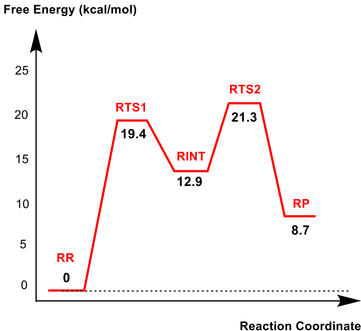
Fig. 4 Free energy profile diagram along intrinsic reaction coordinate for the recyclisation to give avibactam from the covalent complex with CTX-M-15. Free energy is measured from reactant complex (RR) for each stationary-state structure using the MP2/6-31G* level of calculation. RTS1 , RINT , RTS2 , and RP represent the first transition state, reaction intermediate, second transition state, and final energy minimum, respectively, during the recyclisation reaction.
