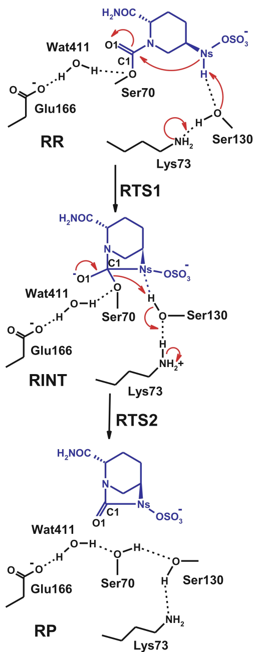
Fig. 3 Possible fates for reaction of the CTX-M-15 avibactam covalent complex: (a) recyclisation, and (b) hydrolysis. RR and HR , RTS1 and HTS1 , RINT and HINT , RTS2 and HTS2 , and RP and HP denote the reactive complex, first transition state, reaction intermediate, second transition state, and final energy minimum, respectively, during the recyclisation and hydrolysis reactions, respectively.
