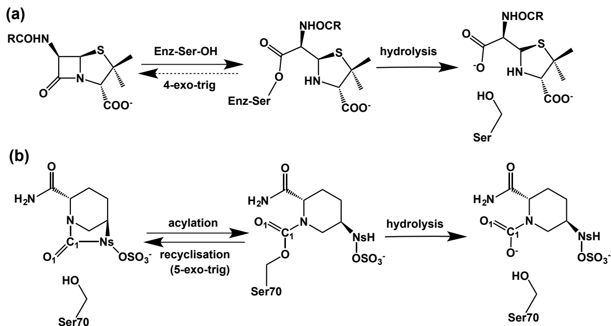
Fig. 1 \beta -Lactams react irreversibly with penicillin binding proteins/ \beta -lactamases nucleophilic enzymes to form an acyl-enzyme complex in contrast to avibactam which reacts reversibly. (a) Irreversible reaction of a \beta -lactam with nucleophilic serine enzyme as exemplified by reaction of a penicillin with a penicillin binding protein (transpeptidase) to give a stable acyl-enzyme complex, which only undergoes slow hydrolysis; (b) Schematic representation of the acylation, recyclisation, and hydrolysis reactions between a serine \beta -lactamase and avibactam.
