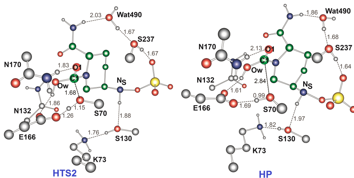
Fig. 7 Calculated structures of the energy minima and transition states for hydrolysis of the avibactam derived acyl-enzyme complex in the CTX-M-15 active site. Selected interatomic distances are given in Å. HR , HTS1 , HINT , HTS2 , and HP represent the reactive complex, first transition state, reaction intermediate, second transition state, and final energy minimum, respectively, during the hydrolysis reaction.
