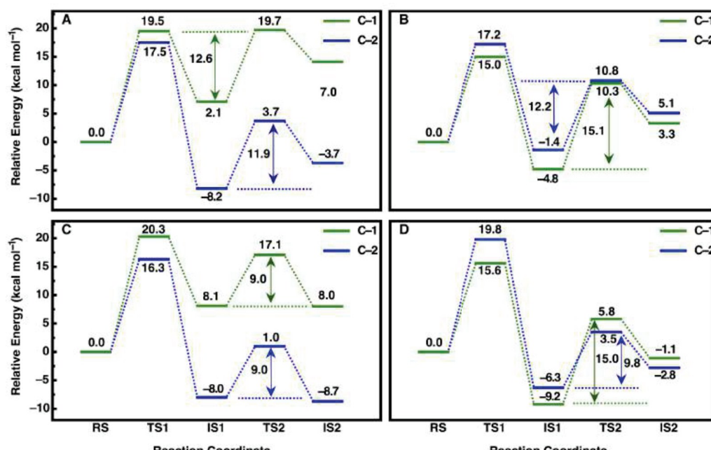
Figure 7: Calculated free energy profiles (kcal mol -1 ) for the hydrolysis of (A, C) ( R )- and (B, D) ( S )-SO by (A, B) wild-type StEH1 and (C, D) the R-C1B1 variant in the binding mode with the lowest activation free energies for each enantiomer respectively (for the corresponding activation free energies see Table 3 ). RS, TS1, IS1, TS2 and IS2 indicate the Michaelis complex (RS), the transition state for the alkylation step (TS1), the resulting alkylenzyme intermediate (IS1), the transition state for the hydrolysis step (TS2) and the tetrahedral intermediate (IS2). For details of the overall reaction mechanism see Figure 1 . All values above or below each reacting state show the calculated free energy relative to the Michaelis complex, and the values next to each arrow show the calculated activation free energy of the hydrolysis step relative to the energy of the alkylenzyme intermediate.
