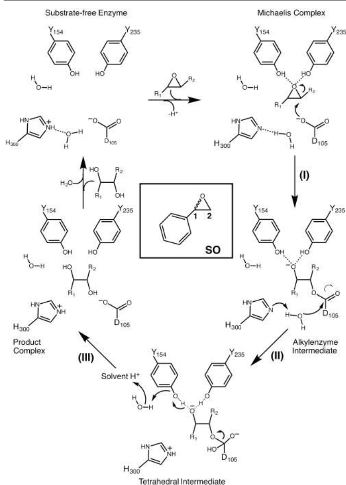
Figure 1: Schematic overview of a generalized mechanism for the reaction catalysed by potato epoxide hydrolase 1 (StEH1). Highlighted in particular here are (I) the alkylation step, involving nucleophilic attack of the side chain of D105 on one of the carbon atoms of the bound epoxide; (II) hydrolysis of the resulting alkyl-enzyme intermediate by an active site water molecule to yield a tetrahedral intermediate, and (III) breakdown of the tetrahedral intermediate, leading to release of the product diol from the active site. The structure of styrene oxide (SO) is also highlighted in the inset box. This figure is adapted from ref. 17 .
