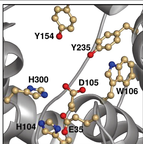
Figure 2: An overview of key active site residues in the unequilibrated substrate-free form of wild-type StEH1 based on a 1.95Å-resolution crystal structure of the enzyme 6 (PDB ID: 2CJP).
