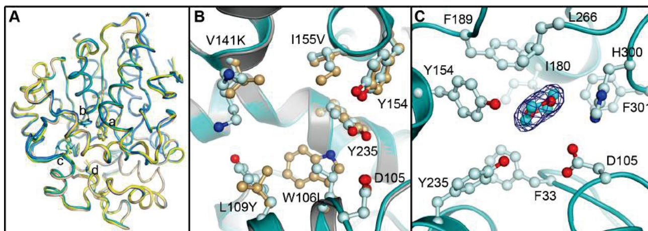
Figure 9: Crystal structure of the R-C1B1 variant of StEH1. Shown here are: (A) Superimposed C_{\alpha} -traces of the two subunits of wild-type StEH1 (PDB-ID: 2CJP) and the R-C1B1 variant (PDB-ID: 4UFN) present in the asymmetric unit of the respective crystals, coloured yellow and wheat for the wild-type enzyme, and teal and marine for the variant. The locations of amino acid exchanges are marked by a (W106L), b (L109Y), c (V141K), d (I155V), and * (P94L). (B) A zoom-in on the superimposed active sites of wild-type StEH1 (grey cartoon) and R-C1B1 (blue cartoon), showing the side chains of the two lid tyrosines, the catalytic D105 as well as the sites of amino acid exchanges, with carbon atoms in gold for wild-type StEH1 and in light blue for the variant. (C) The dioxane binding site observed in R-C1B1. All side chains within or near van der Waals distance of the ligand are shown, coloured as in B. The carbon atoms of the dioxane are coloured in cyan. The final electron density observed for the dioxane is contoured at sigma levels of 1.0 for the 2F_o - F_c map (blue mesh), and 3.0 (green) and -3.0 (red) for the F_o - F_c map. Note that no sufficiently high density peaks are observed around the ligand in the latter.
