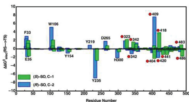
Figure 8: Overview of the electrostatic contributions of each individual residue and water molecule in our simulation systems to the overall calculated activation energy ( \Delta\Delta G^{\ddagger}_{\text{elec}} ) for formation of the alkylenzyme intermediate (energy of TS1 in Figure 7 ), during the hydrolysis of ( R )- and ( S )-SO by wild-type StEH1, following nucleophilic attack at C-1 for ( S )-SO (green bars) and C-2 for ( R )-SO (blue bars). Shown here are the preferred Mode 2 conformations for both substrates, and the red circles on the annotations denote water molecules. All energies are in kcal mol -1 , and were extracted from the EVB trajectories using the linear response approximation, as in our previous works 17, 34 .
