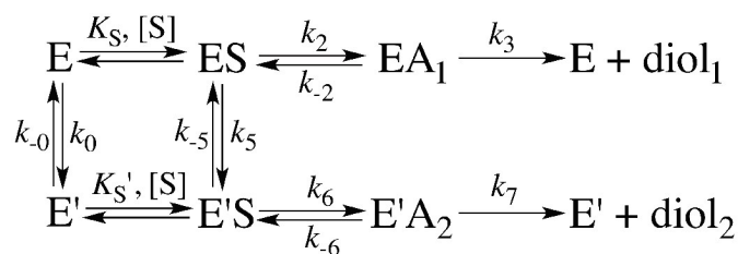
Scheme 1: Kinetic scheme for the StEH1 catalysed hydrolysis of different substrate enantiomers. E and E' denote the different enantiomers, ES and EA denote the Michaelis complex and the enzyme in complex with an alkylenzyme intermediate, and diol1 and diol2 denote the two product diols.
