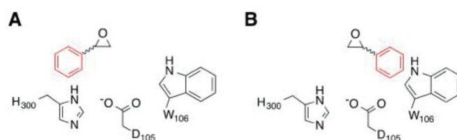
Figure 4: A schematic illustration of the two active site conformations of styrene oxide used in this work. Shown here are (A) Mode1 , where the phenyl ring forms a stacking interaction with the H300 side chain, and (B) Mode2 , where the phenyl ring interacts with the side chain of W106 in the wild-type enzyme (note that although the substrate conformation is retained in the R-C1B1 variant, W106 has been replaced by a leucine).
