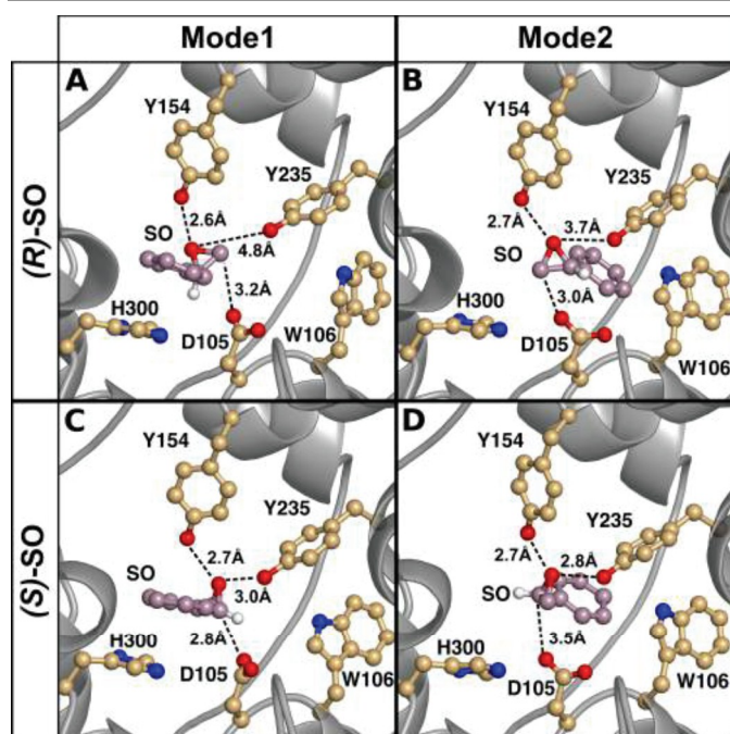
Figure 6: A comparison of representative structures of the Michaelis complexes obtained after molecular dynamics equilibration of wild-type StEH1 in complex with (A, B) (R)- and (C, D) (S)-SO, with the substrate placed in the active site in (A, C) Mode1 and (B, D) Mode2 respectively. The figure highlights the distance between the epoxide oxygen and the hydroxyl oxygens of Y154 and Y235, as well as the distance between the side chain of D105 for the preferred epoxide carbon for each enantiomer (C-1 for (S)-SO and C-2 for (R)-SO). The C-1 hydrogen has also been included in this figure to illustrate the stereochemistry. For discussion of the associated activation and reaction free energies of the different binding modes see the main text, and for structures of the corresponding transition states and intermediates for the first reaction step (formation of the alkyl-enzyme intermediate), see Figures S8 to S11 .
