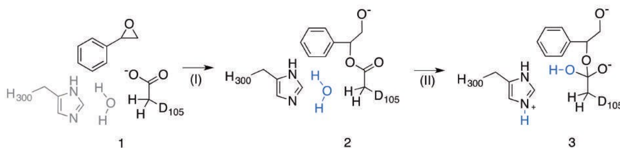
Figure 5: Overview of the valence bond states used to describe the StEH1 catalysed hydrolysis of styrene oxide (SO). Shown here are (1) the Michaelis complex, (2) the alkyl-enzyme intermediate and (3) the tetrahedral intermediate corresponding to (I) the alkylation and (II) hydrolysis steps of this reaction respectively. Note that the imidazole side chain and hydrolytic water molecule were not included in the reference EVB calculation of Step I . Additionally, the hydrolytic water molecule in step II has been highlighted in blue to follow the movement of protons. This figure has been adapted from ref. 17 .
