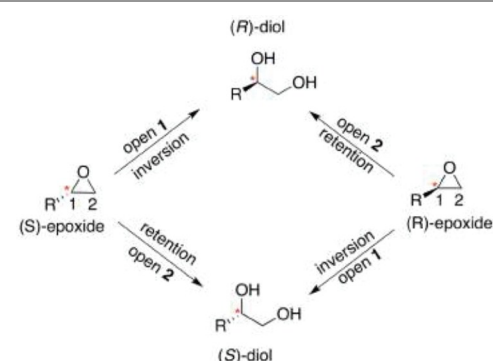
Figure 3: A schematic overview of the enantioconvergent hydrolysis of different enantiomers of an epoxide substrate to give the same product diol. In the present case, StEH1-catalyzed styrene oxide hydrolysis proceeds primarily through attack at C-1 for the (S)-enantiomer, and C-2 for the (R)-enantiomer, in contrast to the non-enzymatic hydroxide-catalyzed hydrolysis, where hydroxide addition at each of the two carbon atoms occurs with almost equal rates 19 .
