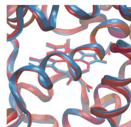
Figure 3: Superposition of the optimised structure of Cpd I (in blue) and the experimental structure of the resting state (in red). A zoom into the active site is depicted; for a view of the full structure see Figure S3 in the ESI.
