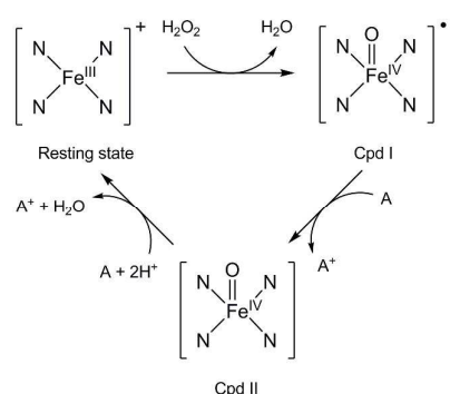
Figure 1: Catalytic cycle of lignin peroxidase. The four N atoms stand for the porphyrin ring and A is an electron-donating substrate.
