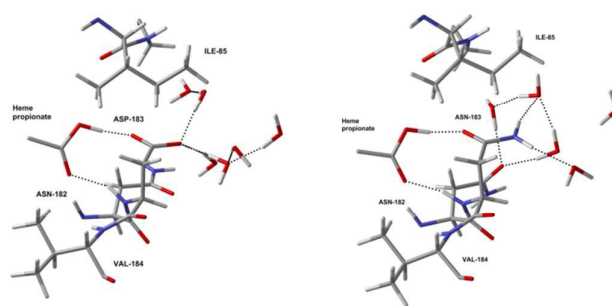
Figure 5: Optimised local structures of Cpd I (left) and the D183N mutant protein (right) around residue 183.
