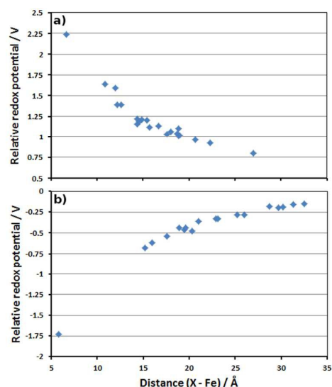
Figure 4: Plots of the distance between the deleted residue charges and Fe (in Å) versus the calculated RRP (in V). a) Asp and Glu residues; b) Arg and Lys residues.
