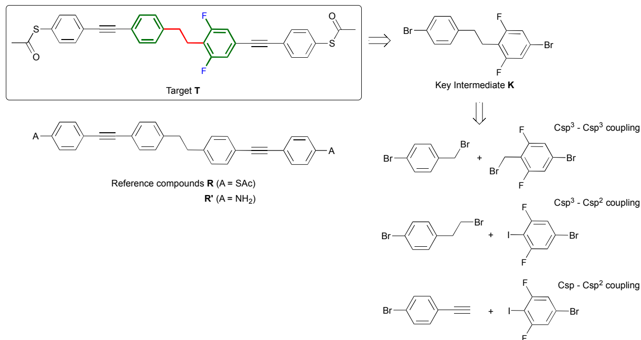
Scheme 1. Structure of target compound T and reference compounds R and R' , and retrosynthetic pathways to T through intermediate K .
