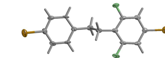
Figure 1. Molecular structure of K in the crystal. Displacement parameters are drawn at the 50% probability level.
