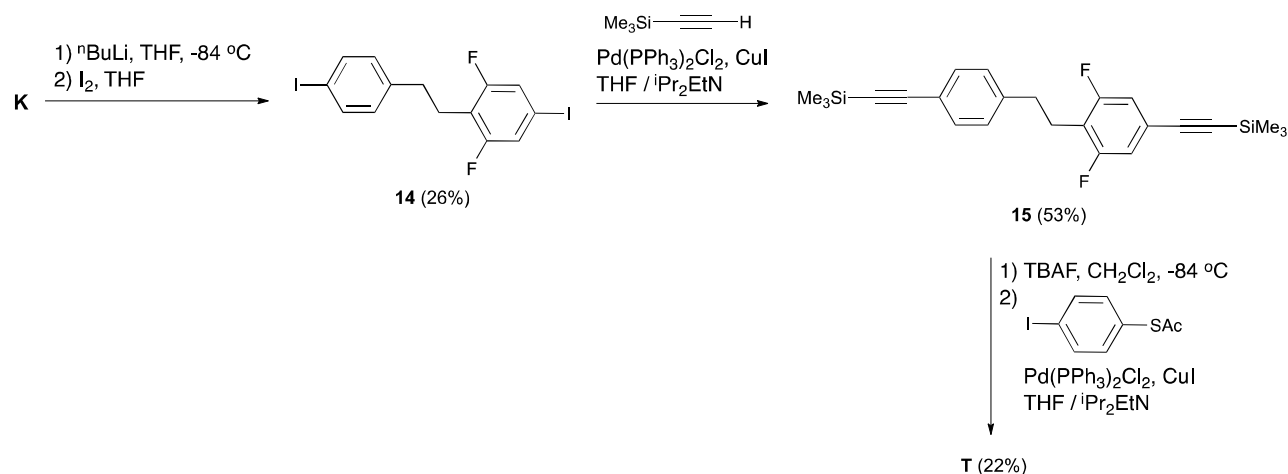
Scheme 5. Synthesis of molecular wire T
