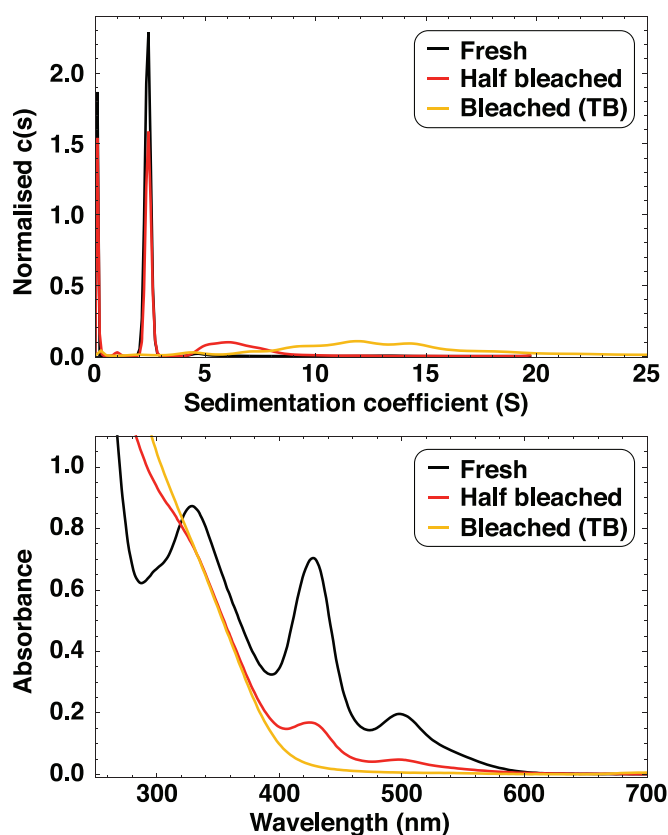
Fig. 4 Top: sedimentation coefficient distributions (60,000 rpm, 395 nm) and bottom: UV-Vis absorption spectra of fresh clusters (black), TB clusters (yellow) and clusters that are not yet fully bleached (red). The small species with sedimentation coefficient close to 0 S is free LA.
