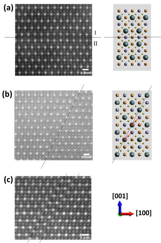
Fig. 3 Atomic resolution HAADF images of antisite domain boundaries (ADB) showing fault displacement of \frac{1}{2}[110] (a), -\frac{1}{4}[201] (b) and -\frac{1}{2}[201] (c).
