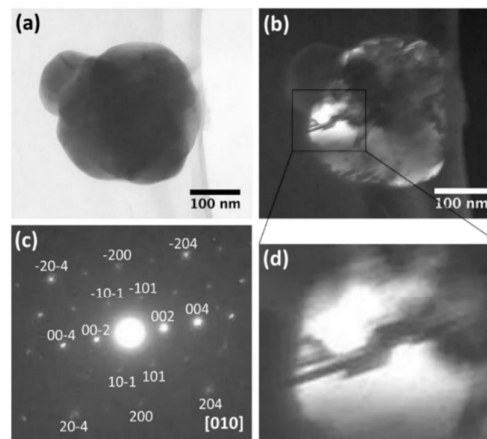
Fig. 5 TEM images of CZTS nanocrystals in bright (a) and dark field (b) taken in the superlattice reflection \mathbf{g} = 002 illustrated by the selected area electron diffraction pattern (c). Expanded dark field image highlighting contrast arising from ADBs (d).
