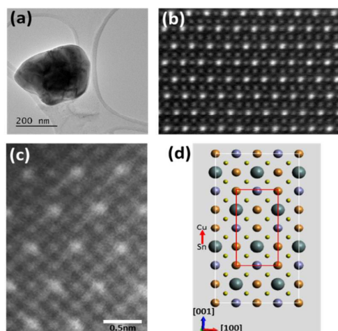
Fig. 2 TEM image of the entire CZTS nanocrystal (a). Atomic resolution high angle annular dark field (HAADF) images (b-c). (d) Schematic representation of an expanded unit cell describing all atomic columns of elements (Cu, Zn, Sn and S) visible in (c).
