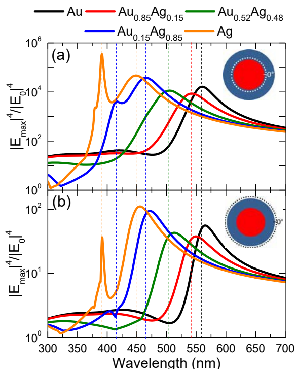
Figure 8. Spectra of the near electric field maximum for Au x Ag 1-x @SiO 2 nanoparticle of 30 nm core radius and 5 nm shell thickness around (a) the core surface, and (b) at the shell surface, for different compositions of Au x Ag 1-x core. The fields are computed at a distance of 0.5 nm from the corresponding surface (see insets).
