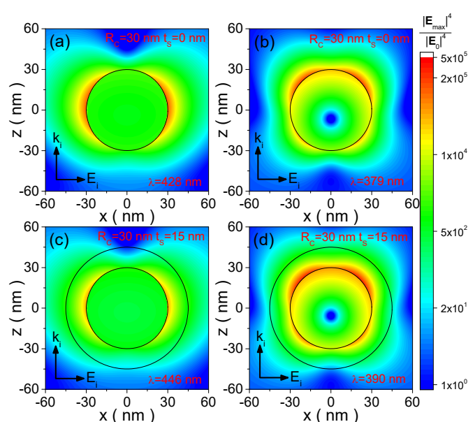
Figure 5. Near electric field distribution maps for (a, b) a bare silver nanoparticle of 30 nm radius, (c, d) an Ag@SiO 2 NP of 30 nm core radius and 15 nm shell
