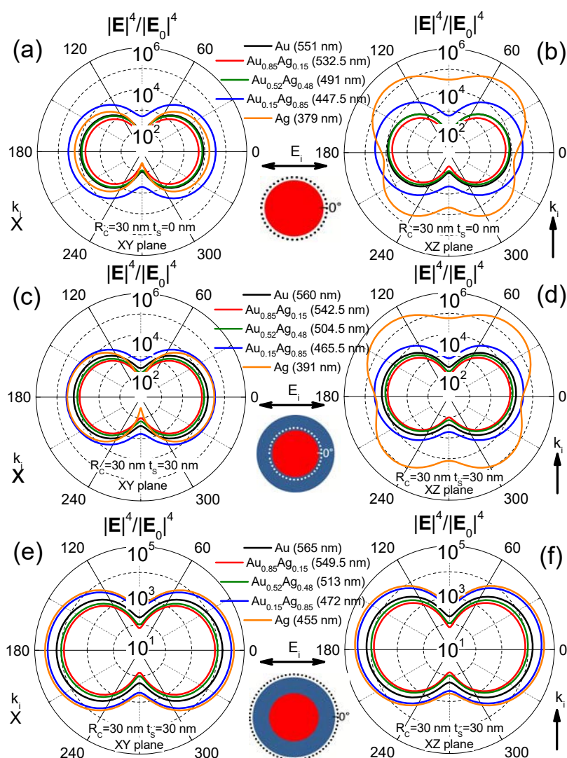
Figure 7. Polar plots of the near electric field distribution (at LSPR wavelength) around (a, b) a bare nanoparticle of 30 nm radius, (c, d) near the core of a core@ \text{SiO}_2 NP of 30 nm core radius and 30 nm shell thickness, and (e, f) near the shell of the same NP as (c, d). The fields are computed at a distance of 0.5 nm from the corresponding surface (dashed circumferences on the schemes between plots indicate where was measured the electric field) Left column is for the XY plane and the right one is for the XZ plane. The analysed compositions of the \text{Au}_x\text{Ag}_{1-x} NPs are indicated in the figure.
