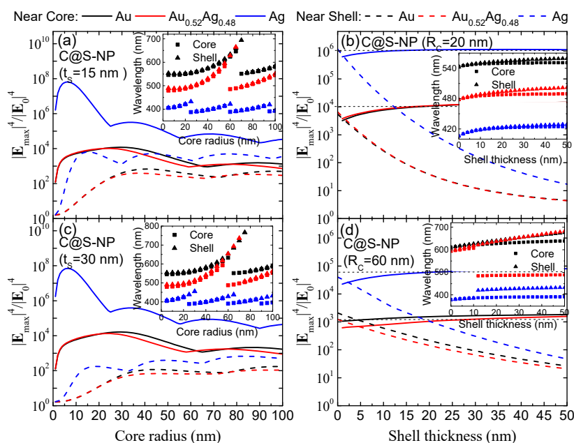
Figure 4. Maximum value of the fourth-power near electric field, computed at a distance of 0.5 nm away from the core surface (solid lines) and from the shell surface (dashed lines) as a function of the core radius for the fixed shell thickness (a) 15 nm and (c) 30 nm, and as a function of shell thickness for the fixed core radius of (b) 20 nm and (d) 60 nm. Core particles of three compositions have been considered for all the plots. The insets are the plots of the wavelengths corresponding to the maximum value of the near electric field around the core (squares) and the shell (triangles) as a function of the nanoparticle radius and shell thickness, respectively.
