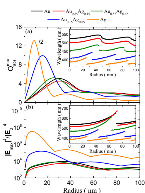
Figure 3. Variation of (a) absorption efficiency and (b) near electric field (computed at a distance of 0.5 nm from the NP surface) with the size of \text{Au}_x\text{Ag}_{1-x} NPs. The composition of the bimetallic NPs are indicated in (a). The insets are the plots of wavelengths corresponding to the maximum value of the absorption efficiency and the near electric field as a function of the nanoparticle radius, respectively.
