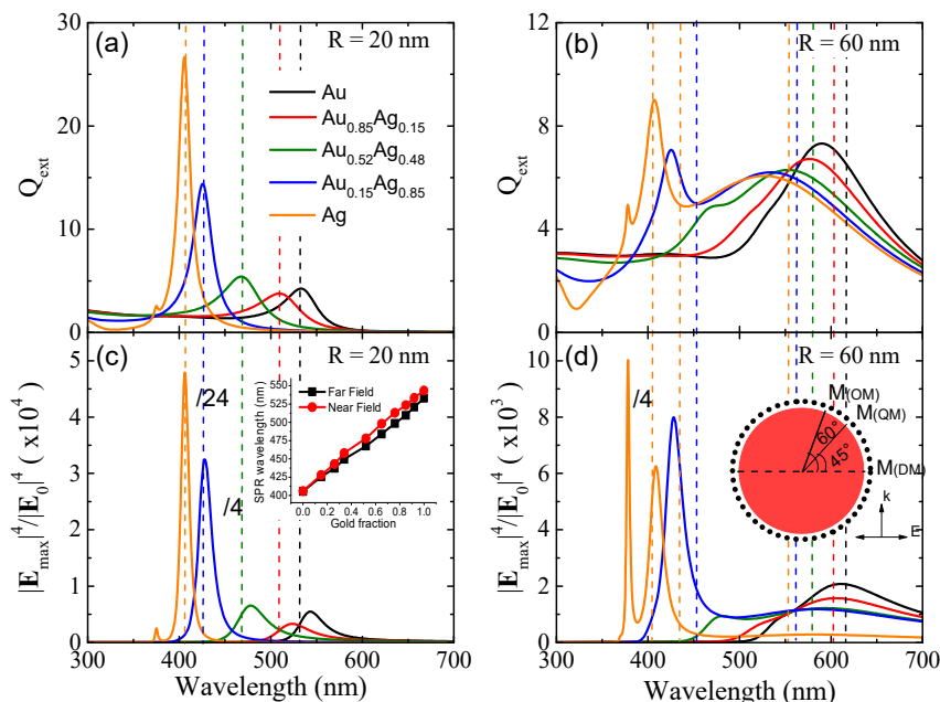
Figure 2. (a, b) Extinction efficiency and (c, d) maximum near electric field enhancement spectra for the bare \text{Au}_x\text{Ag}_{1-x} NPs of radius (a), (c) 20 nm and (b), (d) 60 nm with different compositions. The vertical dashed lines situated at the maximum of each SPR mode in Q_{\text{ext}} and extended to |E_{\text{max}}|^4/|E_0|^4 plots are presented to appreciate the relative change of the SPR modes in the near field. Inset in (c) shows the position of SPR bands for 20 nm \text{Au}_x\text{Ag}_{1-x} NPs. The inset in (c) represents the variation of the LSPR maximum in the far- (black squares) and the near-field (red circles) as a function of the gold fraction.
