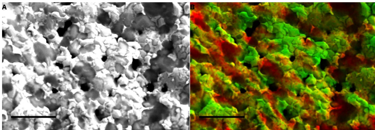
Figure 5: (A) SEM image of the cobalt graphene foam (CoGF) pre-acid wash and (B) Carbon intensity EDX map showing regions of high carbon signal (red) and low carbon signal (green). Scale bars are 10 \mu\text{m} and images taken at 15 kV in SE mode.
