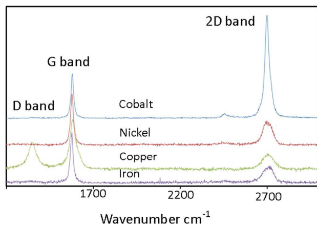
Figure 3: Raman spectra of graphene derived from four different metals. Blue shows the cobalt graphene foam (CoGF), red the nickel graphene foam (NiGF), green the copper graphene foam (CuGF) and purple the iron graphene foam (FeGF). Spectra are normalized with respect to the G band.
