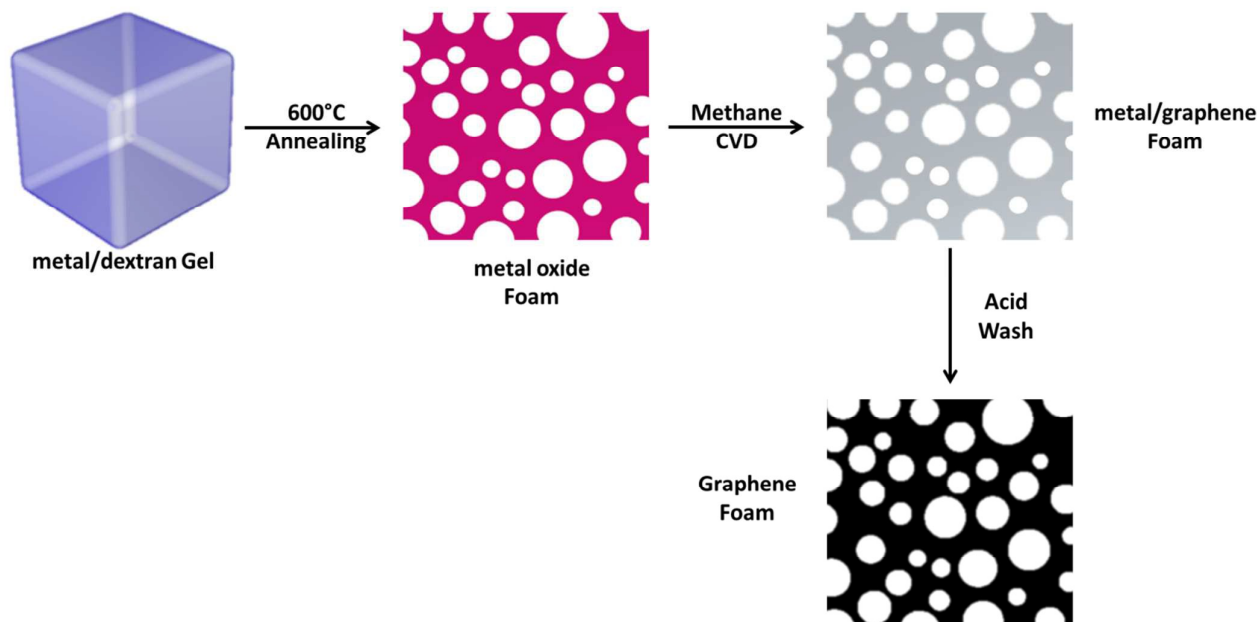
Figure 1. Schematic of the synthesis of metal graphene foams.
