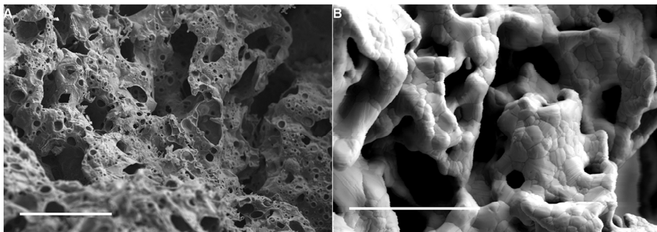
Figure 2: SEM (SE) images (A) showing the cobalt oxide foam, image taken at 10 kV with scale bar 100 \mu\text{m} , and (B) showing the cobalt metal foam obtained from cobalt oxide reduced at 1000 ^{\circ}\text{C} in the presence of hydrogen. Image taken at 8 kV with scale bar 20 \mu\text{m} .
