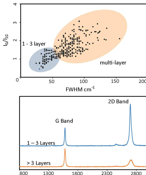
Figure 4: Top: Scatter plot of I_G/I_{2D} ratio vs FWHM for CoGF showing the mixture of 1 – 3 layer graphene (blue region) and multi-layer graphene (orange region). Bottom: Individual Raman spectra of two commonly occurring regions in the cobalt derived graphene (CoGF), 1-3 layers (blue) and > 3 layers (orange). Positions in the scatter plot are marked with blue and orange diamonds respectively.
