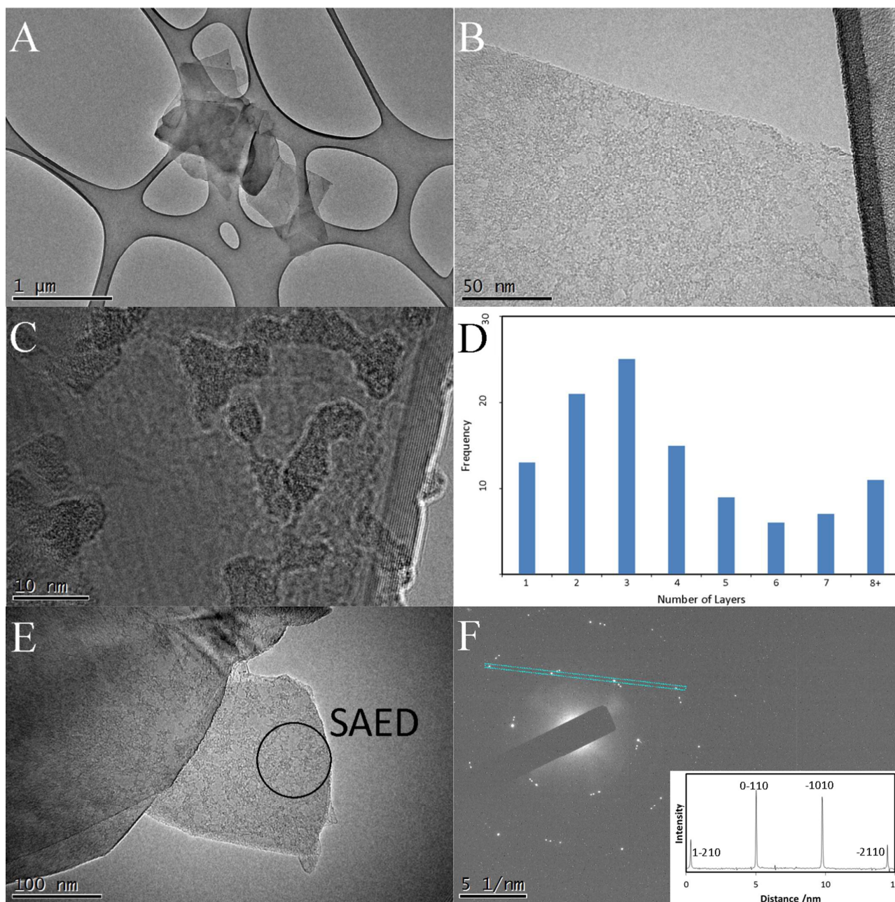
Figure 7: (A) Low magnification TEM image of graphene sheets from the cobalt graphene foam (CoGF). (B) HRTEM image of a single graphene sheet. (C) HRTEM image of a multi-layer graphitic sheet. (D) Histogram of the number of layers observed for the graphene in the TEM across 107 images. (E) TEM image of graphene and the region where the SAED pattern was taken. (F) SAED from region shown in E) and intensity profile inset.
