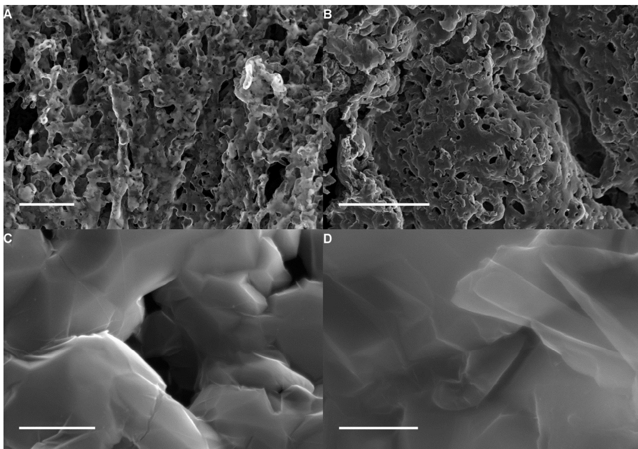
Figure 6: (A) – (D) SEM (SE) images of the cobalt graphene foam (CoGF) after HCl wash. Scale bars are 50 \mu\text{m} , 30 \mu\text{m} , 1 \mu\text{m} and 500 nm respectively and images taken at 15 kV, 5 kV, 5kV and 15 kV respectively.
