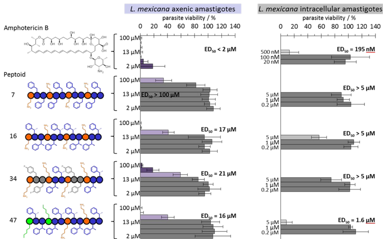
Figure 2. Biological data for intracellular L. mexicana amastigote assay. Briefly, RAW 264.7 murine macrophages were subcultured in 96-well plates and incubated with L. mexicana amastigotes for 24 hours. Infected macrophages were treated with selected peptoids for 24 hours then lysed with SDS solution to release L. mexicana . Following a 48 hour incubation, parasite viability was assessed using the alamarBlue reagent. For cytotoxicity against macrophages only, the protocol was repeated in the absence of parasites.
