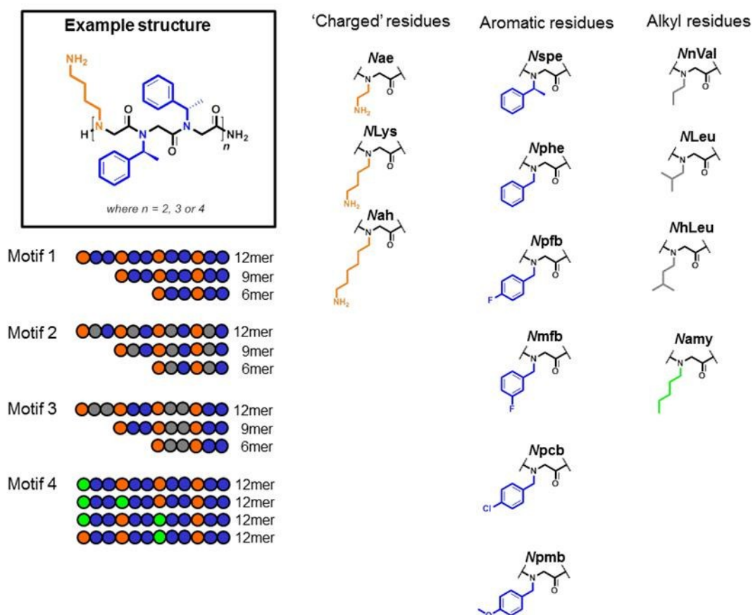
Figure 1. An example of the peptoids synthesised and the chemical structures of subunits used in this peptoid library. The different structural motifs are shown to illustrate the repeating subunits in our sequences.
