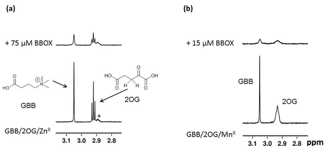
Fig. 2. Monitoring the binding of GBB and 2OG with psBBOX as determined by NMR direct ligand-observation. The GBB (Me 3 singlet at 3.05 ppm) and 2OG (CH 2 triplet at 2.91 ppm) signals from CPMG edited 1 H NMR experiments are shown. (a) GBB and 2OG binding to BBOX-Zn II (b) GBB and 2OG binding to BBOX-Mn II . The assay mixture contains 25 μM GBB, 300 μM 2OG, 150 μM Mn II , 80 mM KCl, in 50 mM Tris-D 11 buffer, pH 7.5, in D 2 O. The asterisk indicates an impurity.
