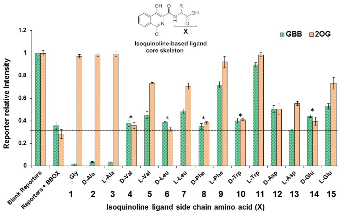
Fig. 4 The chart compares the signal intensity of GBB (green) and 2OG (orange) in the absence of psBBOX (1st left set of column; intensity set to unit intensity) with their intensity after the addition of psBBOX (2nd left set of column) and with their intensity after the addition of isoquinoline-based inhibitors 1-15 (side-chain amino acid X varying). The threshold line represents the relative intensity of the reporters in the presence of psBBOX. After the addition of isoquinoline-ligand, the level above this line represents reporter displacement; the level below represents reporter enhancement of binding. Asterisks highlight isoquinoline-ligands whose addition results in a negligible difference on GBB/2OG under these conditions. The final assay mixture contained 25 \mu\text{M} GBB, 300 \mu\text{M} 2OG, 150 \mu\text{M} \text{Mn}^{\text{II}} , 15 \mu\text{M} BBOX, 80 mM KCl and 25 \mu\text{M} isoquinoline-based ligand in 50 mM Tris- \text{D}_{11} buffer, pH 7.5, in \text{D}_2\text{O} . The error bars represent standard deviations from three separate measurements.
