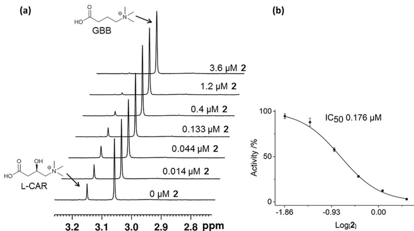
Fig. 5 Measurements of IC_{50} value of the isoquinoline-ligand 2 by ^1H NMR. (a) Bottom to top; psBBOX catalysed GBB turnover into L-carnitine (CAR) in the presence of increasing amounts of 2 . (b) Dose response curve of (a). Error bars represent standard deviations from three separate measurements. The assay mixture contained 200 \mu M GBB, 600 \mu M 2OG, 100 \mu M Fe^{II} , 500 \mu M L-ascorbate, 80 mM KCl and 0.140 \mu M BBOX in 50 mM Tris- D_{11} , pH 7.5 in D_2O .
