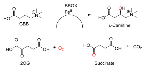
Scheme 1. BBOX catalyses the stereoselective C-3 hydroxylation of GBB to give L-carnitine. The co-substrates are 2OG and oxygen and the co-products are succinate and CO 2 .
