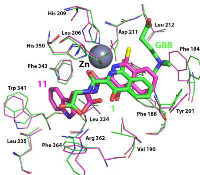
Fig. 6 Docking simulation showing possible conformational changes as a result of binding inhibitors 1 (green sticks, Cl in yellow) and 11 (pink sticks, Cl in yellow) to a model of the psBBOX active site based on a hBBOX X-ray crystal structure (PDB ID: 3O 2G). 20
