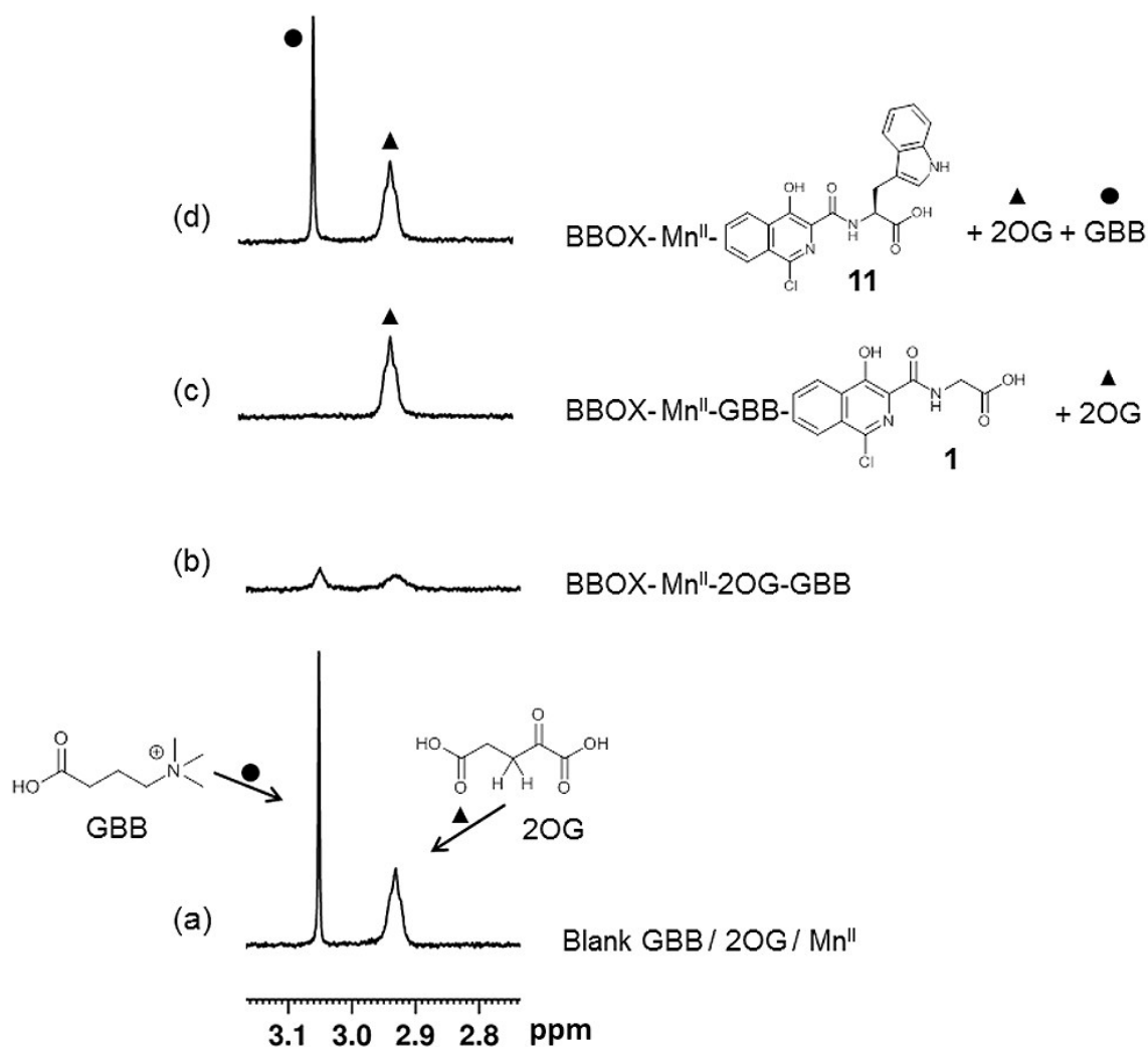
Fig. 3 Studying the binding of isoquinoline ligands 1 and 11 with psBBOX using a NMR dual-reporter displacement assay. 2OG and GBB are used as reporter ligands in CPMG edited ^1H NMR experiments. (a) Reporter ligands GBB and 2OG with Mn^{II} in solution in the absence of psBBOX (b) After the addition of psBBOX (c) Addition of 1 to sample of b (d) Addition of 11 to sample of b. Symbols (●, ▲) indicate reporter signal recovery due to displacement. The final assay mixture contained 25 \mu M GBB, 300 \mu M 2OG, 150 \mu M Mn^{II} , 15 \mu M BBOX, 80 mM KCl and 25 \mu M isoquinoline-based ligand in 50 mM Tris- D_{11} buffer, pH 7.5, in D_2O .
