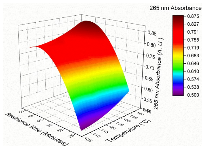
Figure 10. Response contour plot for carvone semicarbazone optimisation
