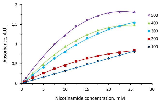
Figure 7. Measured nicotinamide absorbance at varying path lengths
