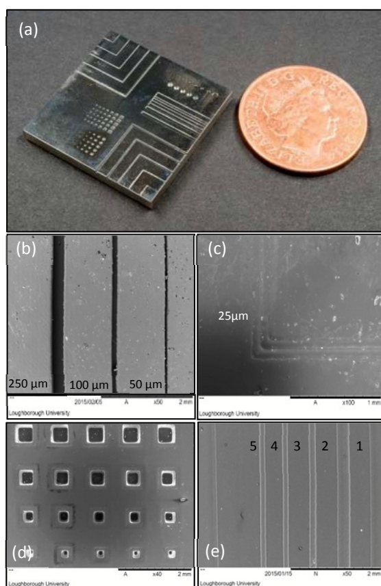
Figure 4. (a) Test piece produced in order to assess the resolution of 3DP-LOC devices and SEM images of (b) Successfully cleared channels from 50 – 250 \mu\text{m} (c) unsuccessfully cleared 25 \mu\text{m} channels (d) Successful manufacture of holes from 200-500 \mu\text{m} (e) SEM micrograph of channel separation (raised channel wall sections appear lighter in colour)
