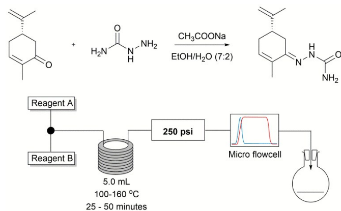
Figure 3. (above) reaction scheme for the formation of carvone semicarbazone (below) schematic for the flow setup
