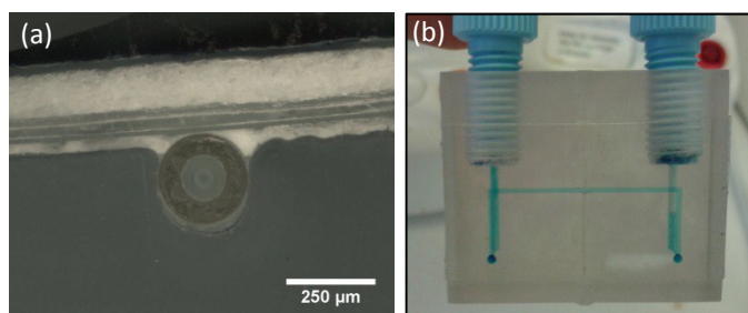
Figure 5. (a) 275 \mu\text{m} u-shaped fibre guides and (b) dye testing of device fitted with fibre to ensure its robustness and ability to cope with high flow rates without leakage
