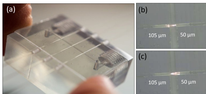
Figure 6. (a) Optimal fibre combination test piece equipped with various combinations of fibres (b) close up images of projection from the 50 \mu\text{m} fibre onto the opposing 105 \mu\text{m} fibre and (c) projection of 105 \mu\text{m} fibre onto opposing 50 \mu\text{m}
