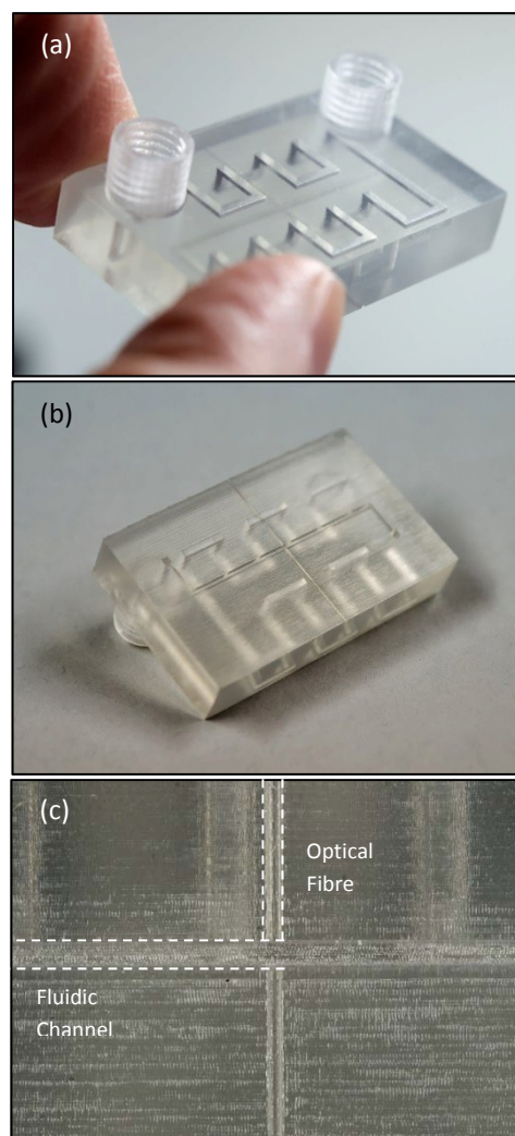
Figure 8. 3D serpentine mixing device used in optimisation (a) Isometric view showing internal channels (b) top face of reactor with high resolution channels (c) close up of monitoring region showing fibers intersecting fluidic channel
