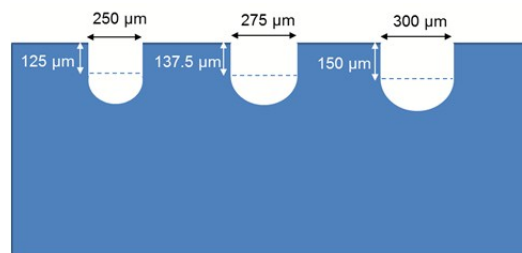
Figure 1. U-shaped fibre channels at the various selected dimensions
