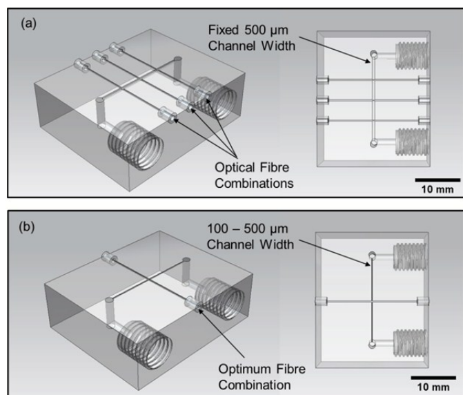
Figure 2. CAD models of (a) optical fibre combination test device and (b) path length test device
