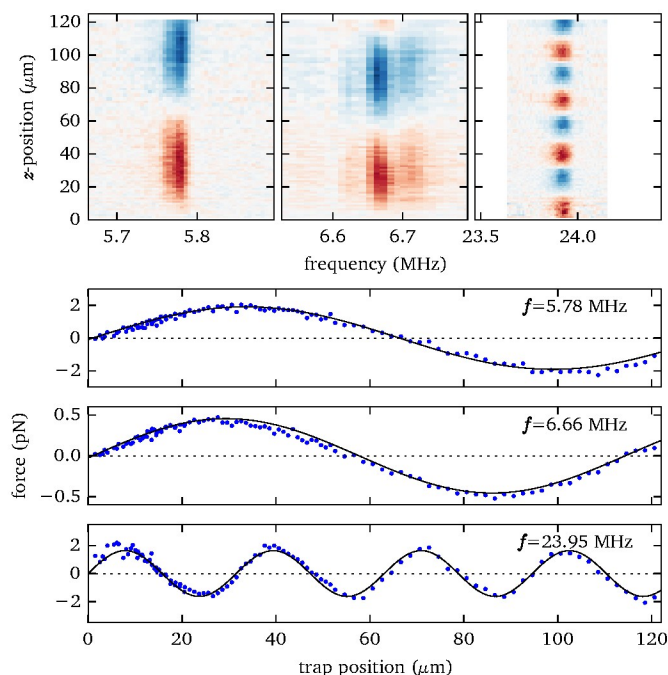
Fig. 9 Measured force profiles for the three most prominent acoustic resonances. The solid black lines in the lower panel are sinusoidal fits to the experimental data (blue points).
