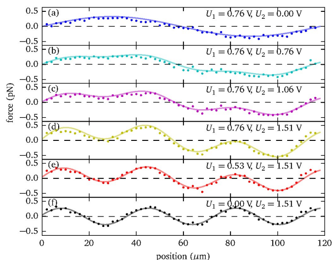
Fig. 11 Force profile engineering by simultaneously exciting two resonances at 6.7 MHz and 21.7 MHz of a 118 \mu\text{m} thick fluid layer. Depending on the relative strength of the individual amplitudes U_1 and U_2 , different force profile shapes can be realized. For the individual modes (top and bottom) the force profiles are well described by a sinusoidal shape (solid lines), determining F_1(z) and F_2(z) of equation (2).
