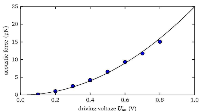
Fig. 4 The measured acoustic force strength acting on a 3.5\ \mu\text{m} diameter silica microsphere scales quadratically with the applied voltage.
