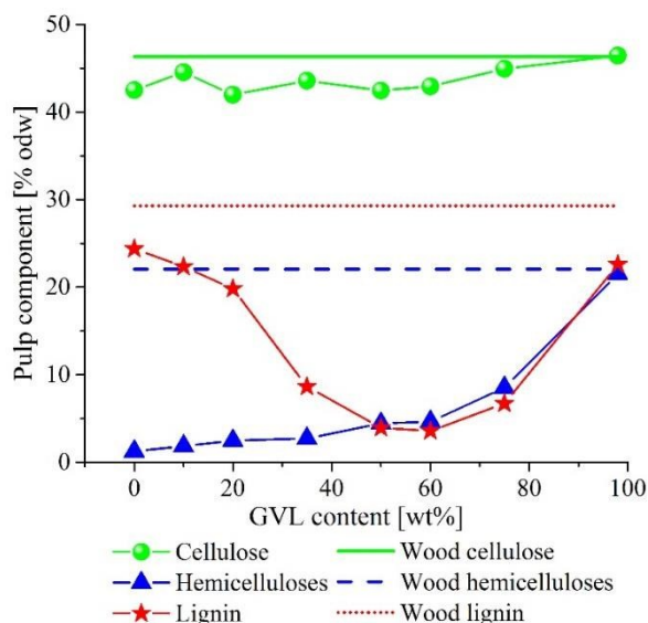
Fig. 1 Effect of GVL content in the fractionation liquor on the removal of wood components from eucalyptus sawdust. Fractionation trials were conducted at 180°C for 120 minutes, with a L:W=10 L/kg. (odw: oven-dried wood).
