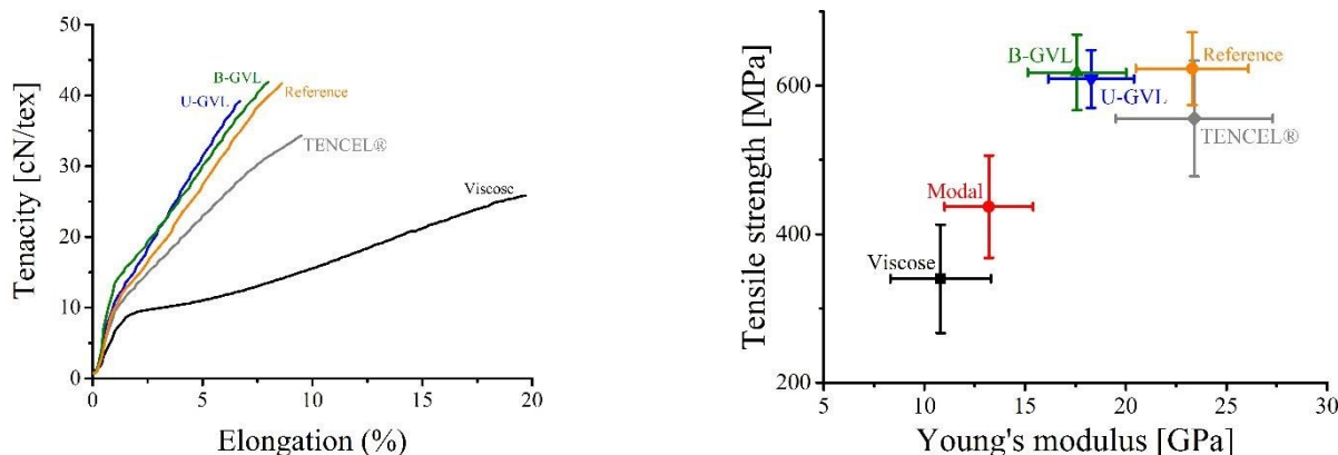
Fig. 4. (LEFT) Stress-strain curves of GVL fibers in comparison to commercial textile fibers. (RIGHT) Young's modulus of different composite and commercial fibers. Values for Viscose, Modal and Lyocell fibers are adopted from Adusumali et al. 2006 48 .
