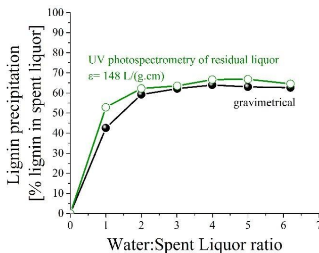
Fig. 5. Relative lignin precipitation from GVL/water fractionation spent liquor by addition of water.
