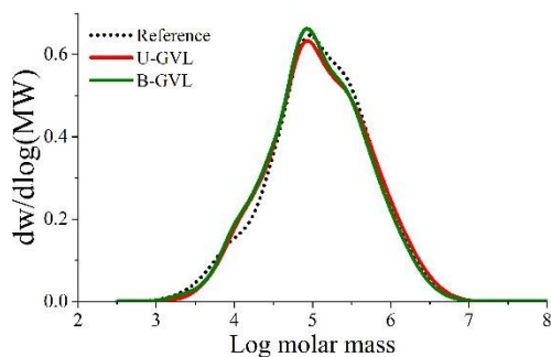
Fig. 2. Molecular mass distribution of unbleached and bleached GVL/water pulps, in comparison with a commercial bleached acid sulfite hardwood dissolving pulp used as reference. (dw/dlog(MW): differential mass fraction).
