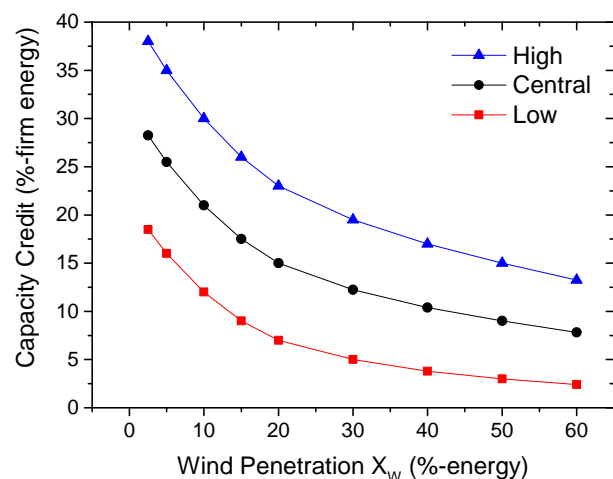
Fig. 8 Capacity credit of wind power generators, based on data presented by Gross et al. 75 and references therein. It can be observed that initial deployment of wind power can contribute between 17 - 37 % of its firm capacity, but that this capacity credit reduces with increasing deployment.
