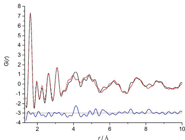
Figure 8: Refinement of the IPC-1P model against PDF data. R_w = 18.0\% . The black solid line is experimental data, the red dashed line is the calculated PDF from the model and the blue line is the difference between the two, offset by -3.
