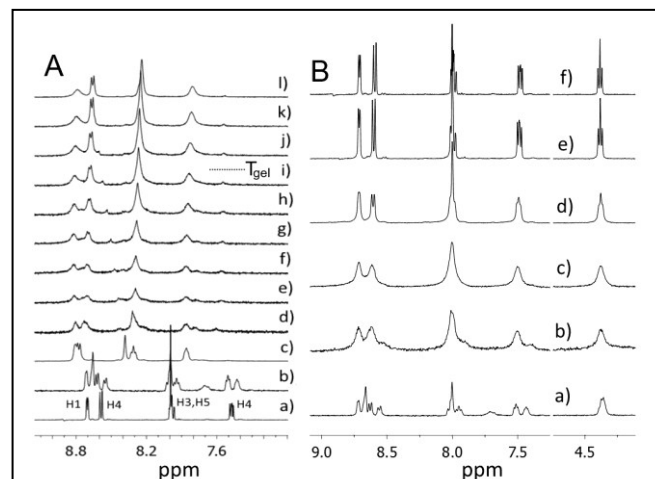
Figure 4. Panel A: 1 H-NMR spectra of a) 1 at 80°C; b) 1 at 25°C and c) after addition of 1 eq. of ZnCl 2 ; d-l) temperature dependent spectra of 1-ZnCl 2 gel system (from 35 °C to 75°C, 5°C step increase). Panel B: Temperature dependent 1 H-NMR spectra of ligand 1 (conc. = 1.4 × 10 -2 M) in DMSO-d 6 from 25° C (a) to 75°C (f) (10 °C step increase).
