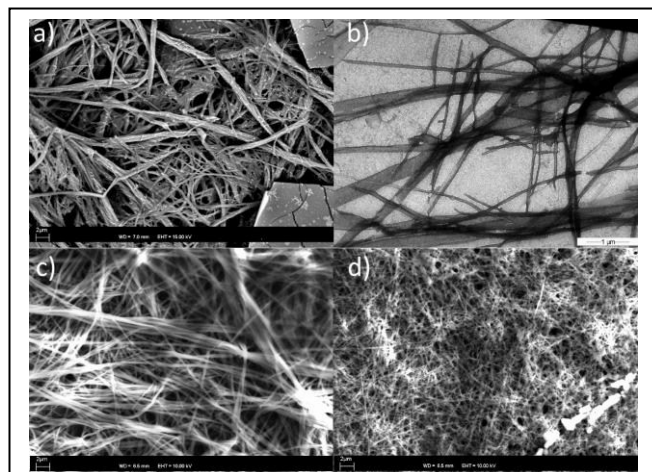
Figure 3. SEM and TEM images of metallogels with ligand 1 : a) SEM image of 1-ZnCl 2 in 9:1 DMSO:water mixture; b) TEM image of 1-ZnCl 2 in 9:1 DMSO:water mixture; c) SEM image of 1-CoCl 2 in 8:2 DMSO:water mixture; d) SEM image of 1-NiCl 2 in 7:3 DMSO:water mixture
