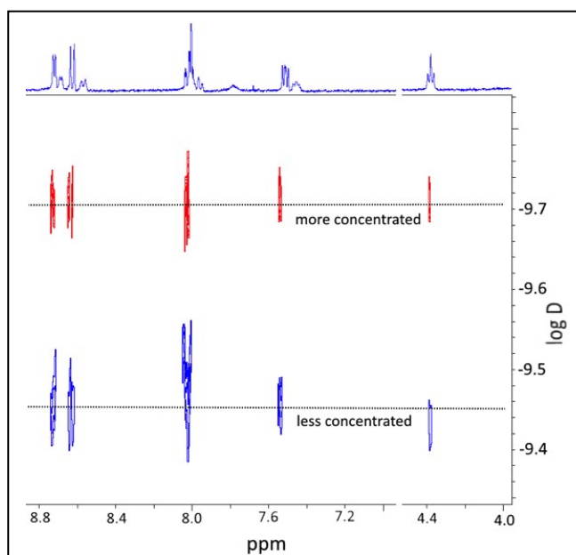
Figure 7. 1 H-DOSY plot of 1 at 4.7 \times 10^{-3} M and 1.4 \times 10^{-2} M concentration. Top projection shows the more concentrated sample (pulse sequence: ledbpgp2s; T = 302 K, ns = 16; TD(f1)=16). Processed with TopSpin software.
