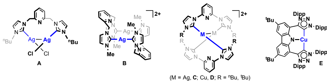
Scheme 2: Examples of isolated Ag(I) and Cu(I) complexes of CNC pincer ligands 12,13,14,15,16,17
