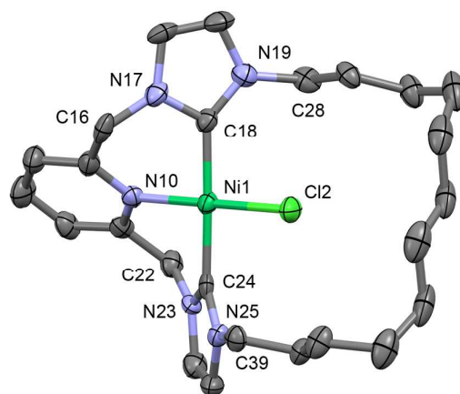
Figure 4. Solid-state structure of 7 . Thermal ellipsoids drawn at the 50% probability level; hydrogen atoms and anion omitted for clarity. Selected bond lengths (Å) and angles (deg): Ni1-Cl2, 2.145(2); Ni1-N10, 1.928(5); Ni1-C18, 1.898(6); Ni1-C24, 1.916(6); N10-Ni1-Cl2, 179.06(15); C18-Ni1-C24, 176.6(3).
