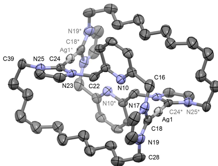
Figure 1. Solid-state structure of 2 . Thermal ellipsoids drawn at the 50% probability level; hydrogen atoms, minor disordered components and anions omitted for clarity. The starred atoms are generated by the symmetry operation 2-x,1-y,1-z. Selected bond lengths (Å) and angles (deg): Ag1–C18, 2.077(3); Ag1–C24*, 2.080(3); Ag1⋯Ag1*, 7.2732(6); C24–Ag1–C18*, 178.99(13); N25–C24–C18*–N19*, 100.2(4).
