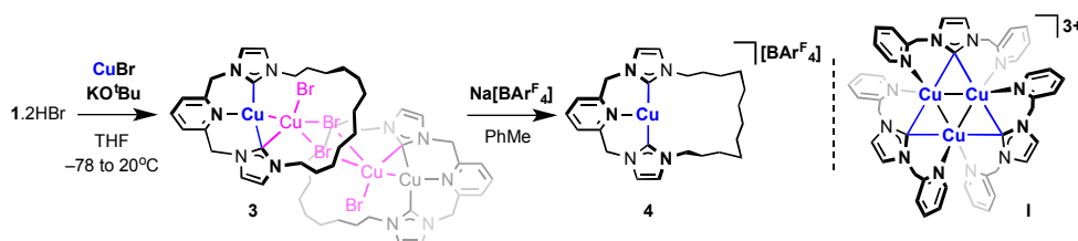
Scheme 4: Preparation of 3 , 4 and a related literature precedent 25
