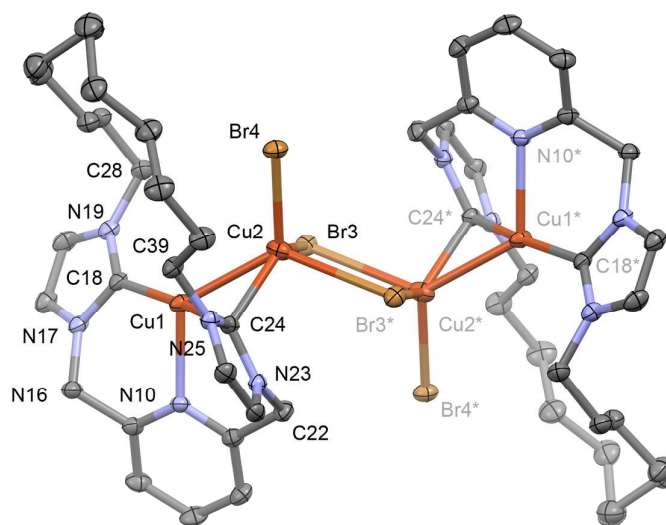
Figure 3. Solid-state structure of 3 . Thermal ellipsoids drawn at the 50% probability level; hydrogen atoms omitted for clarity. The starred atoms are generated by the symmetry operation 1-x, 1-y, 1-z . Selected bond lengths (Å) and angles (deg): Cu1-Cu2, 2.5209(5); Cu1-N10, 2.246(2); Cu1-C18, 1.925(3); Cu1-C24, 1.980(3); Cu2-Br3, 2.4583(4); Cu2-Br3*, 2.7728(5); Cu2-Br4, 2.4149(4); Cu2-C24, 2.070(3); Cu2-Br3-Cu2*, 83.794(15); Br3-Cu2-Br3*, 96.206(15); Cu1-Cu2-C24, 49.92(7); C18-Cu1-C24, 167.92(11).
