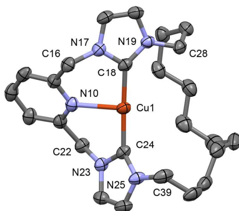
Figure 2. Solid-state structure of 4 . Thermal ellipsoids drawn at the 50% probability level; only one of the unique cations shown ( Z' = 2 ) and hydrogen atoms omitted for clarity. Selected bond lengths (Å) and angles (deg): Cu1-N10, 2.233(3); Cu1-C18, 1.905(3); Cu1-C24, 1.906(3); C18-Cu1-C24, 176.37(13).
