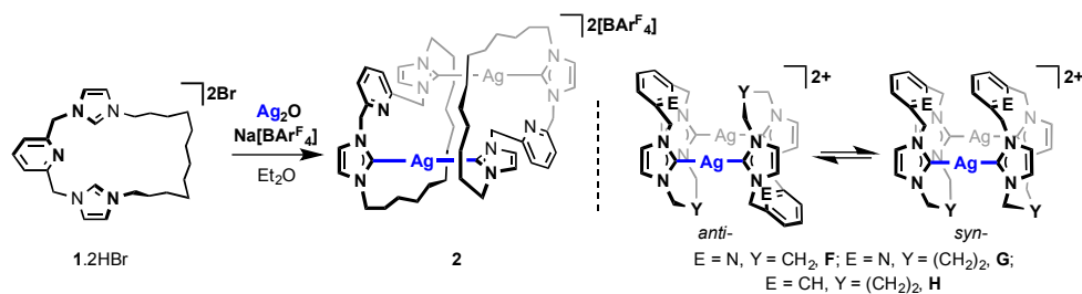
Scheme 3: Preparation of 2 and related literature precedents 11
