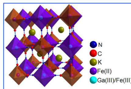
Figure 2. Polyhedral representation of the \text{KGa}_x\text{Fe}_{1-x}[\text{Fe}(\text{CN})_6] ( x=0.02, 0.05, 0.07 and 0.10 ) structure.
